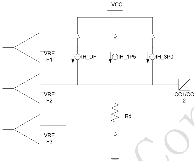
图 9. Plug and Orientation Detection Block
