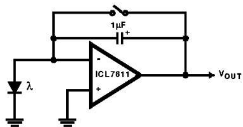
FIGURE 3. PHOTOCURRENT INTEGRATOR
