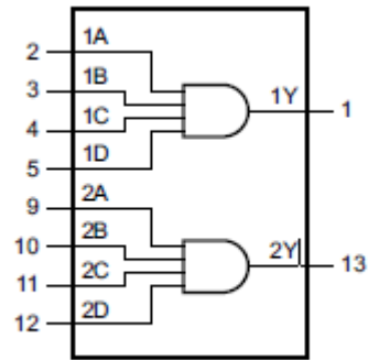
Figure 1. Functional diagram
