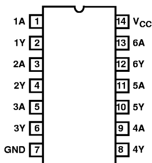
CD54HC14, CD54HCT14, CD74HC14, CD74HCT14 (PDIP, CERDIP, SOIC)
