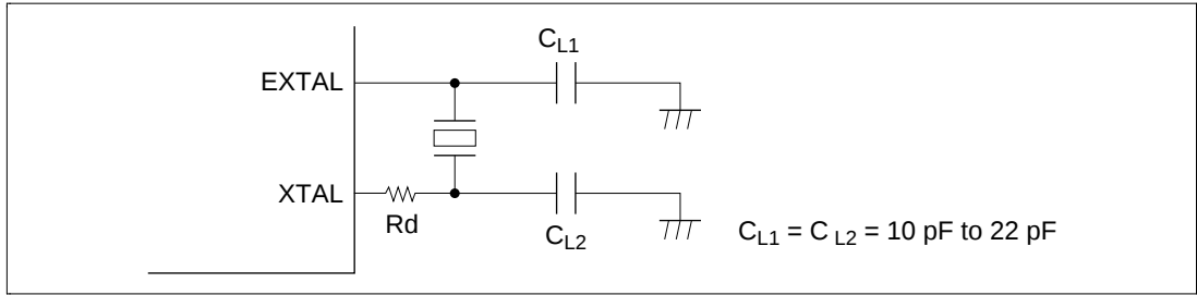
Figure 6.8 Connection of Crystal Oscillator (Example)
