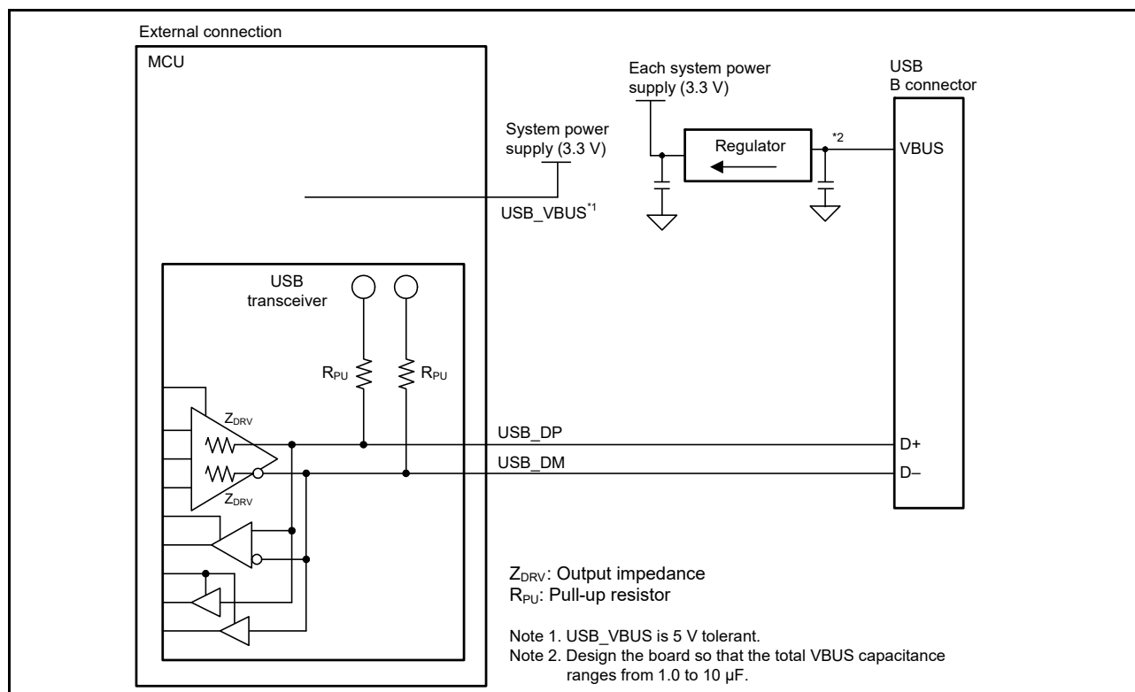
Figure 28.8 Example device connection in bus-powered state
