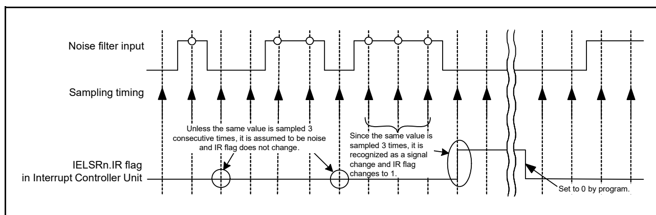
Figure 44.6 Noise filter and interrupt operation example
