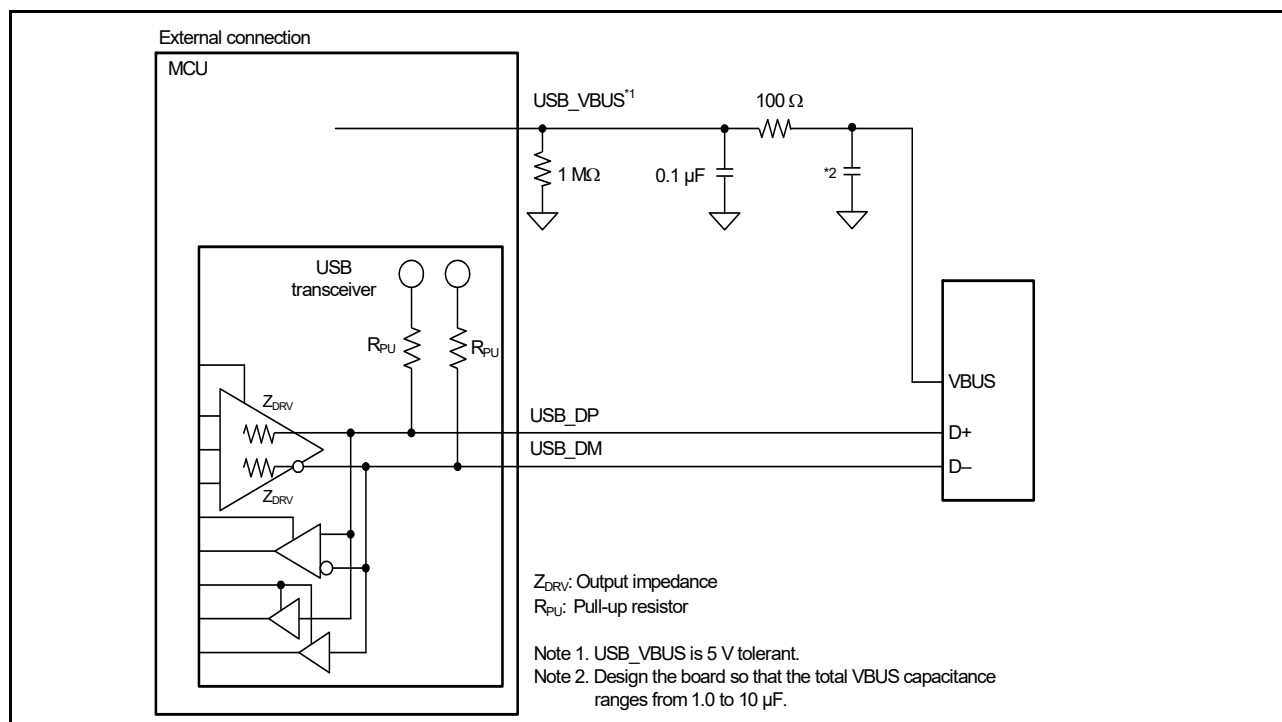
Figure 28.6 Example device connection in self-powered state
