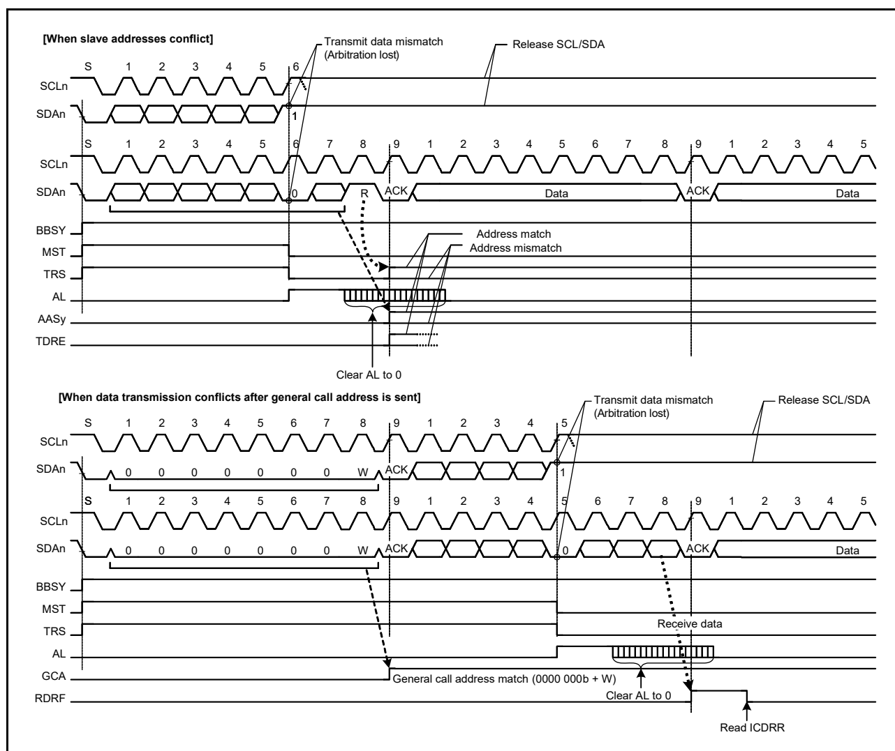
Figure 31.41 Examples of master arbitration-lost detection (MALE = 1)
