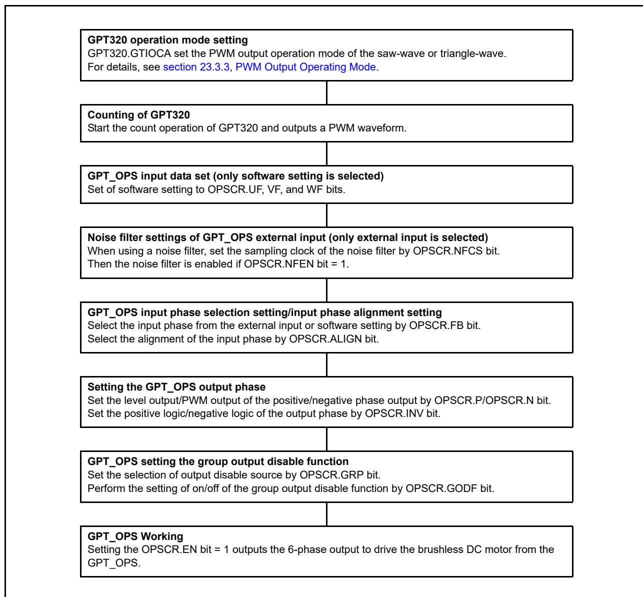
Figure 23.81 Example for setting of GPT_OPS start operation
