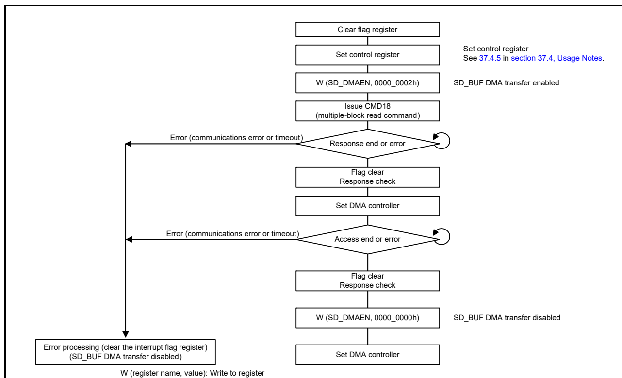
Figure 37.22 Example of SD_BUF_DMA read operation
