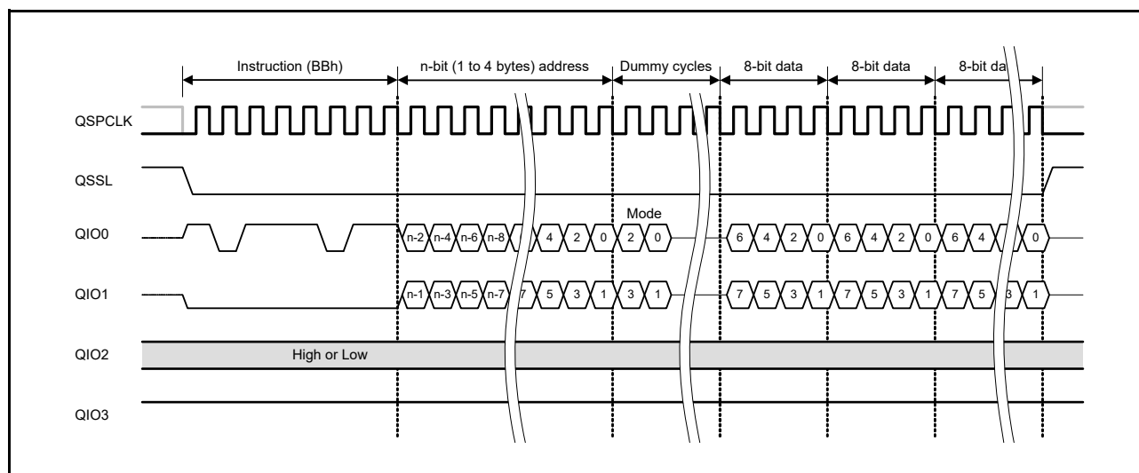
Figure 34.21 Fast read dual I/O bus cycle
