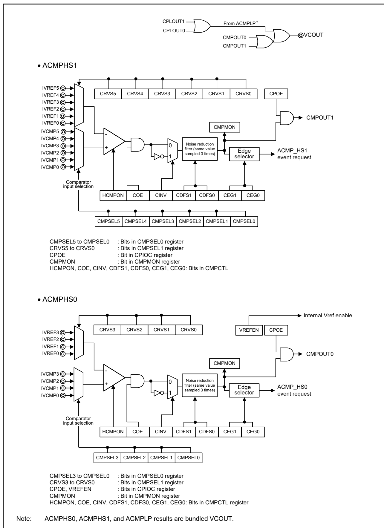
Figure 43.1 ACMPHS block diagram
