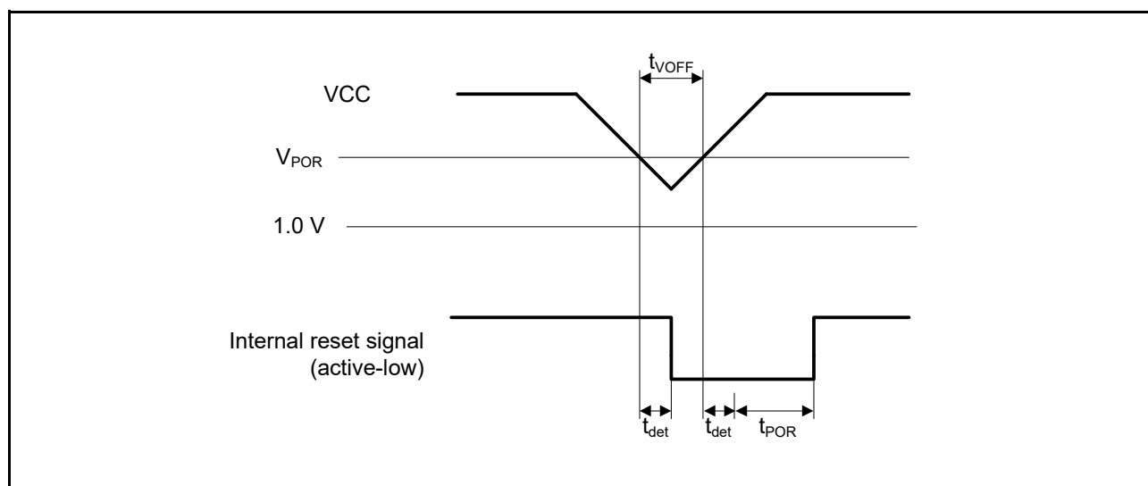
Figure 52.82 Voltage detection reset timing
