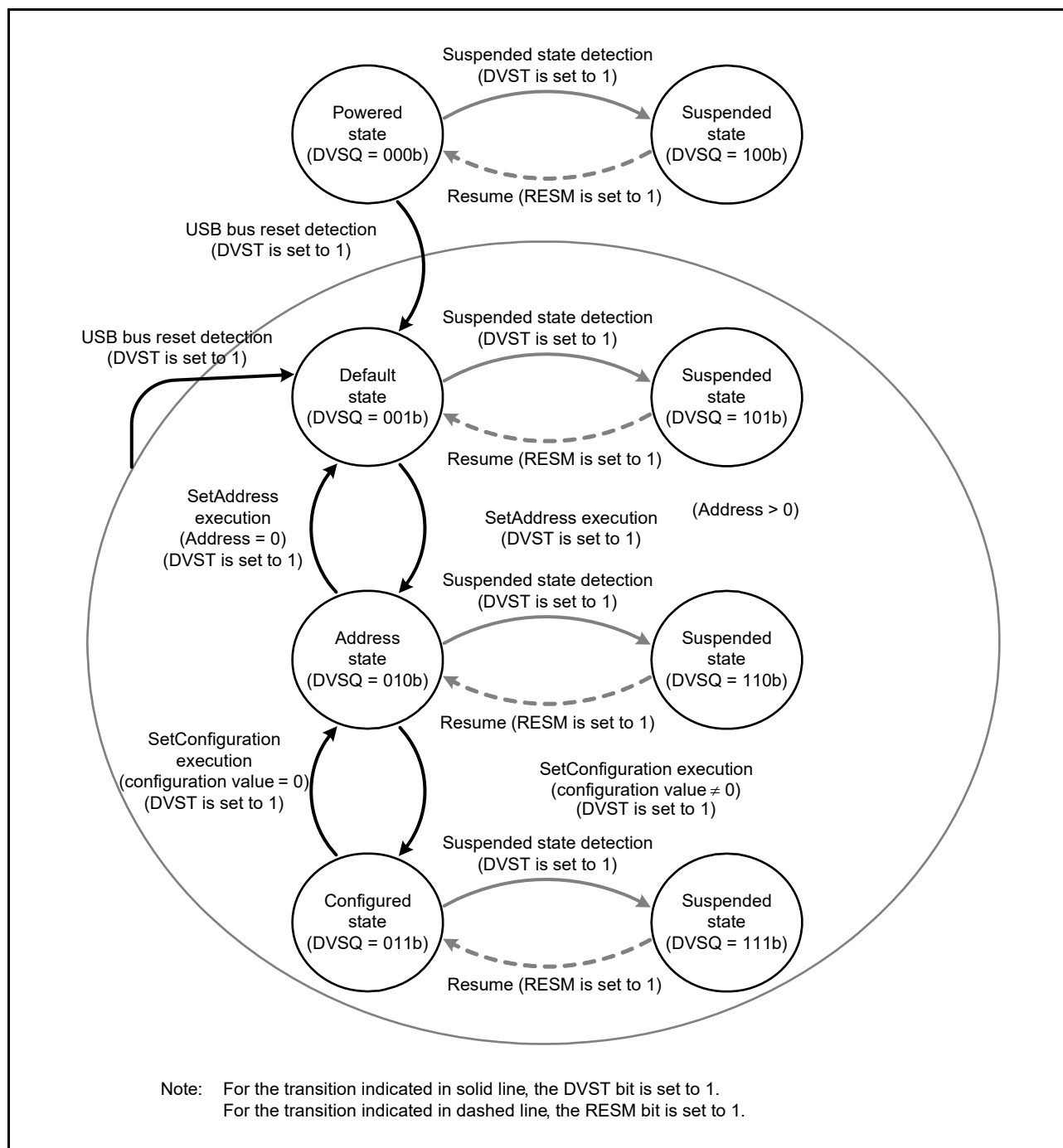
Figure 28.15 Device state transitions
