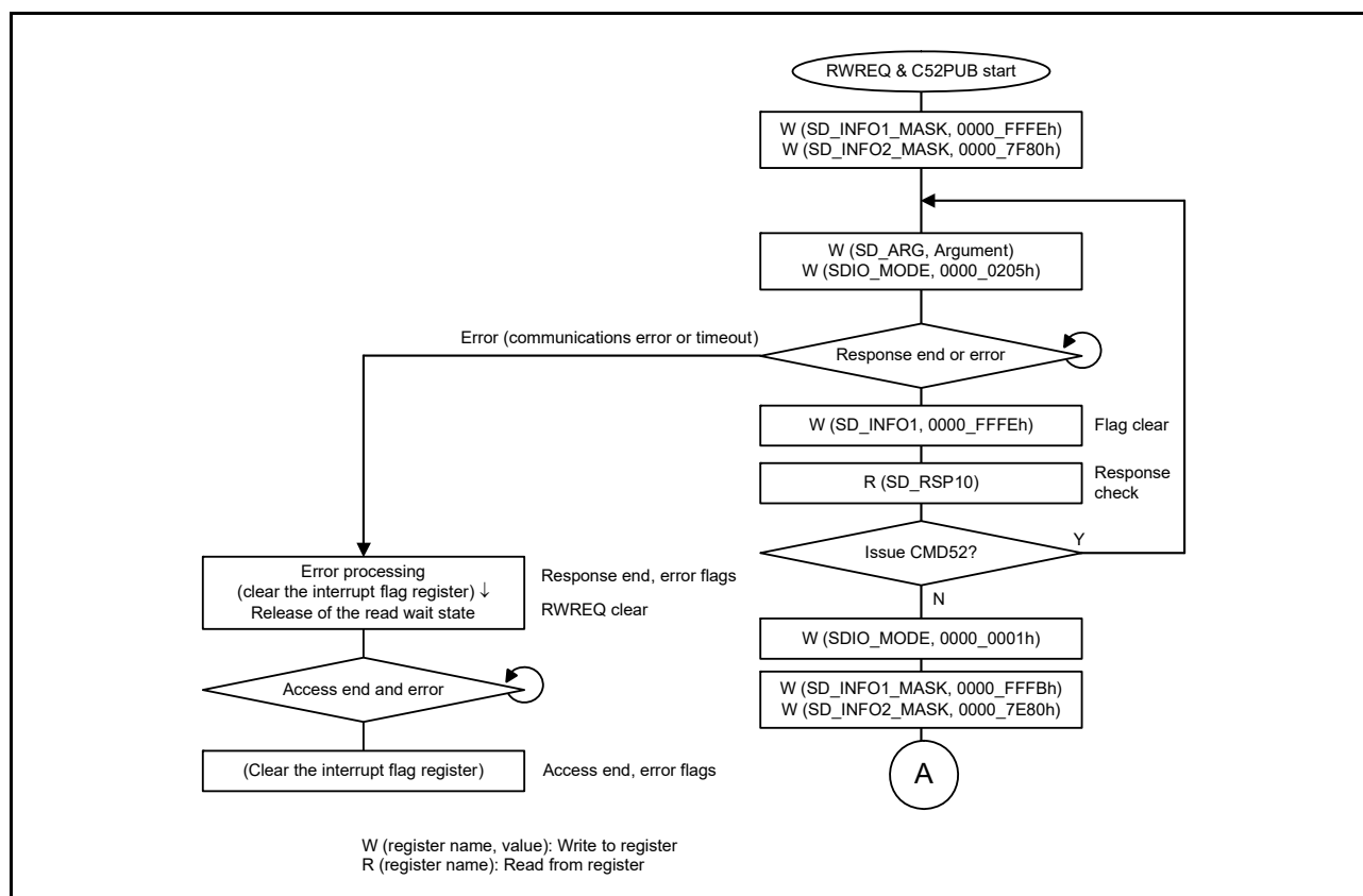
Figure 37.18 CMD52 (SDIO None Abort) is issued at CMD53 multiple block read while SD Host Interface is in read wait state
