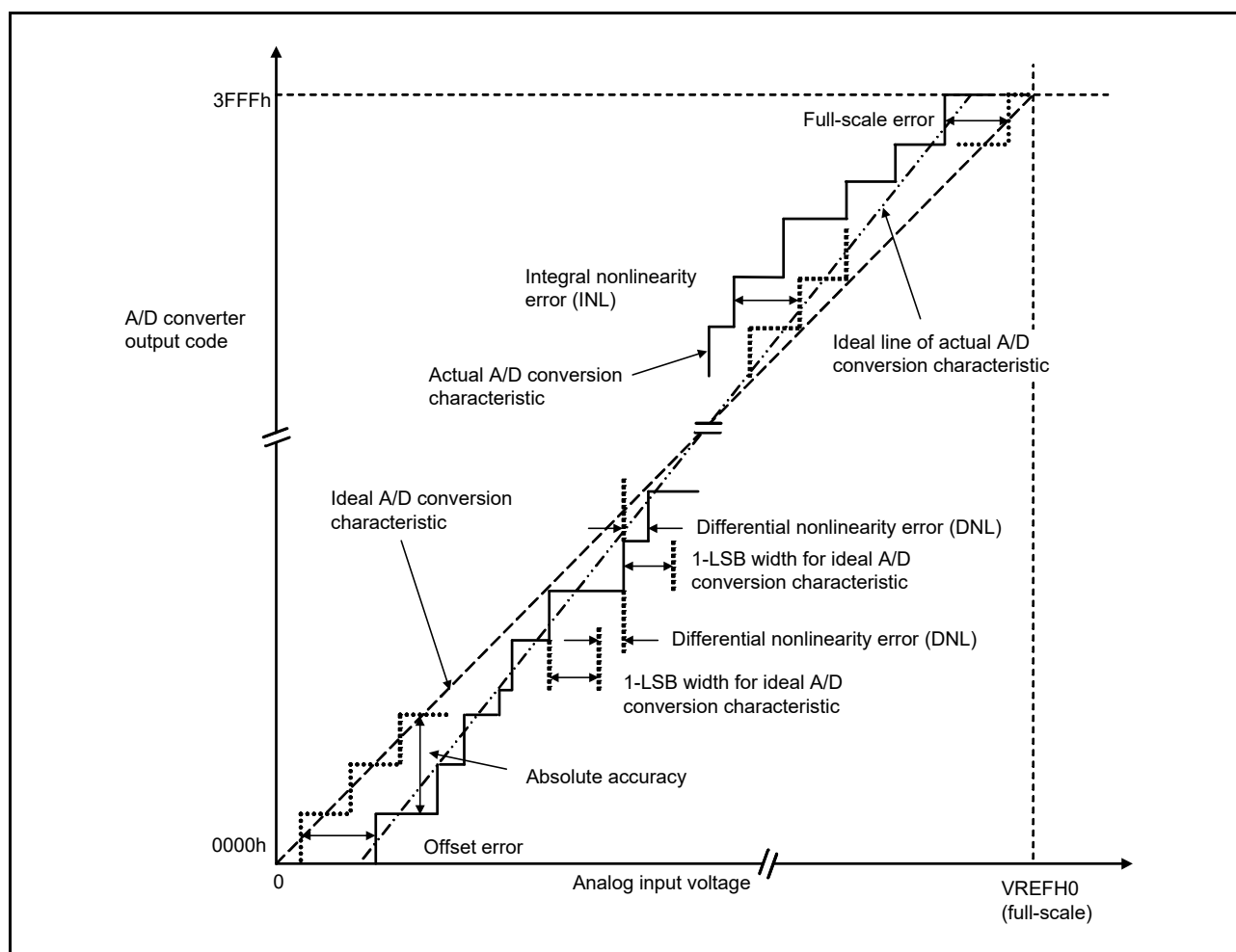
Figure 52.79 Illustration of 14-bit A/D converter characteristic terms
