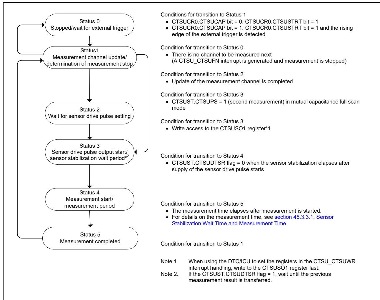
Figure 45.11 Status operation transitions
