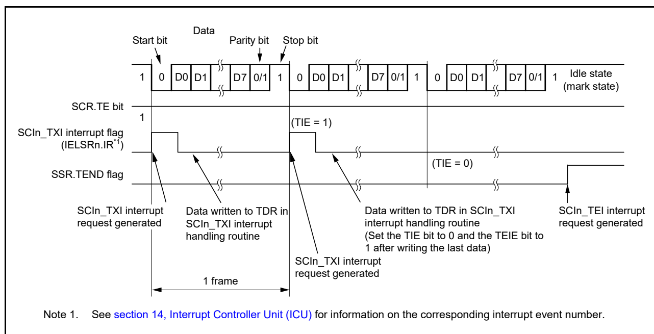
Figure 29.11 Example operation for serial transmission in asynchronous mode (3) with 8-bit data, parity bit, 1 stop bit, CTS function not used, and from the middle of transmission until transmission completion
