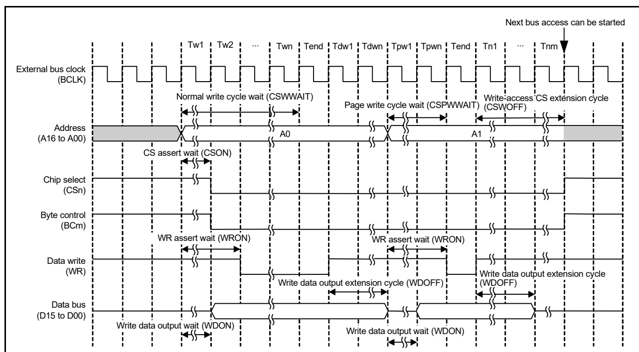
Figure 15.18 Page write access timing ( n = 0 to 3 , m = 0, 1 )
