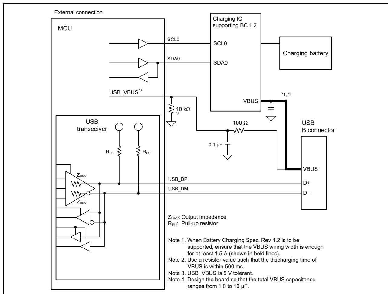
Figure 28.10 Example of functional connection with Battery Charging Rev 1.2 supported
