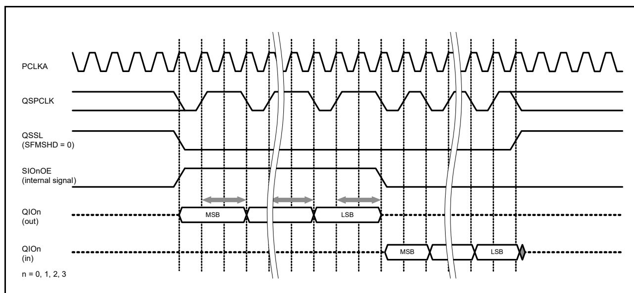
Figure 34.14 Setup time adjustment of serial data output with SFMOHW bit
