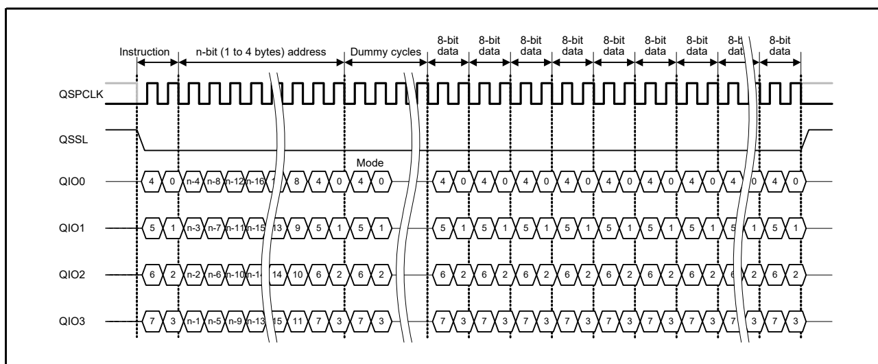
Figure 34.7 Quad SPI protocol example for Fast Read
