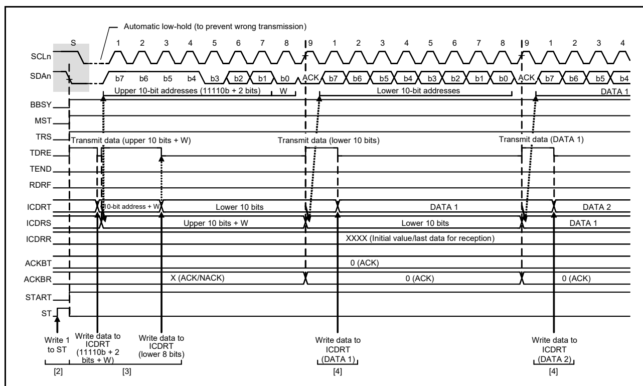
Figure 31.8 Master transmit operation timing (2) (10-bit address format)
