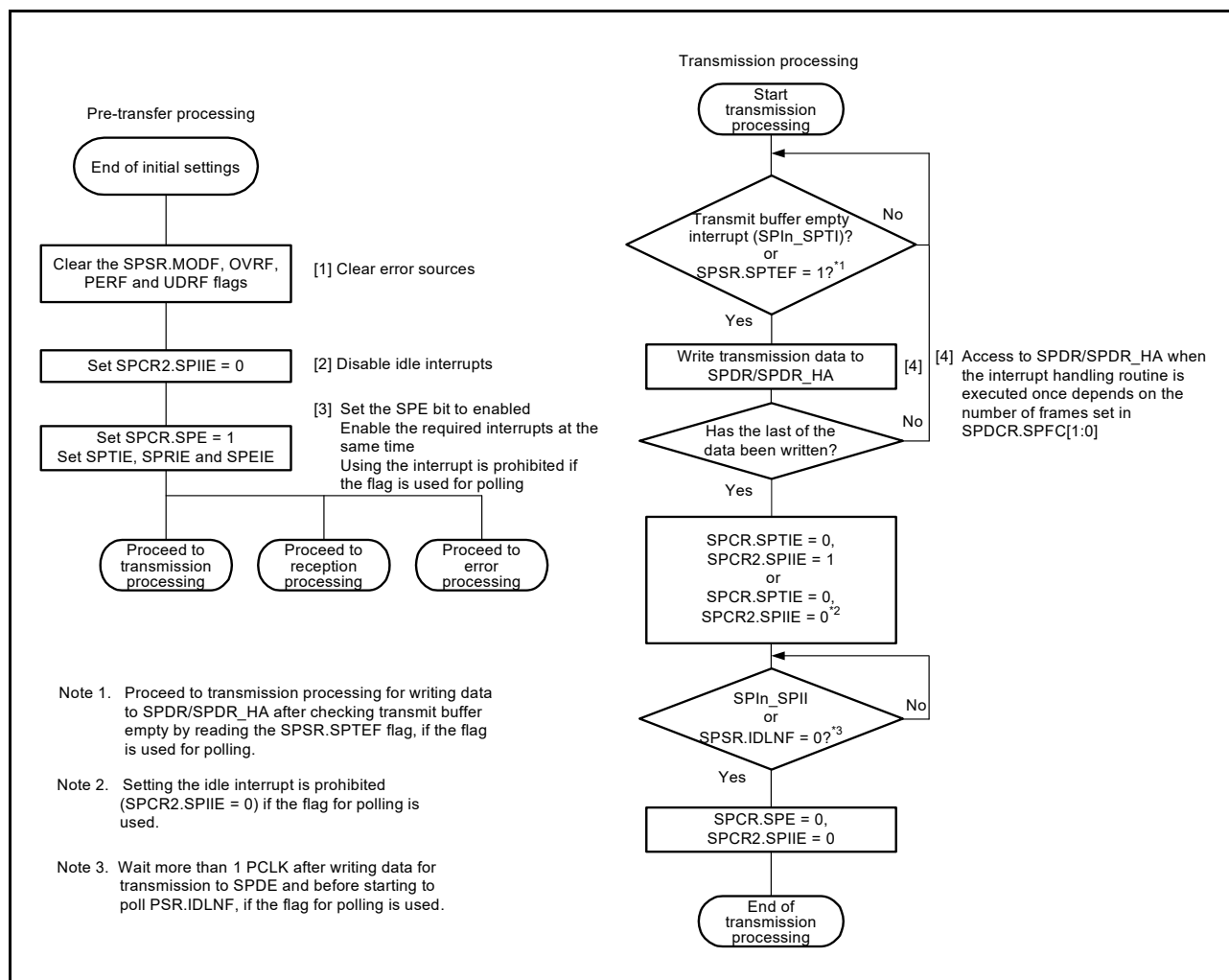
Figure 33.37 Transmission flow in master mode transmission
