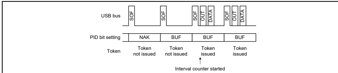
Figure 28.17 Token issuance when IITV = 0
