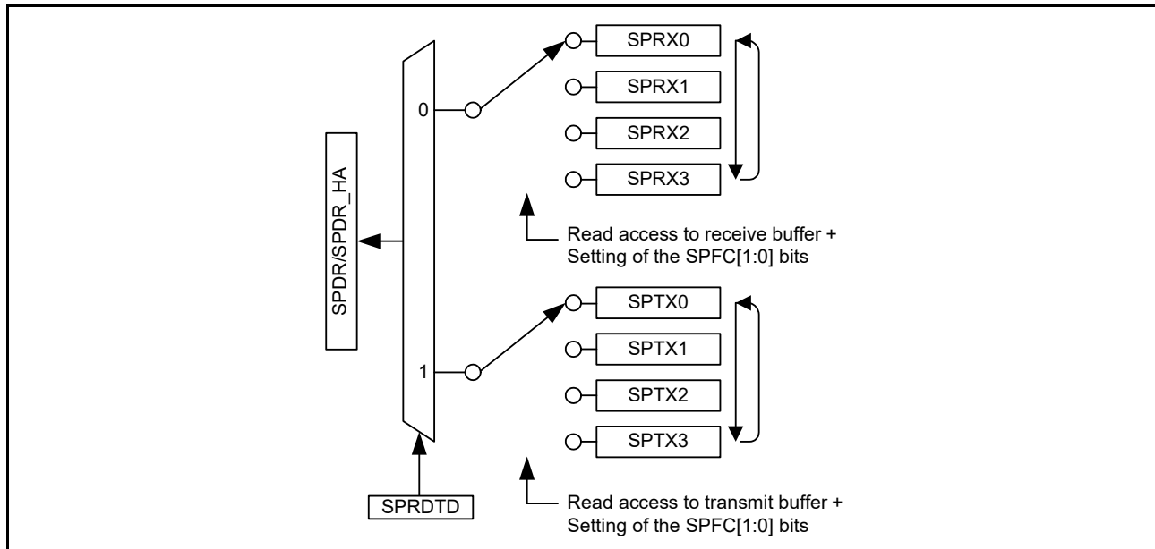
Figure 33.4 Configuration of SPDR/SPDR_HA for read access
