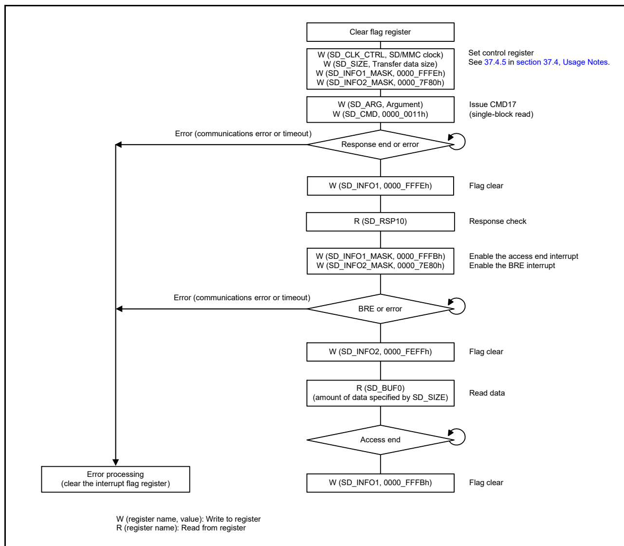
Figure 37.10 Example flow of single block read operation
