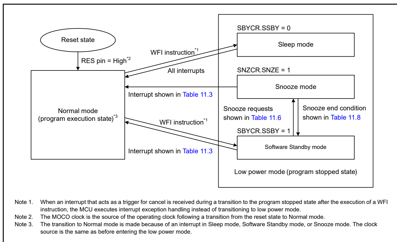
Figure 11.1 Mode transitions
