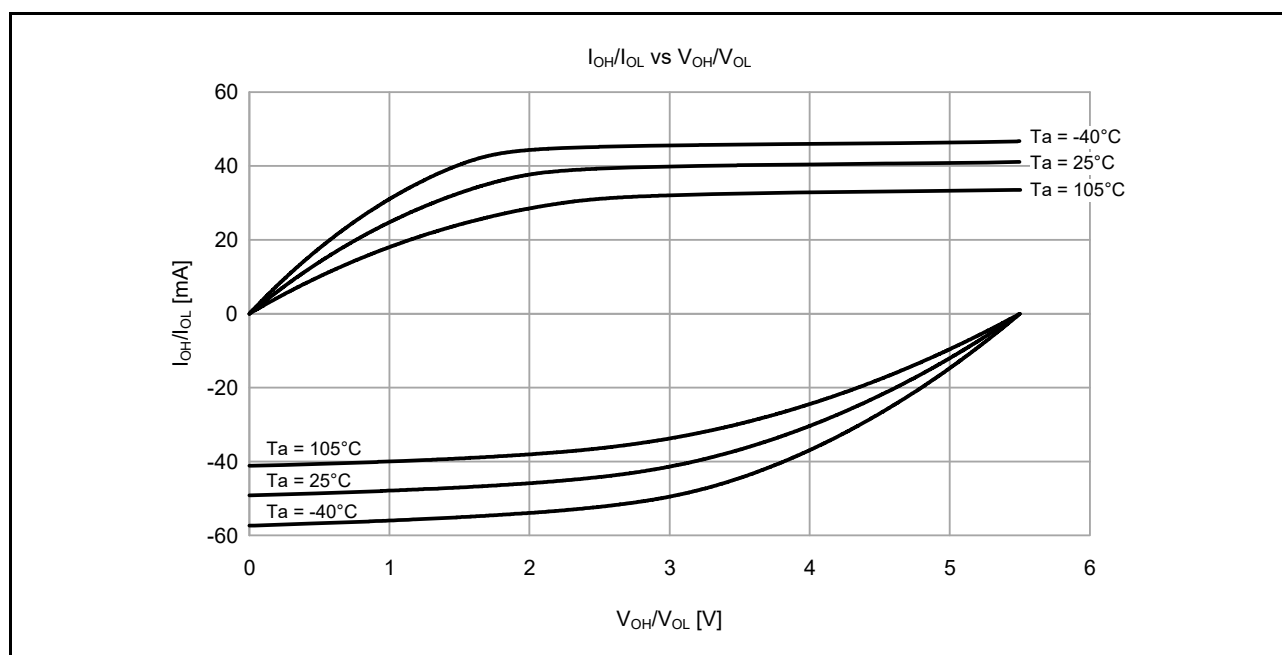
Figure 52.6 V_{OH}/V_{OL} and I_{OH}/I_{OL} temperature characteristics at V_{CC} = 5.5 V when low drive output is selected (reference data)
