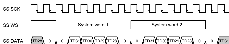
Figure 36.8 Inverted clock
