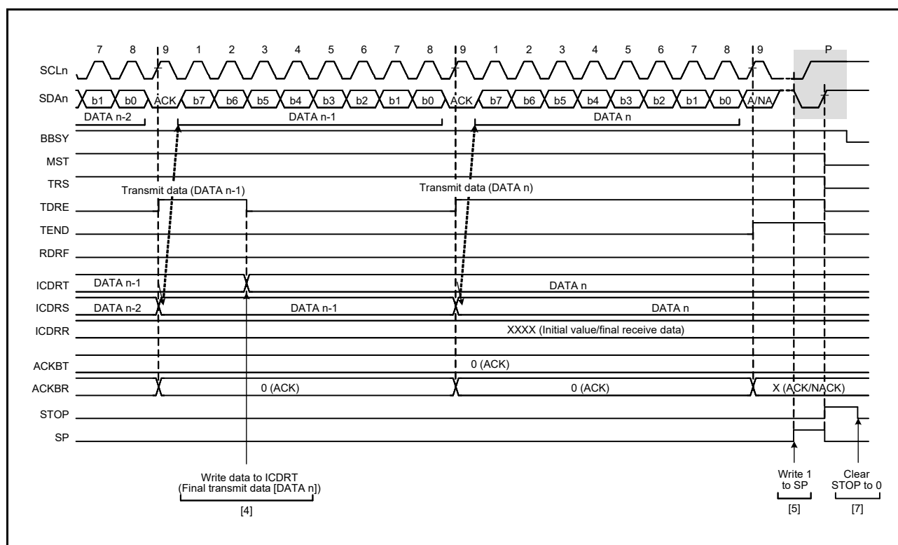
Figure 31.9 Master transmit operation timing (3)
