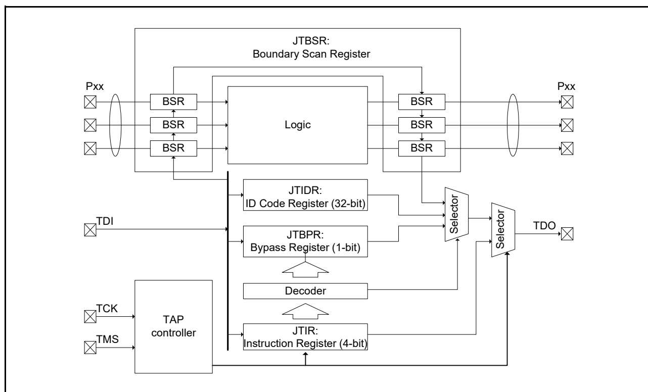
Figure 38.1 Boundary scan function block diagram
