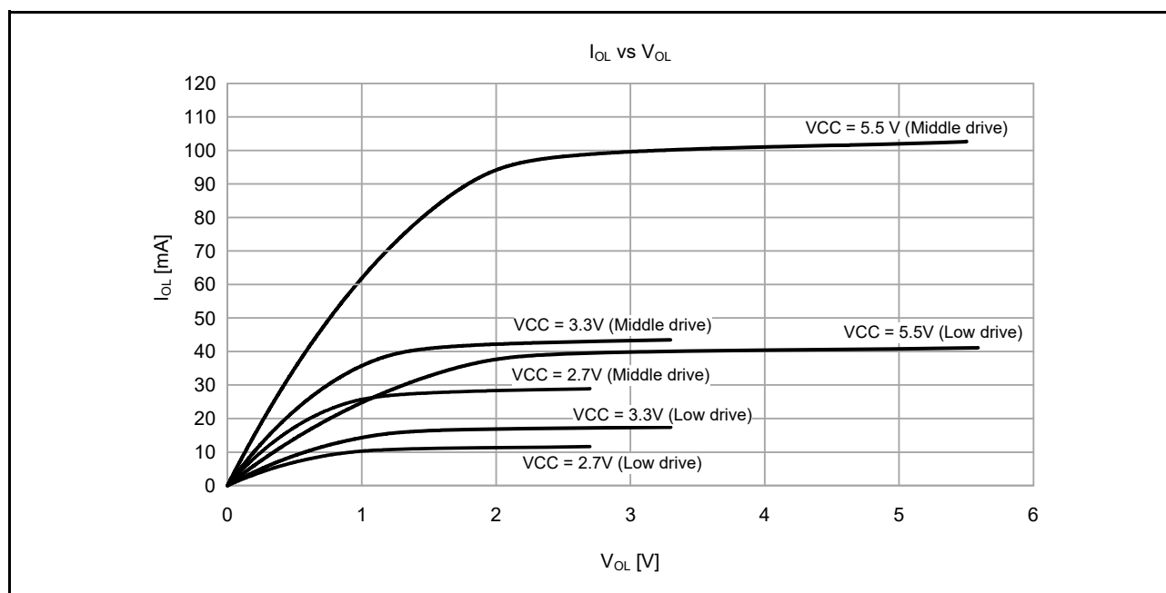
Figure 52.16 V_{OH}/V_{OL} and I_{OH}/I_{OL} voltage characteristics at T_a = 25^\circ\text{C}
