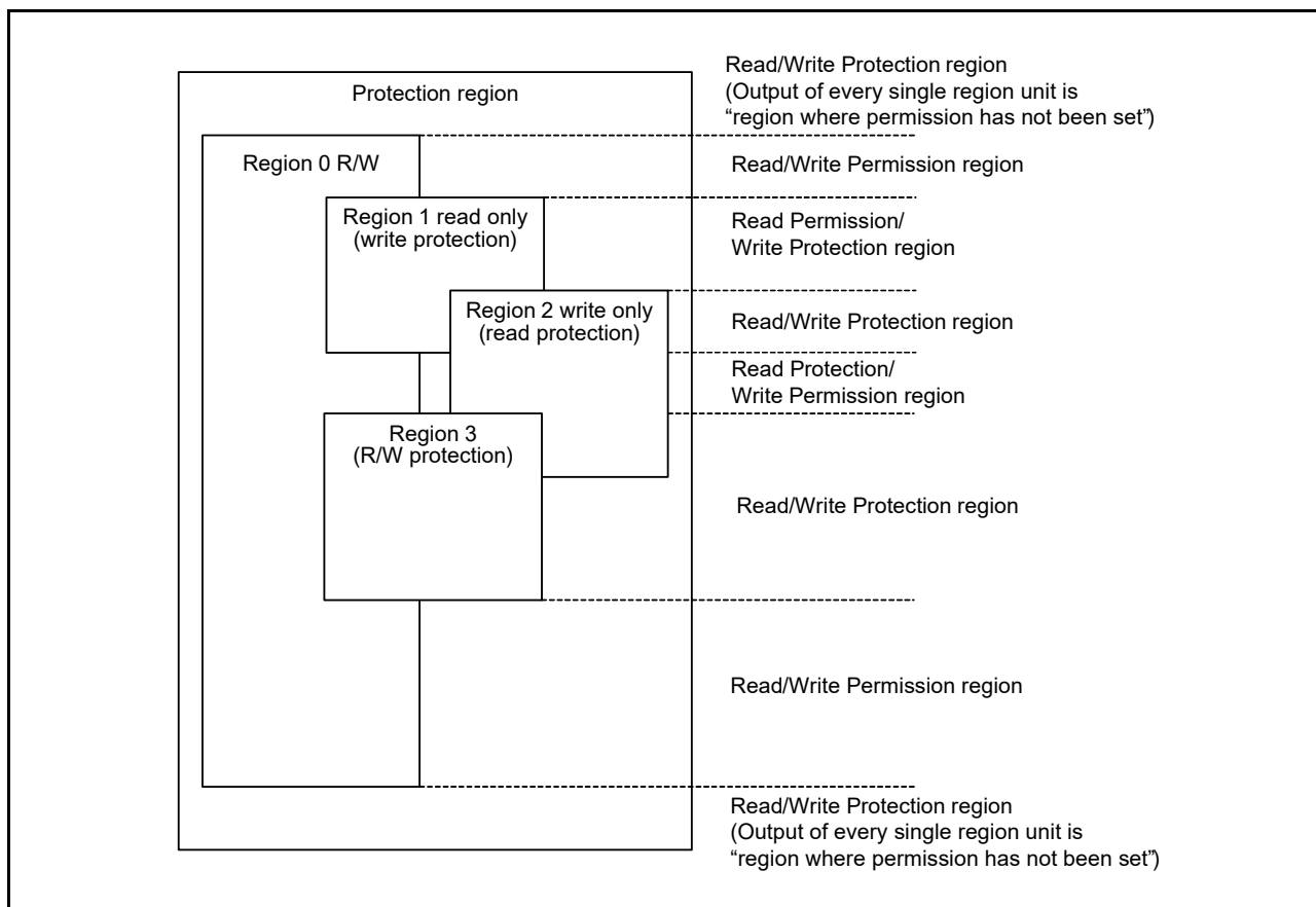
Figure 16.6 Access permission or protection by overlap of the bus master MPU region
