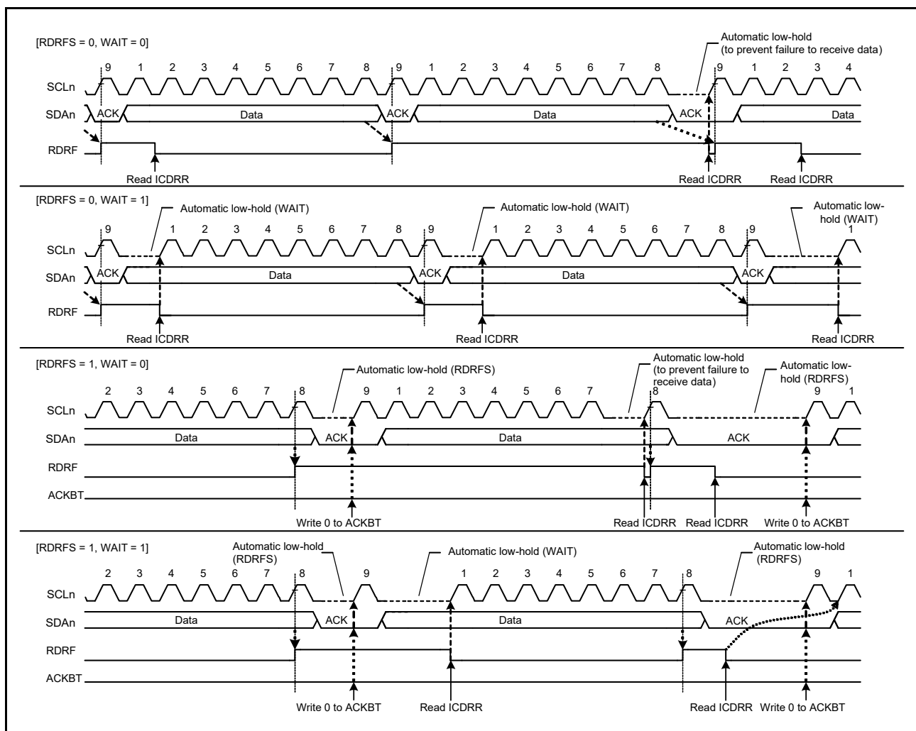
Figure 31.40 Automatic low-hold operation in receive mode using RDRFS and WAIT bits
