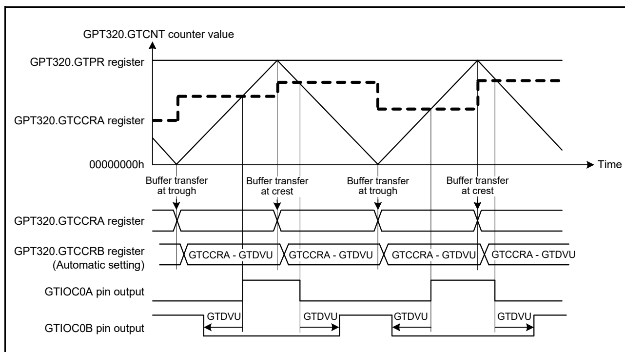
Figure 23.42 Example of automatic compare-match value setting function with dead time (triangle-wave PWM mode 2 or 3, active-high)
