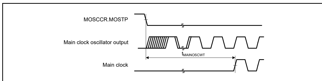
Figure 52.30 Main clock oscillation start timing
