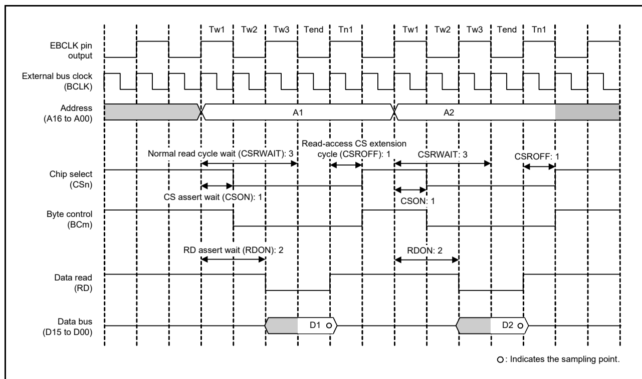
Figure 15.13 Example of normal read operation when BCLK/2 is selected in the EBCLK Pin Output Select bit (n = 0 to 3, m = 0, 1)
