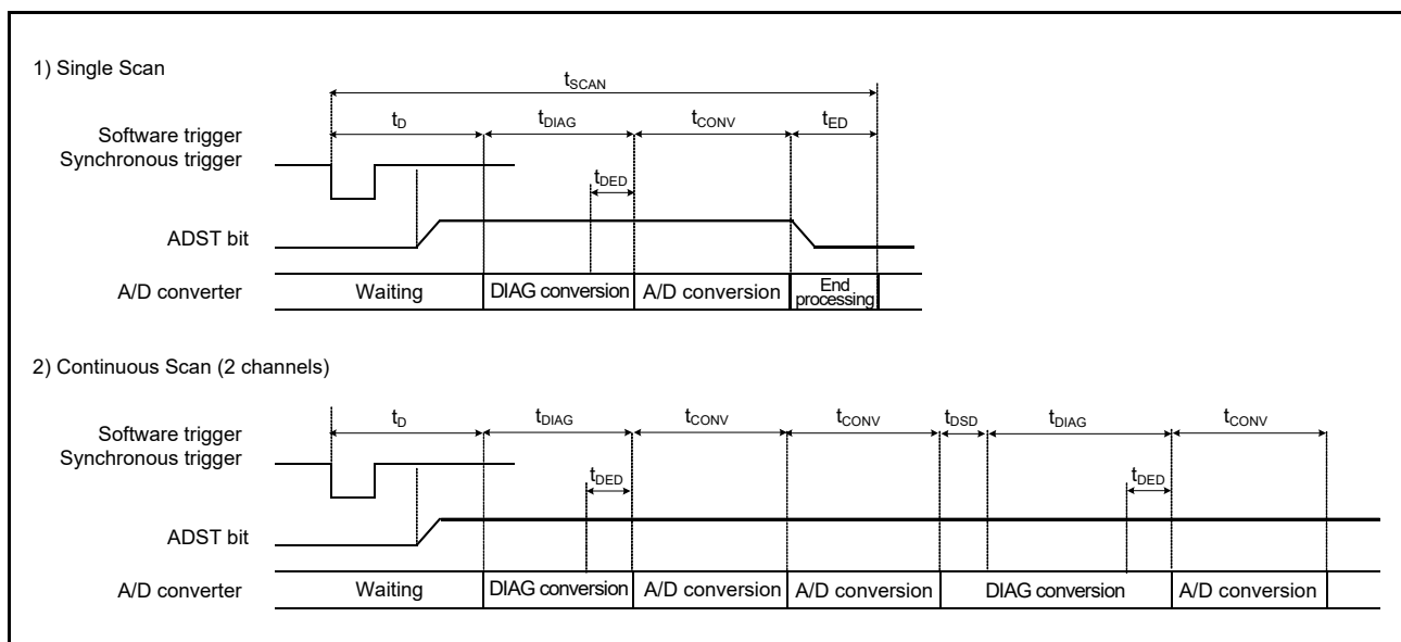
Figure 39.24 Scan conversion timing activated by software or synchronous trigger ELC input
