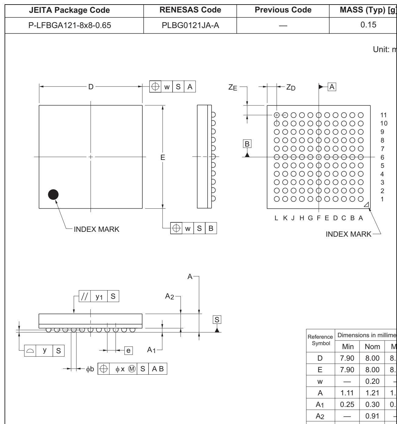
Figure 2.3 BGA 121-pin
