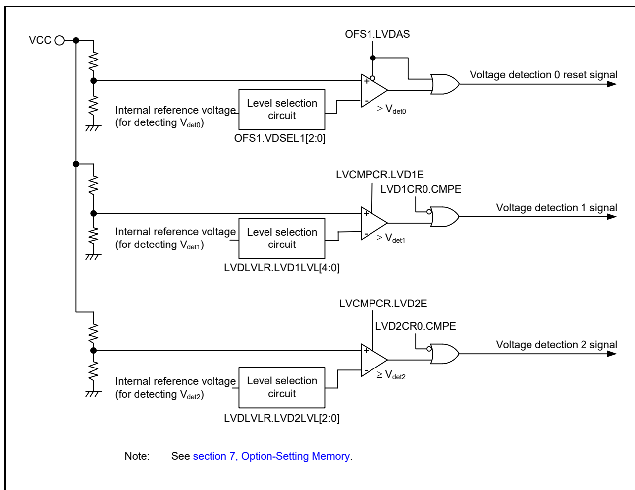
Figure 8.1 Voltage detection 0, 1, and 2 block diagram
