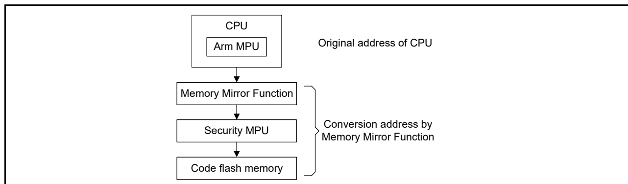
Figure 5.3 Address handling by each module
