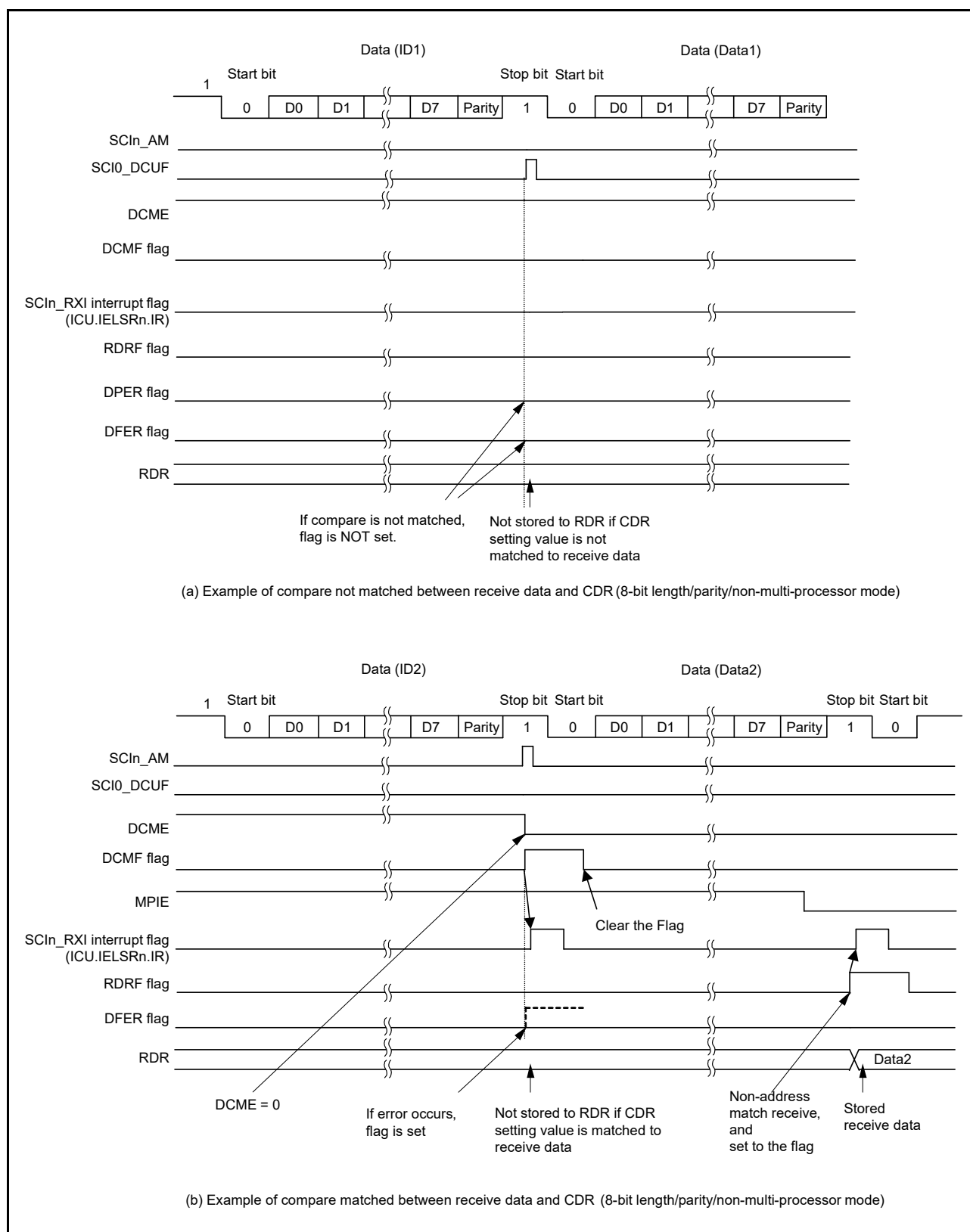
Figure 29.5 Example of address match (1) non-multi-processor mode
