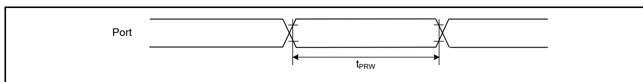
Figure 52.44 I/O ports input timing
