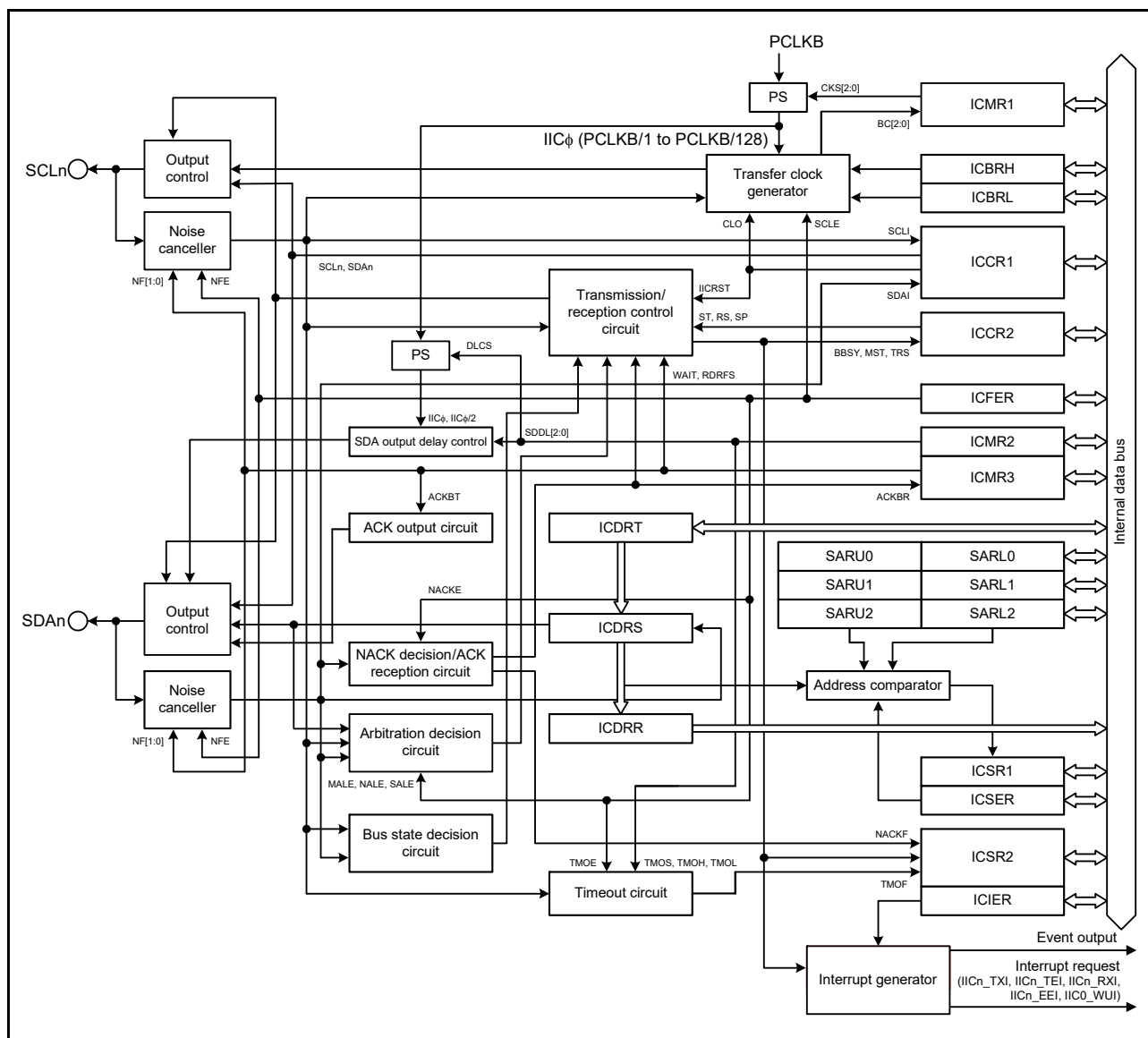
Figure 31.1 IIC block diagram
