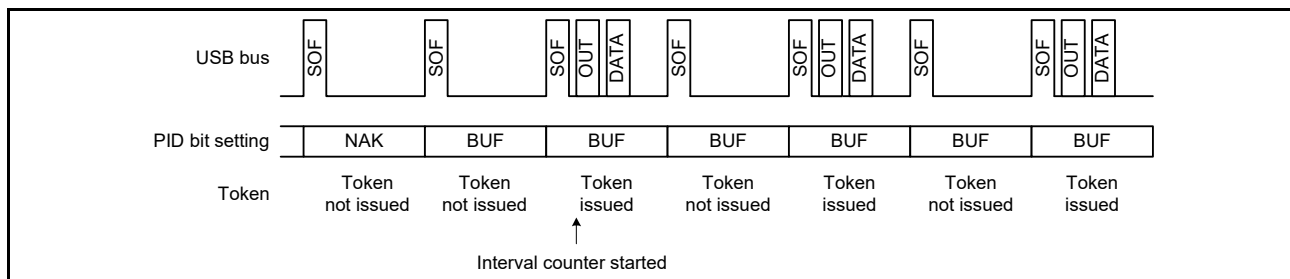
Figure 28.18 Token issuance when IITV = 1
