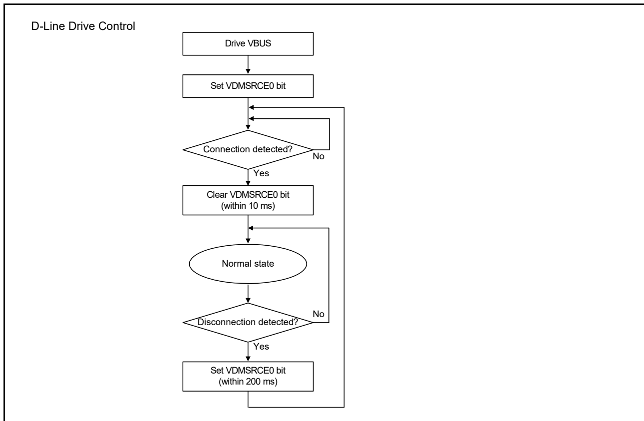
Figure 28.26 Process flow for operating as charging downstream port (steps a to b)
