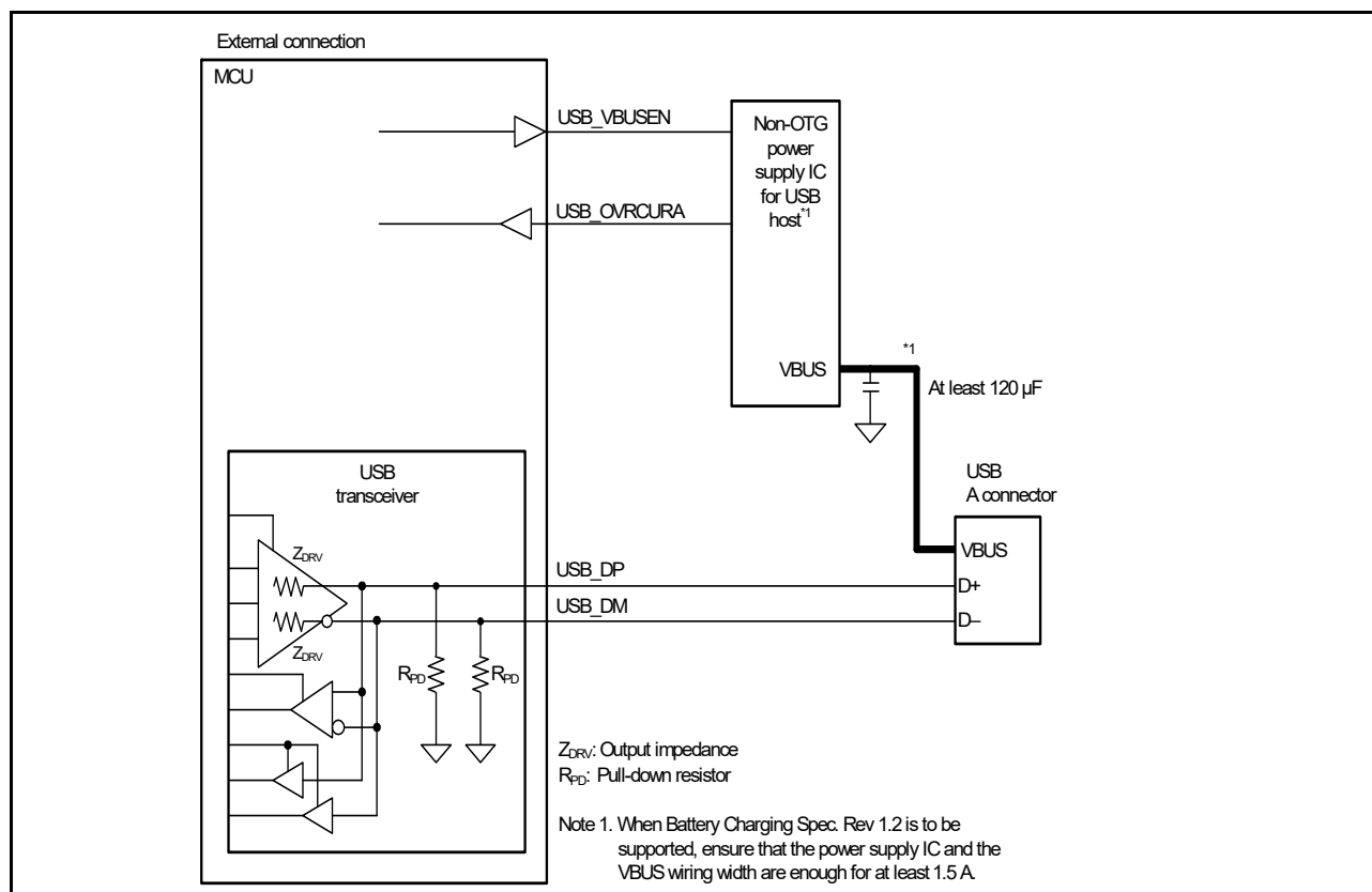
Figure 28.7 Example host connection
