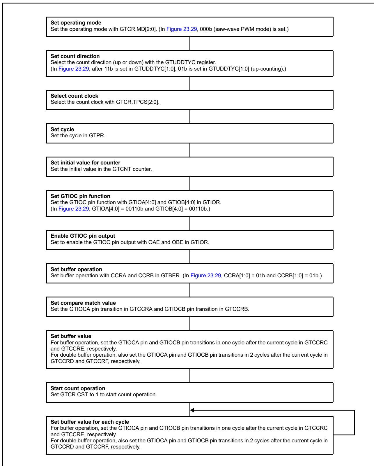
Figure 23.30 Example for setting saw-wave PWM mode
