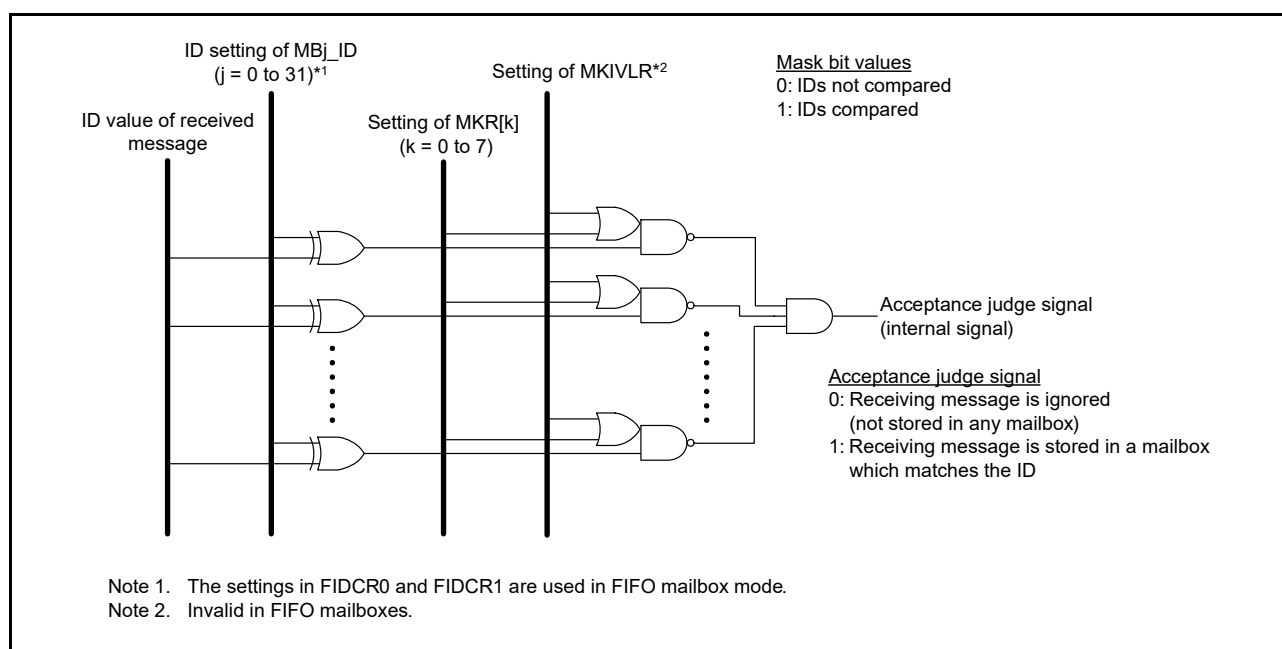
Figure 32.17 Acceptance filtering
