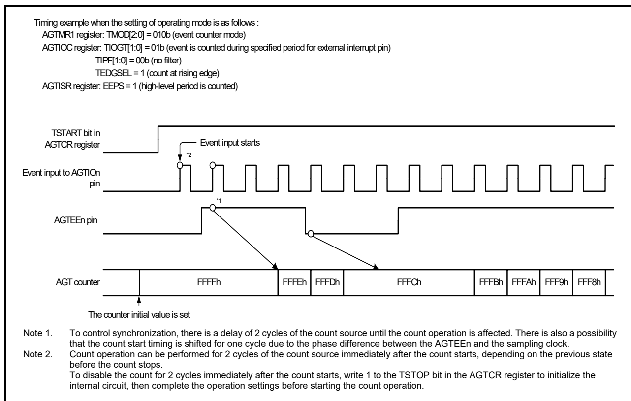
Figure 24.8 Operation example 2 in event counter mode
