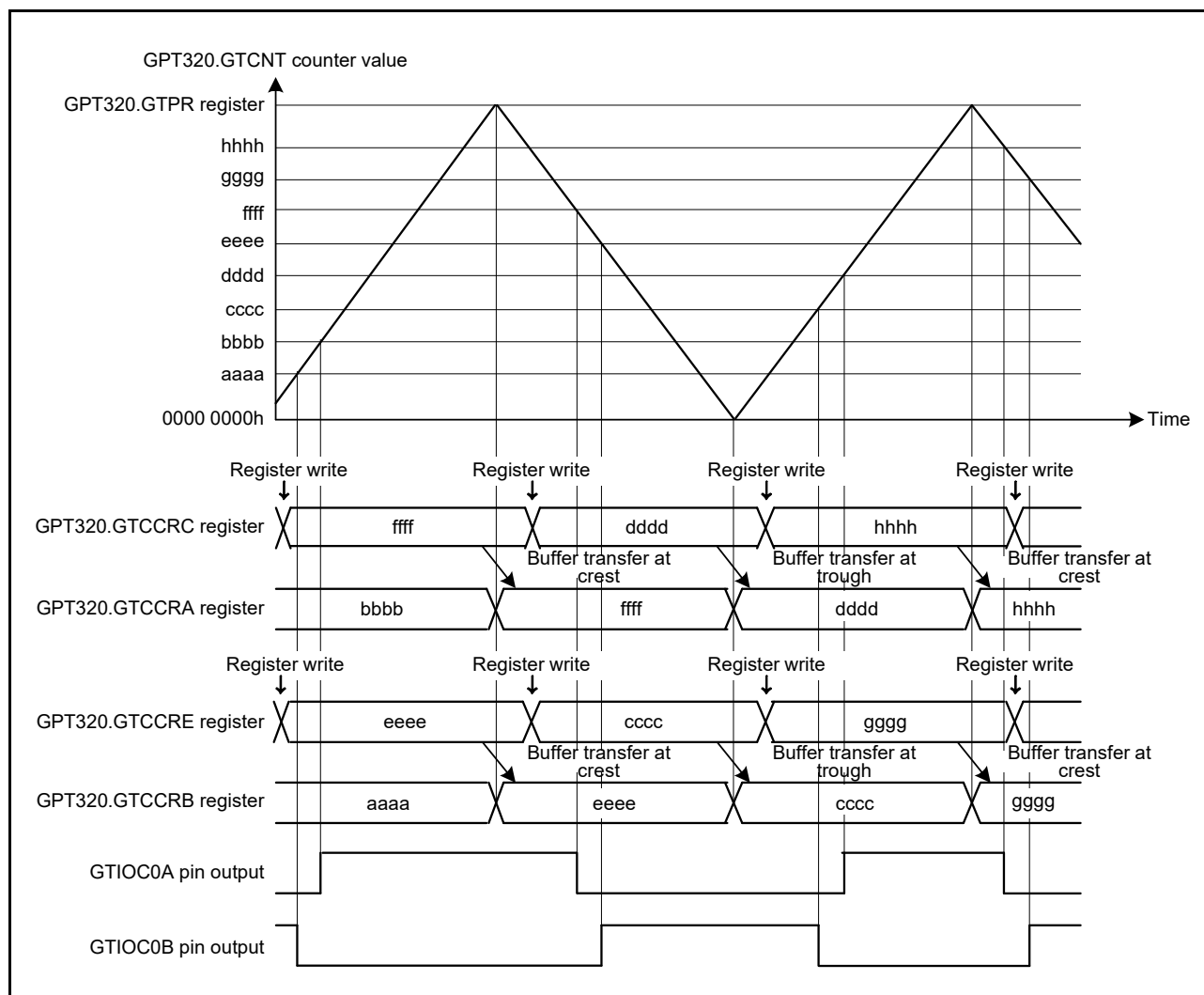
Figure 23.35 Example of triangle-wave PWM mode 2 operation (buffer operation, low output from the GTIOCA pin and high output from the GTIOCB pin at count start, output toggled at GTCCRA/GTCCRB compare match, output retained at cycle end)
