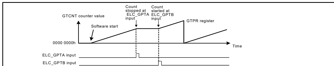
Figure 23.49 Example of count stop operation by hardware source started by software, stopped at ELC_GPTA input, restarted at ELC_GPTB input
