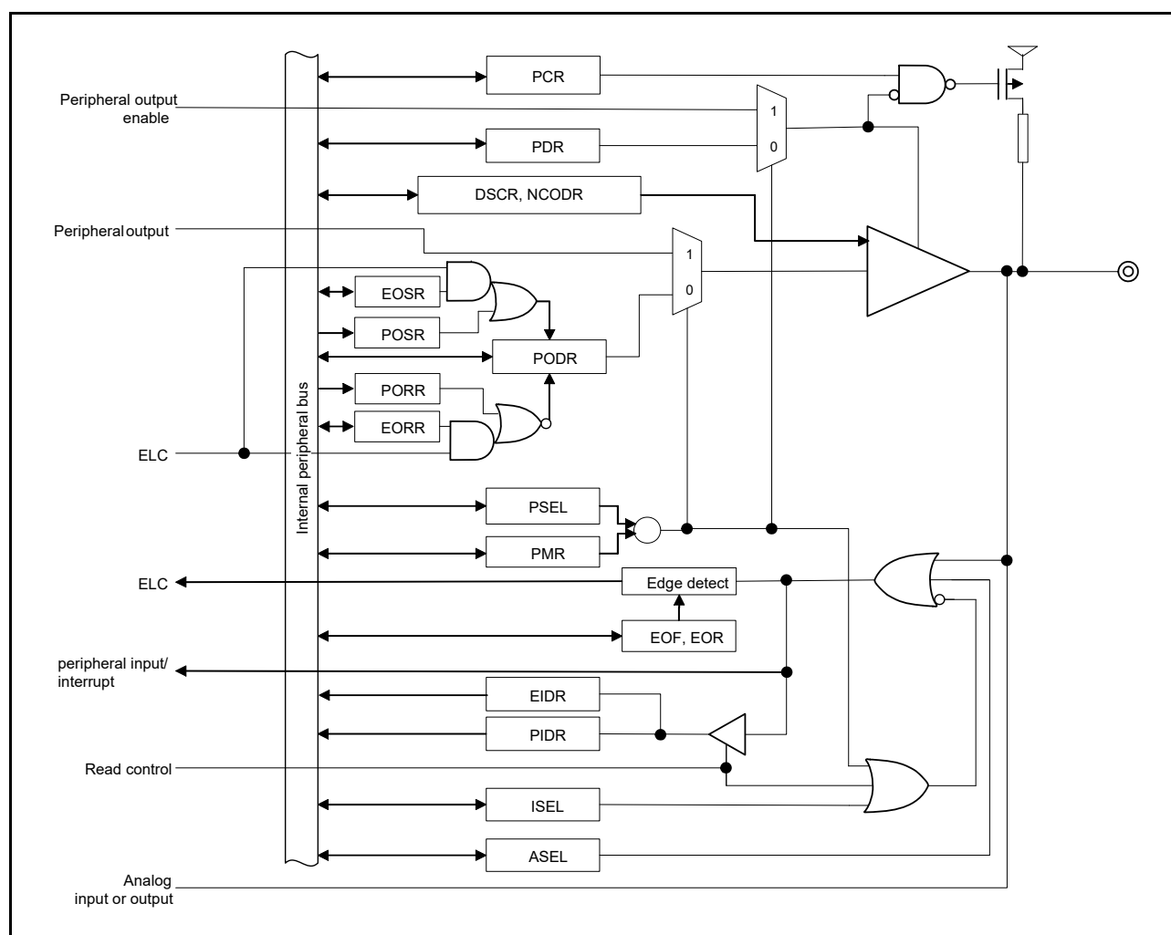
Figure 20.1 I/O Ports registers connection diagram
