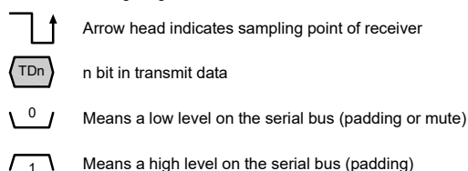
Figure 36.7 Basic format example in transmit mode
