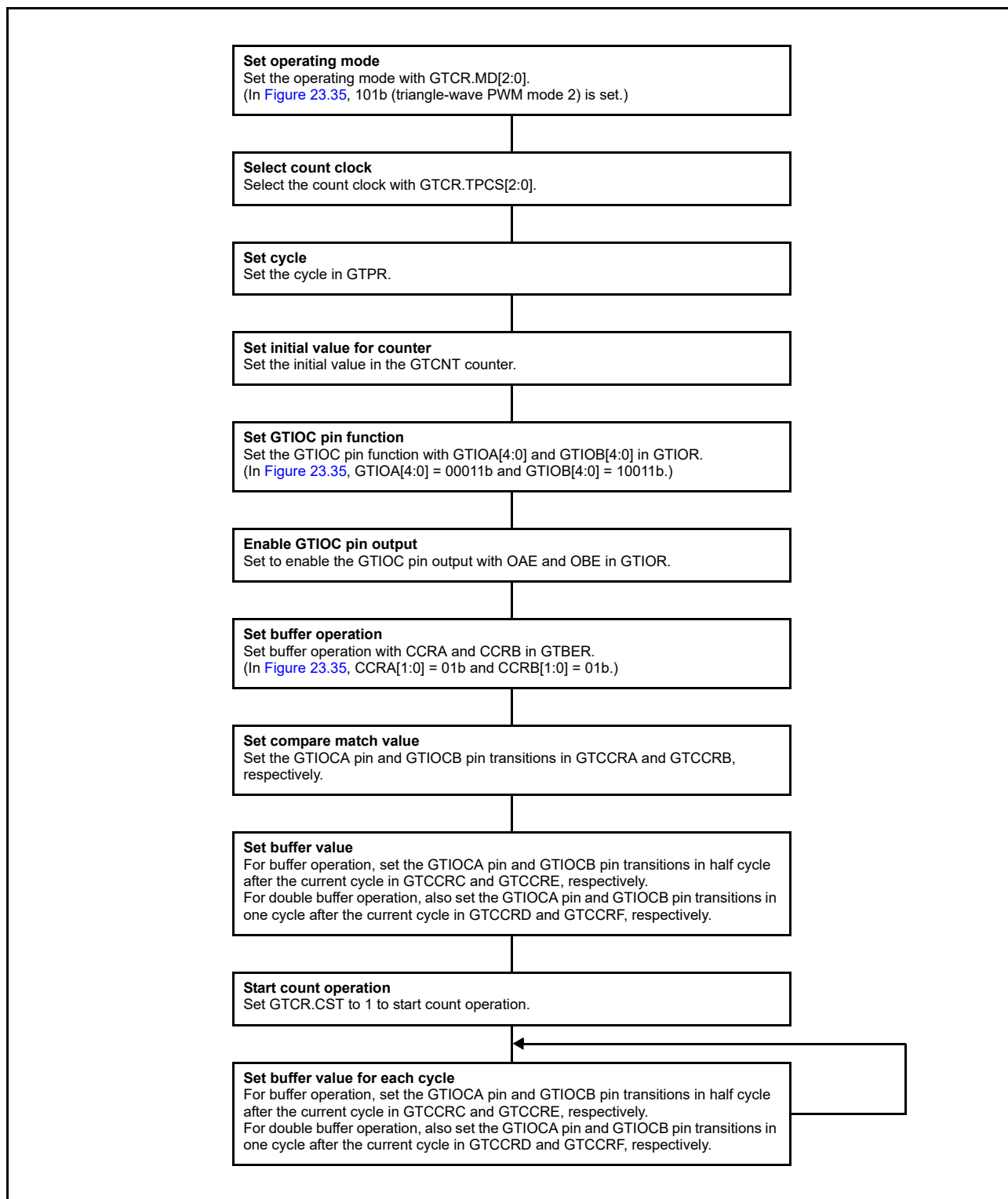
Figure 23.36 Example for setting triangle-wave PWM mode 2
