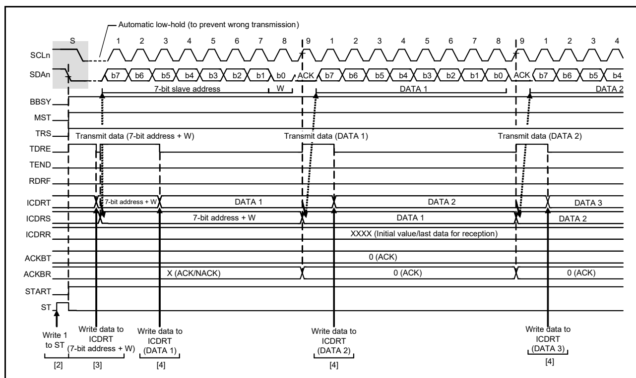
Figure 31.7 Master transmit operation timing (1) (7-bit address format)
