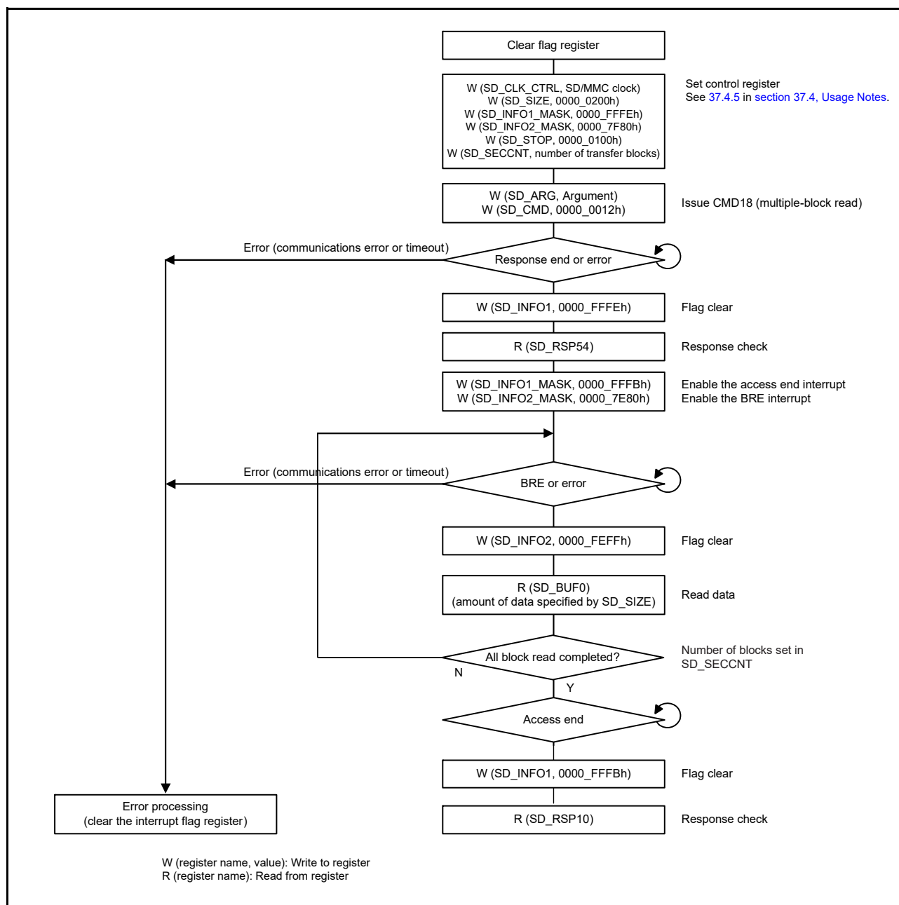
Figure 37.12 Example flow of multiple block read operation
