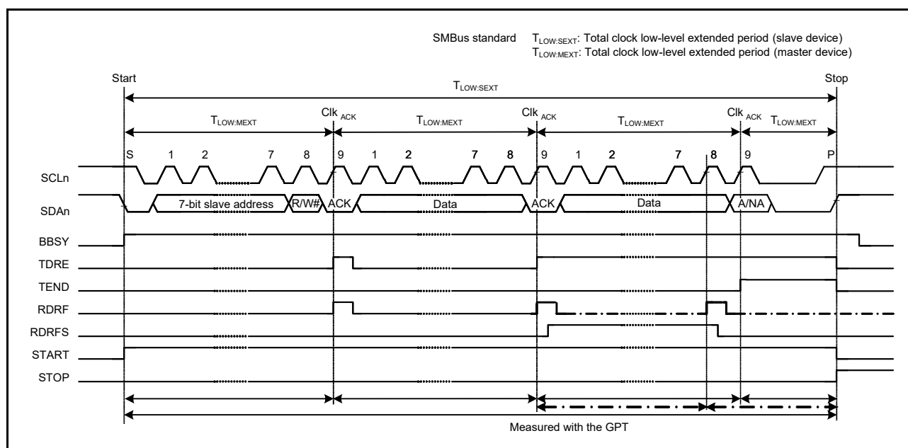
Figure 31.50 SMBus timeout measurement
