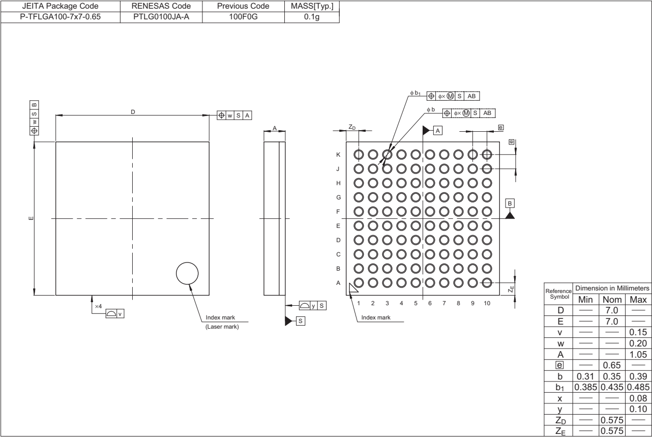
Figure 2.4 LGA 100-pin
