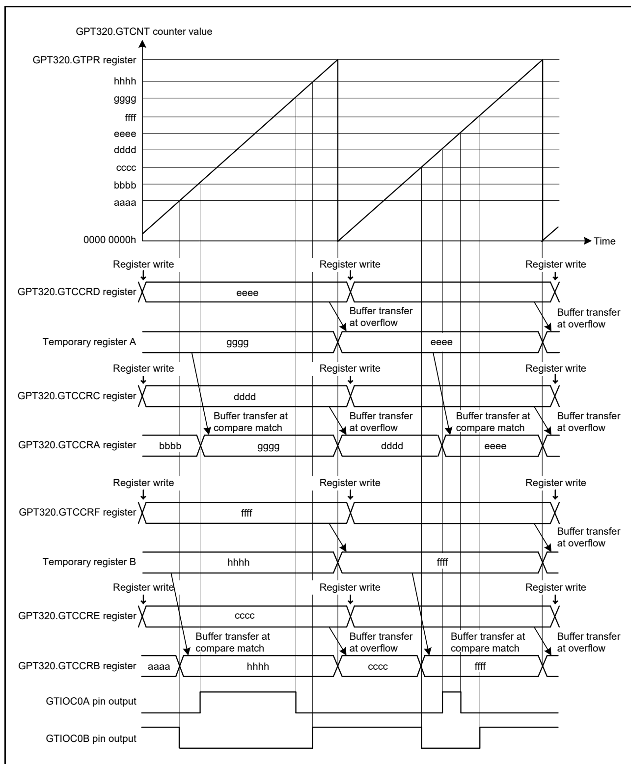
Figure 23.31 Example of saw-wave one-shot pulse mode operation (up-counting, low output from the GTIOC0A pin and high output from the GTIOC0B pin at count start, output toggled at GTCCRA/GTCCRB compare match, output retained at cycle end)
