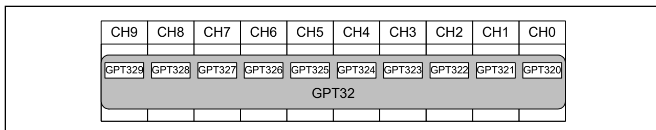
Figure 23.2 Correspondence between GPT channels and module names
