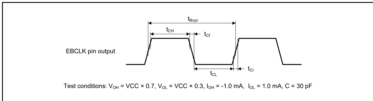
Figure 52.26 EBCLK pin output timing
