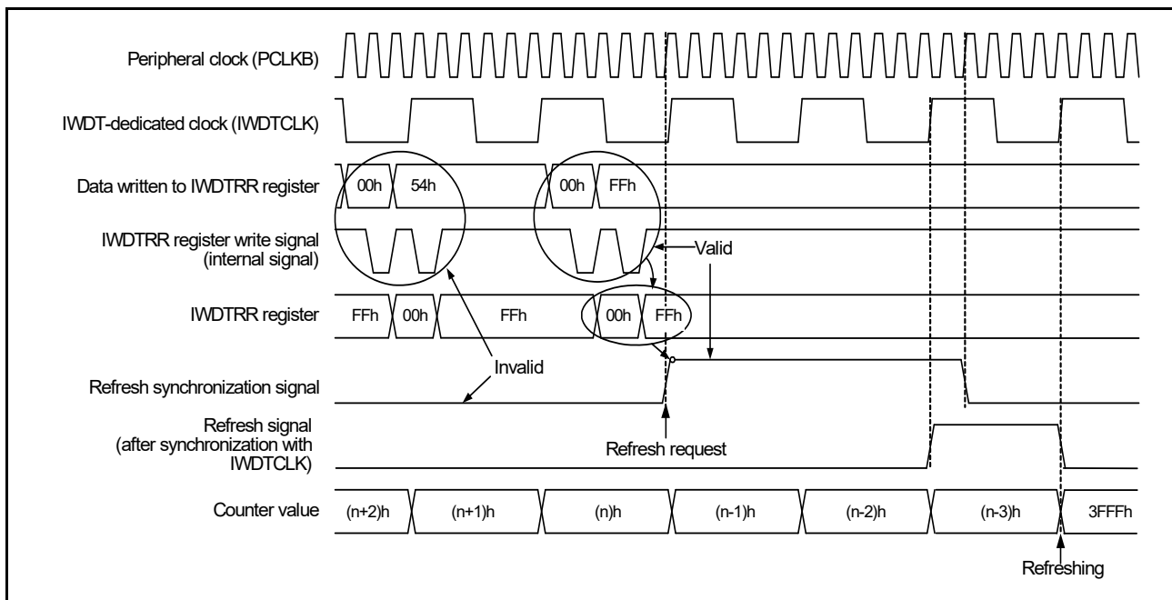
Figure 27.4 IWDT refresh operation waveforms (OFS0.IWDTCCKS[3:0] = 0000b, OFS0.IWDTCCKS[1:0] = 11b)
