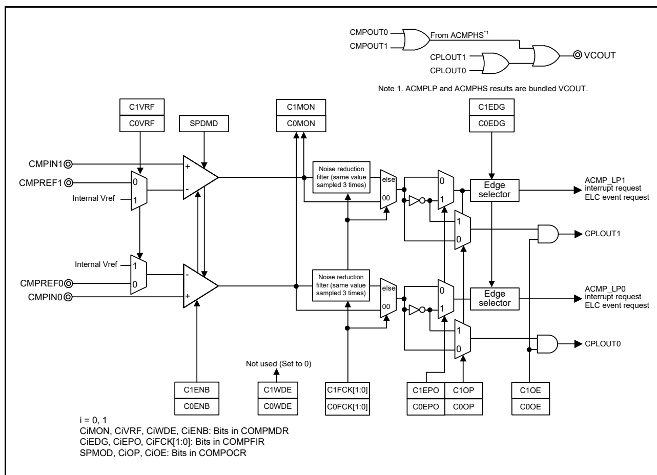
Figure 44.1 ACMPLP block diagram when window function is disabled
