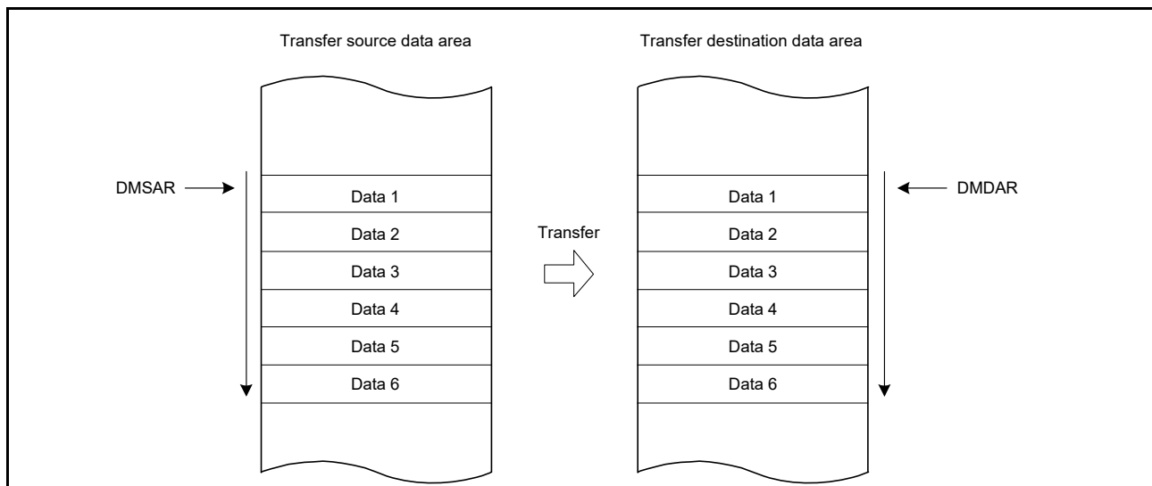
Figure 17.2 Operation in normal transfer mode
