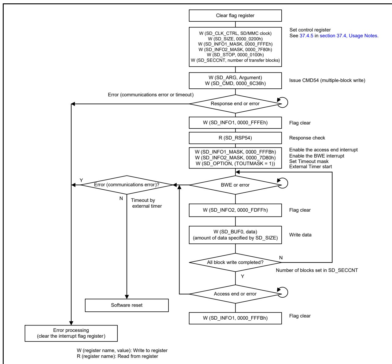
Figure 37.14 Example flow of multiple block write operation using external timer
