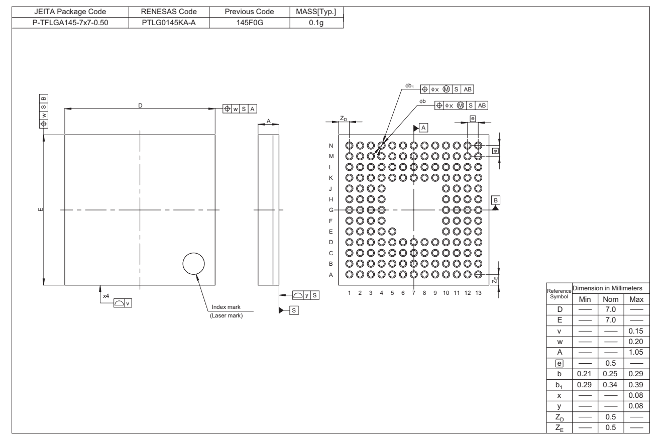
Figure 2.1 LGA 145-pin
