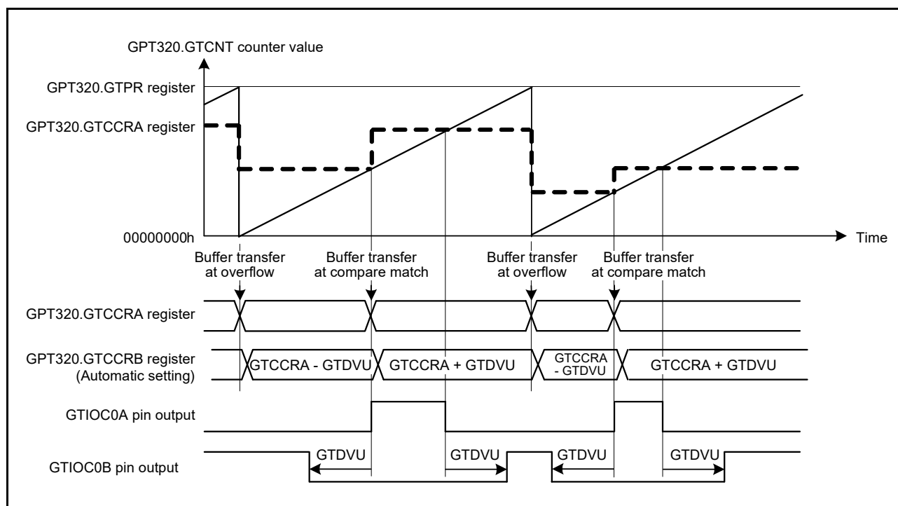
Figure 23.39 Example of automatic dead time setting function operation (saw-wave one-shot pulse mode, up-counting, active-high)
