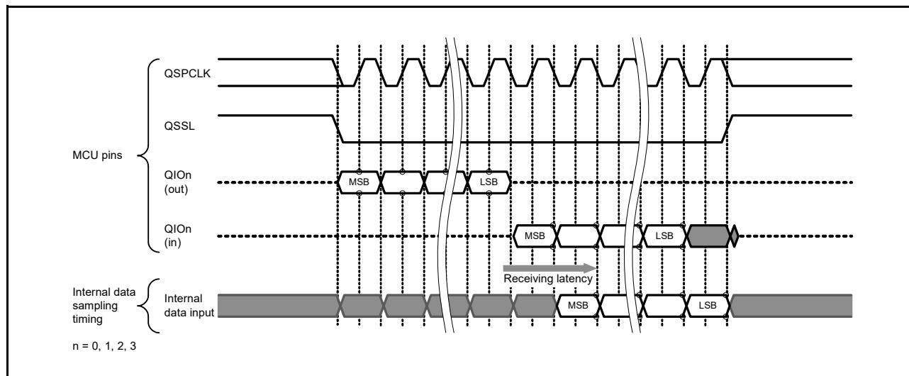
Figure 34.15 Receiving latency
