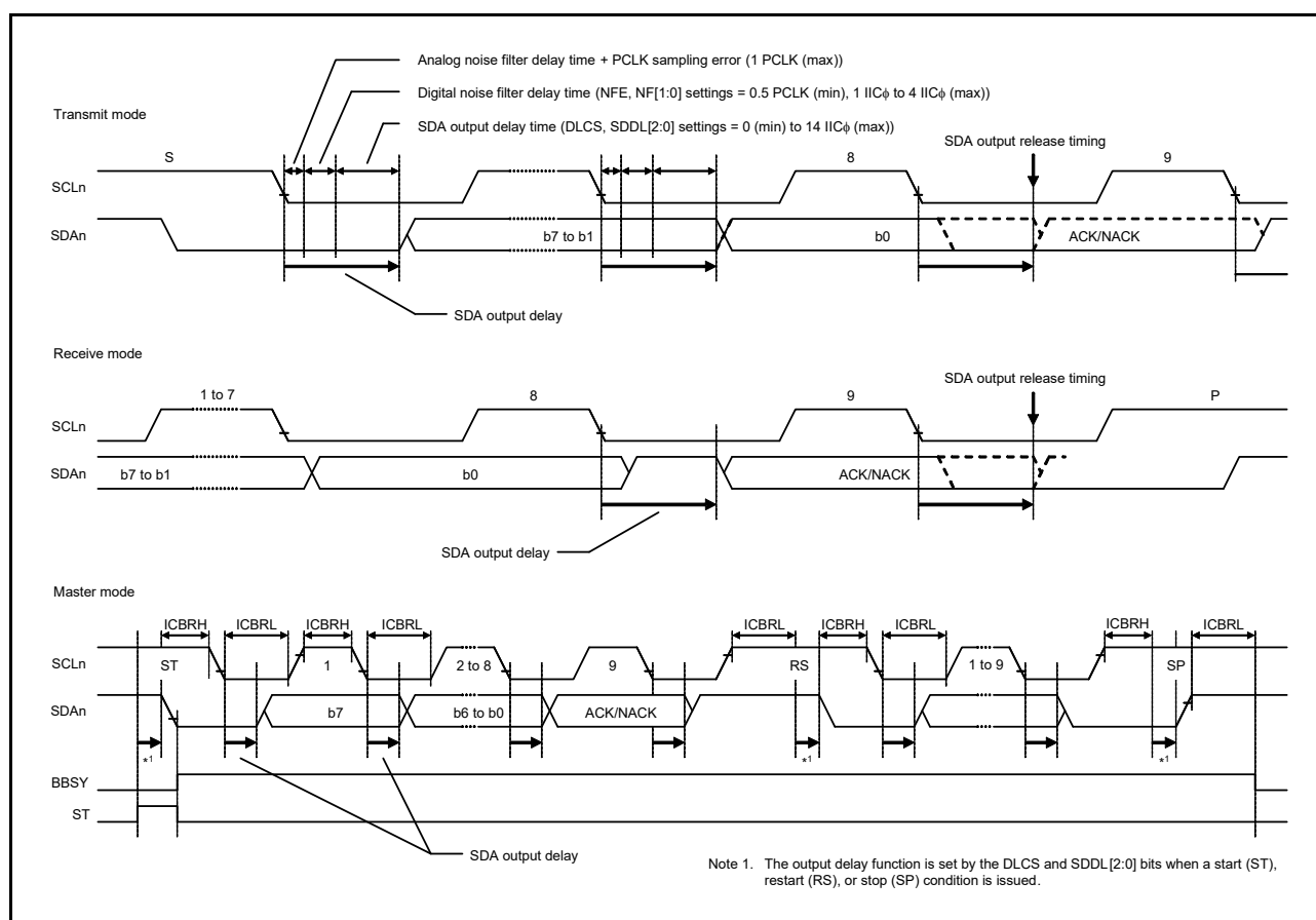
Figure 31.22 SDA output delay function
