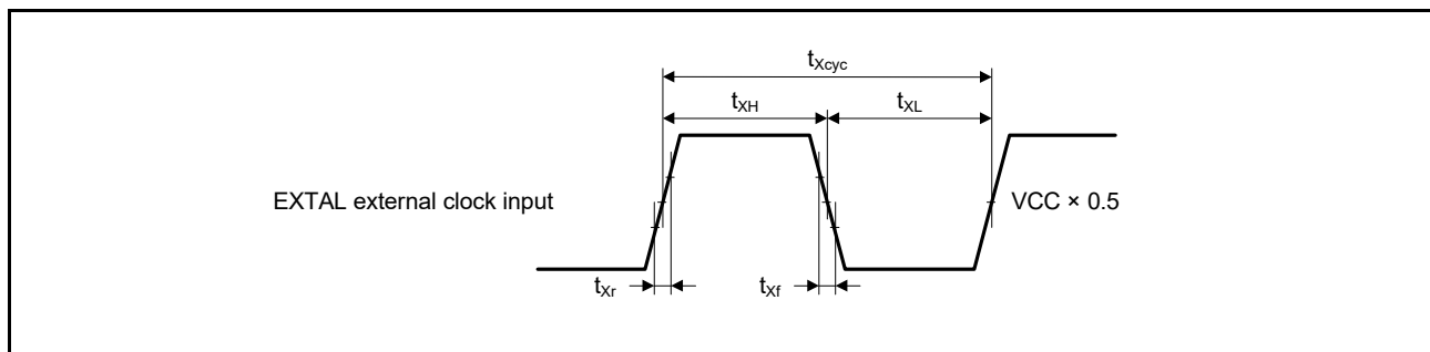
Figure 52.27 EXTERNAL external clock input timing
