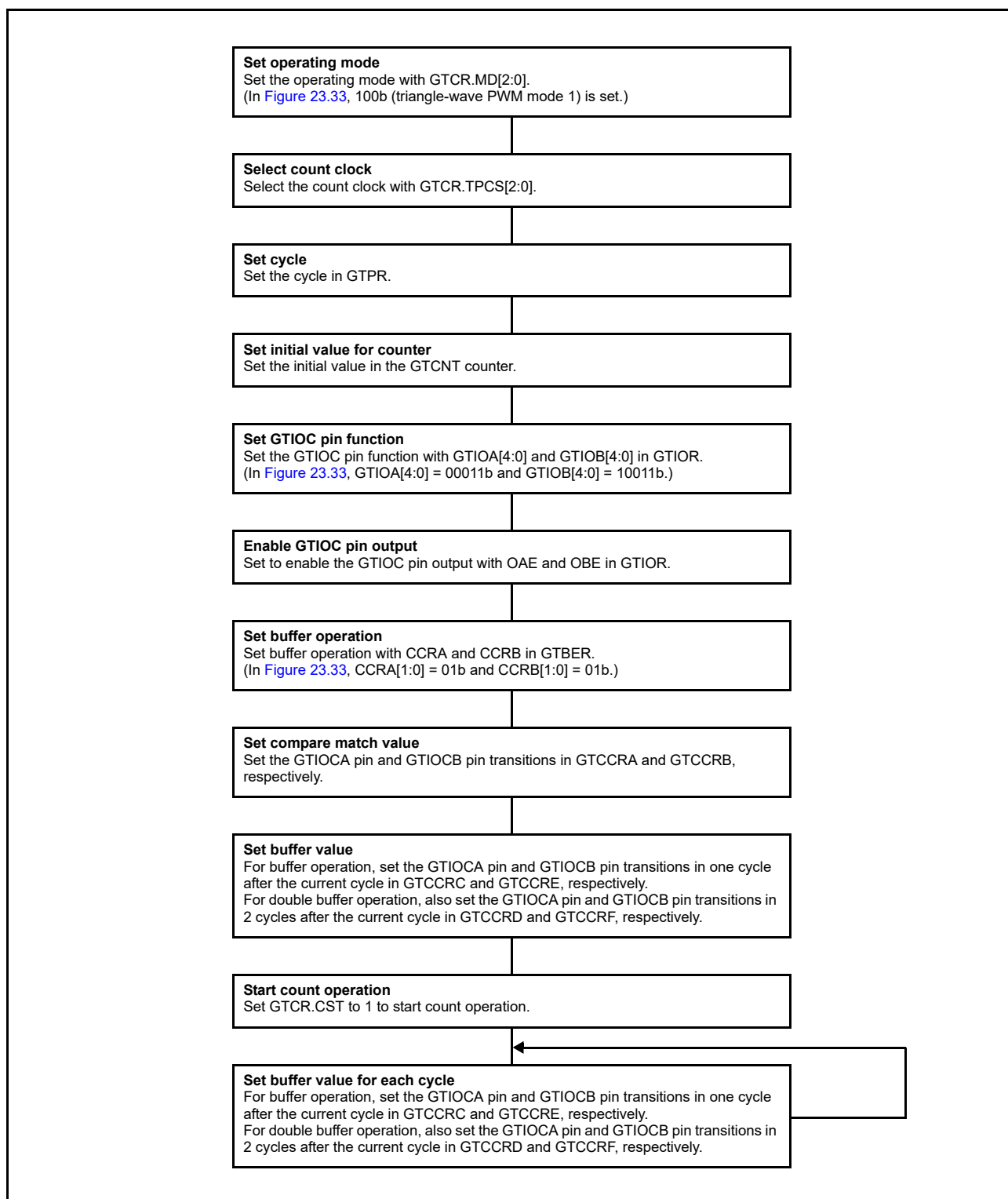
Figure 23.34 Example for setting triangle-wave PWM mode 1
