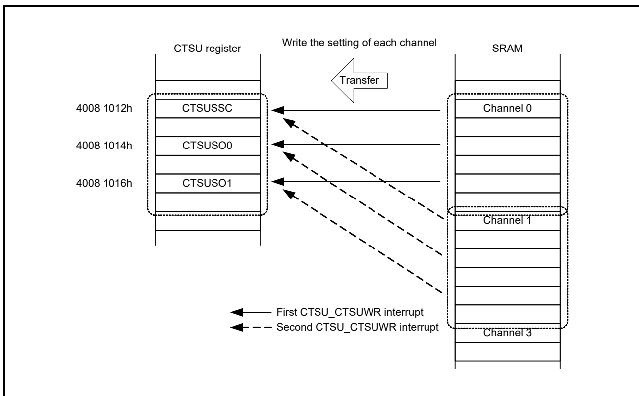
Figure 45.19 Example DTC transfer operation using the CTSU_CTSUWR interrupt
