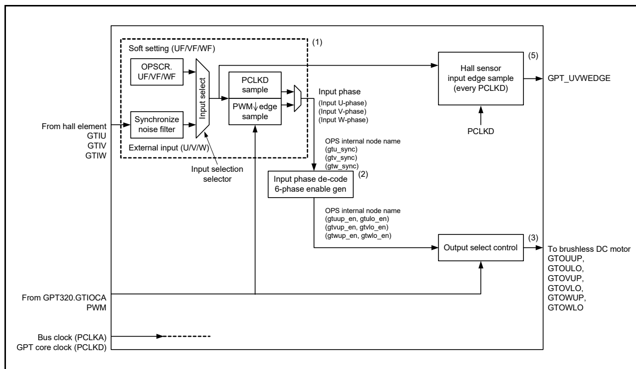
Figure 23.77 GPT_OPS control flow conceptual diagram
