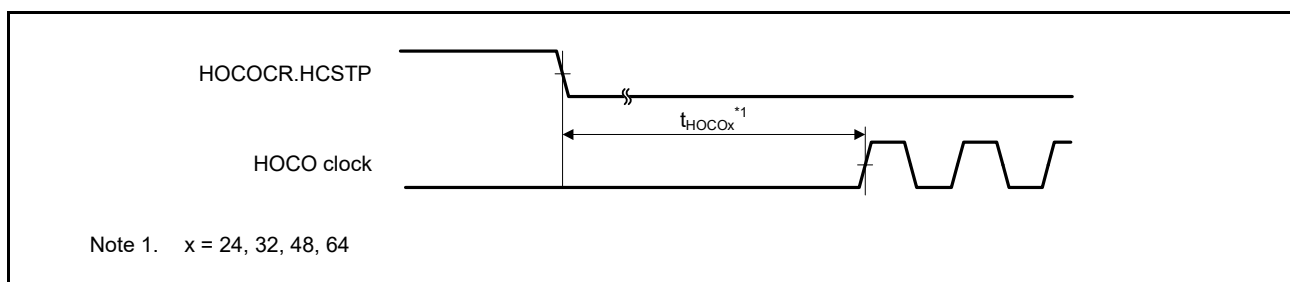
Figure 52.29 HOCO clock oscillator start timing (started by setting HOCOCR.HCSTP bit)
