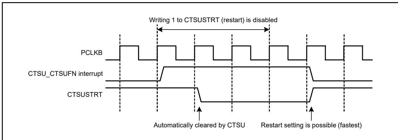
Figure 45.21 Notes on restarting measurement
