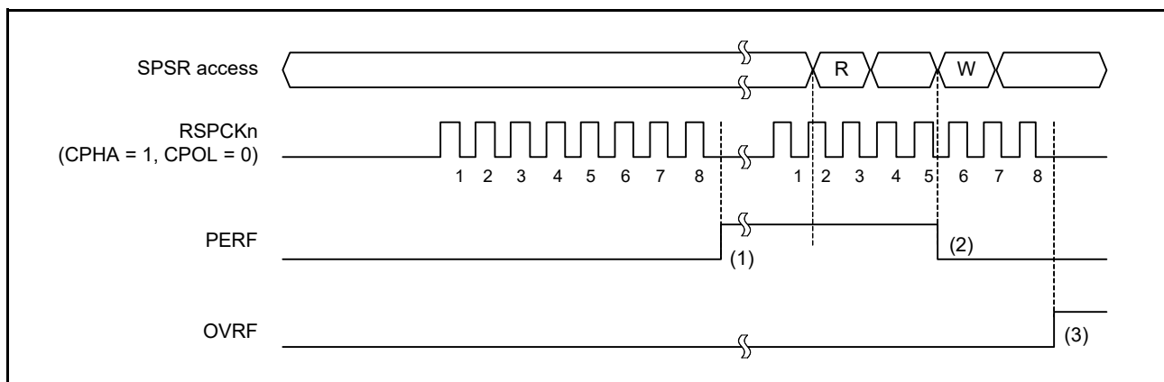
Figure 33.31 Operation example of PERF flag
