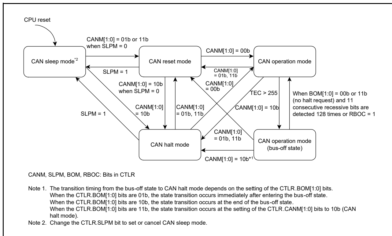
Figure 32.9 Transition between different modes of operation
