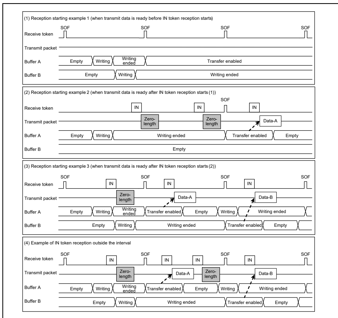
Figure 28.21 Example data setup operation
