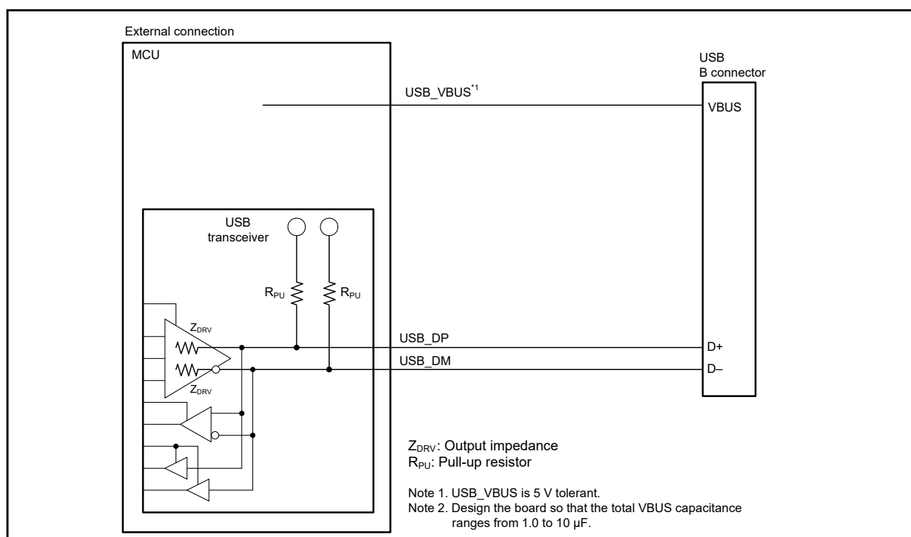
Figure 28.9 Example device connection in bus-powered state 2
