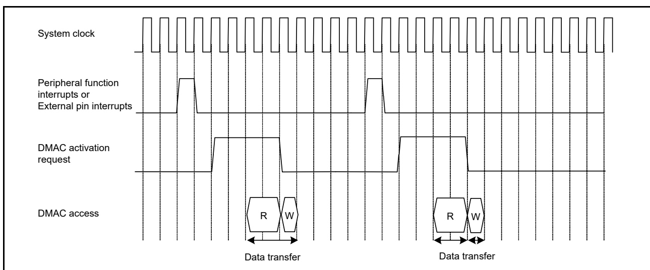
Figure 17.10 DMAC operation timing example (1) (DMA activation by interrupt from peripheral module/external interrupt input pin, normal transfer mode, repeat transfer mode)
