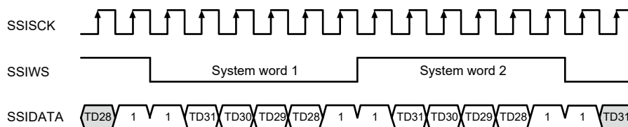
Figure 36.10 Inverted padding polarity
