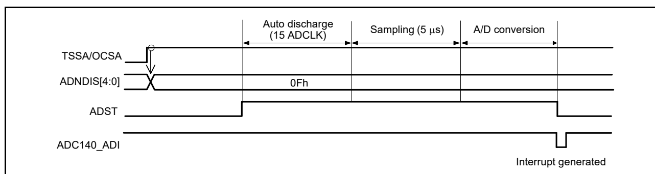
Figure 39.8 Example of operation in single-scan mode with basic operation: AN000 and temperature sensor output or internal reference voltage selected
