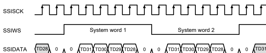
Figure 36.9 Inverted word select
