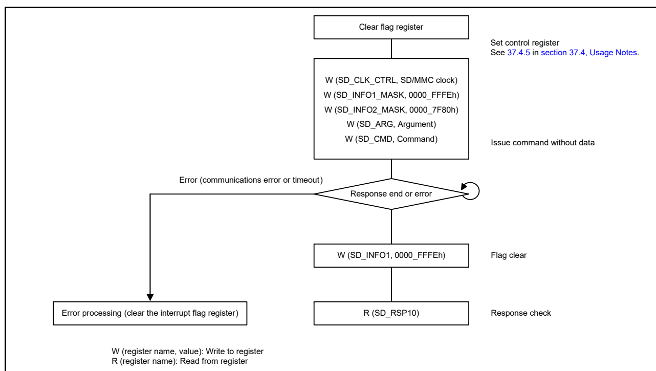
Figure 37.9 Example flow of command without data
