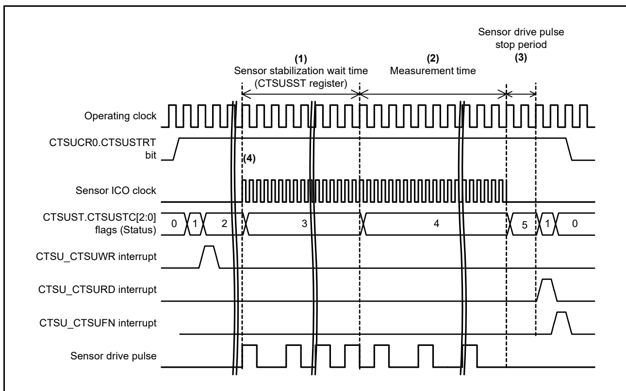
Figure 45.18 Sensor stabilization wait and measurement timing
