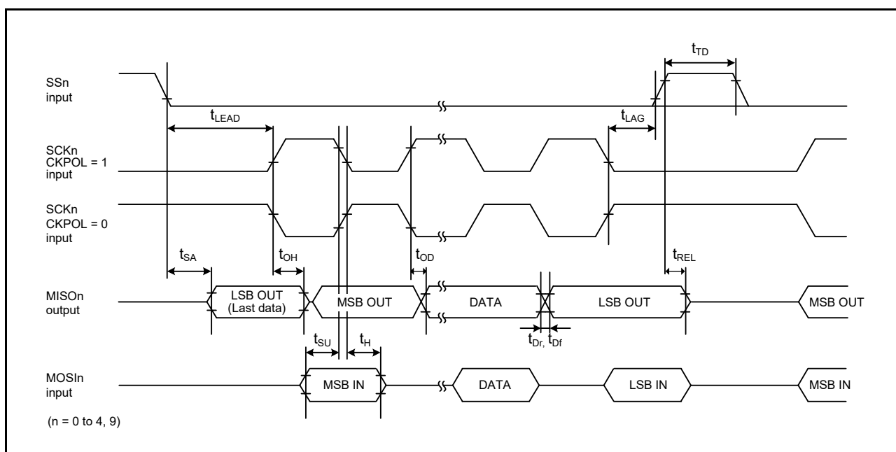
Figure 52.56 SCI simple SPI mode timing (slave, CKPH = 0)
