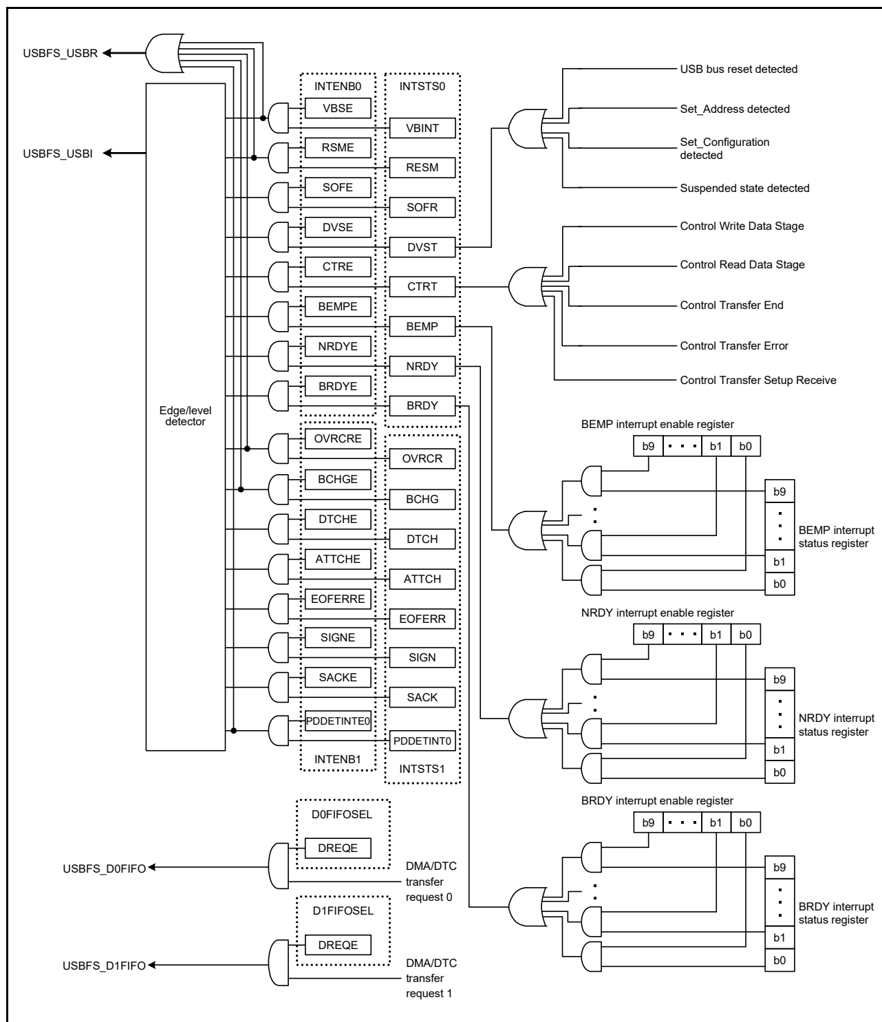
Figure 28.11 USBFS interrupt-related circuits
