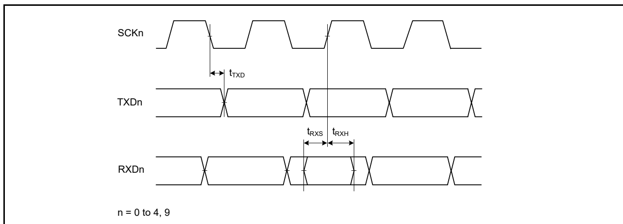
Figure 52.51 SCI input/output timing in clock synchronous mode
