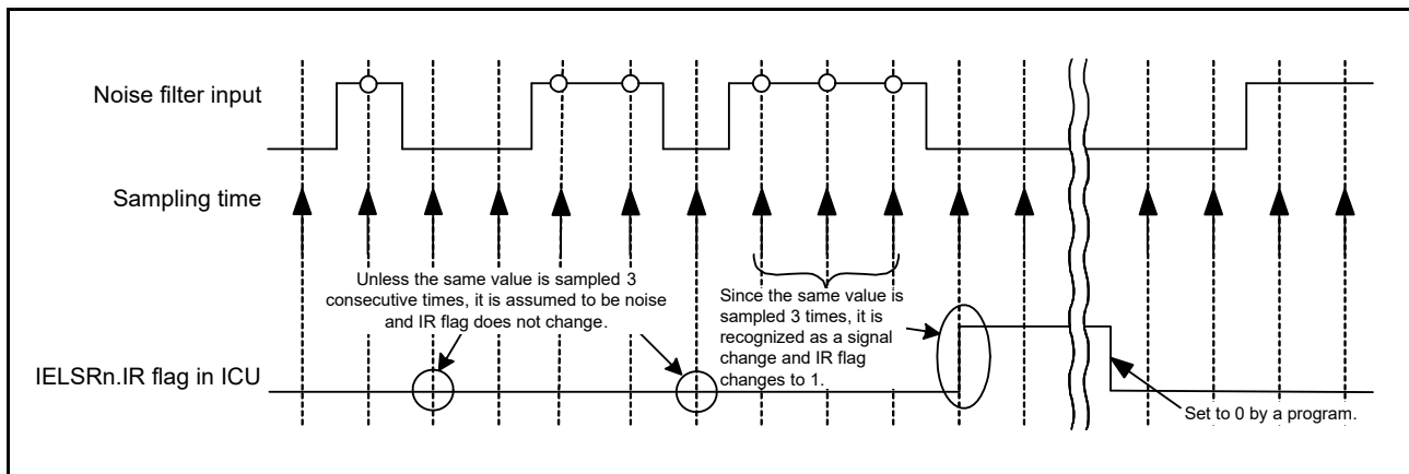
Figure 43.4 Noise filter and interrupt operation example
