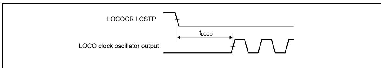
Figure 52.28 LOCO clock oscillator start timing
