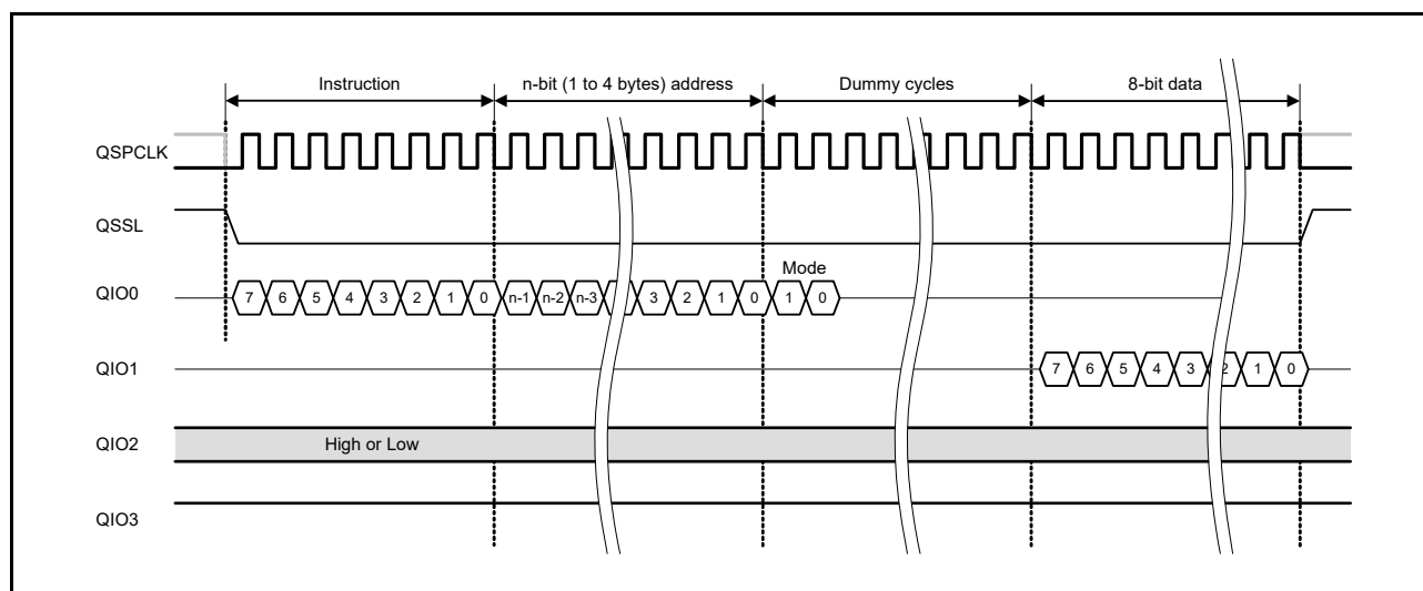
Figure 34.4 Extended SPI protocol example 1 for Fast Read
