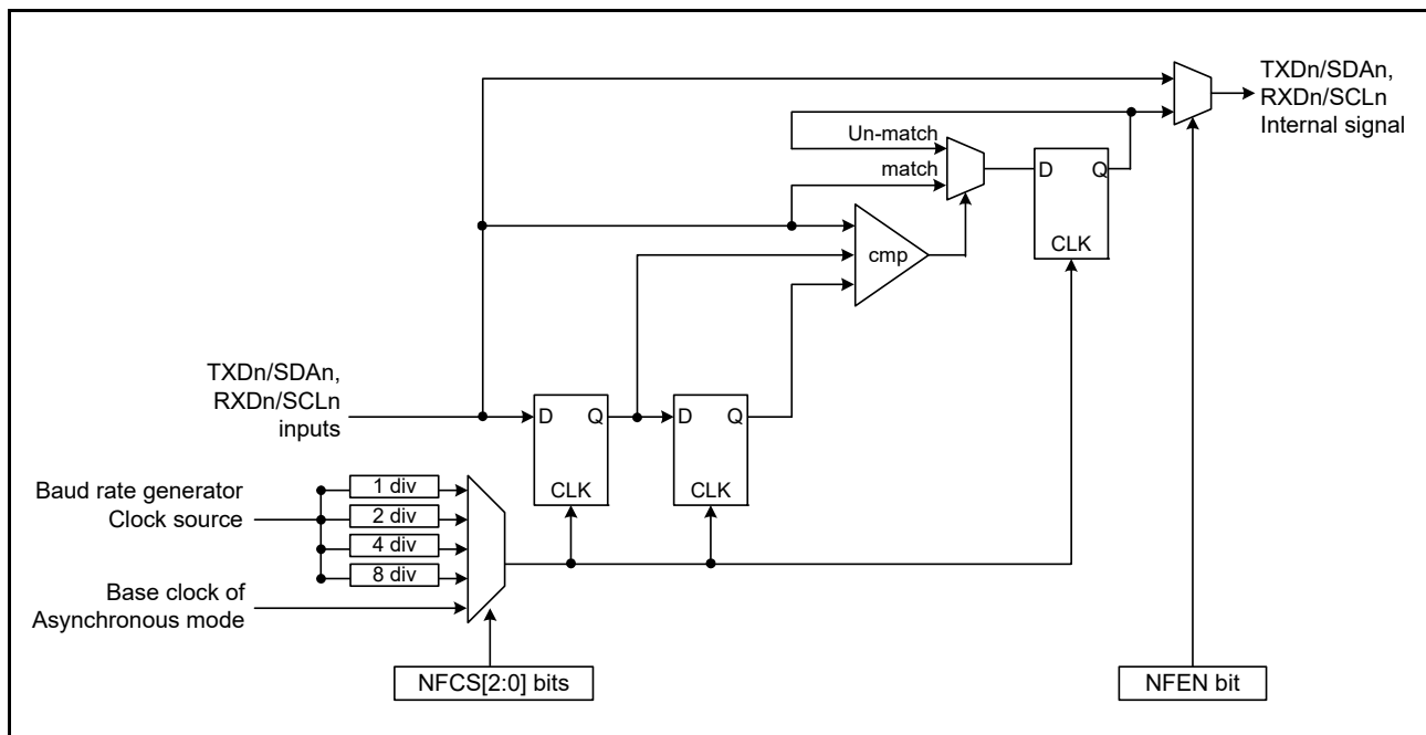
Figure 29.72 Digital noise filter circuit block diagram
