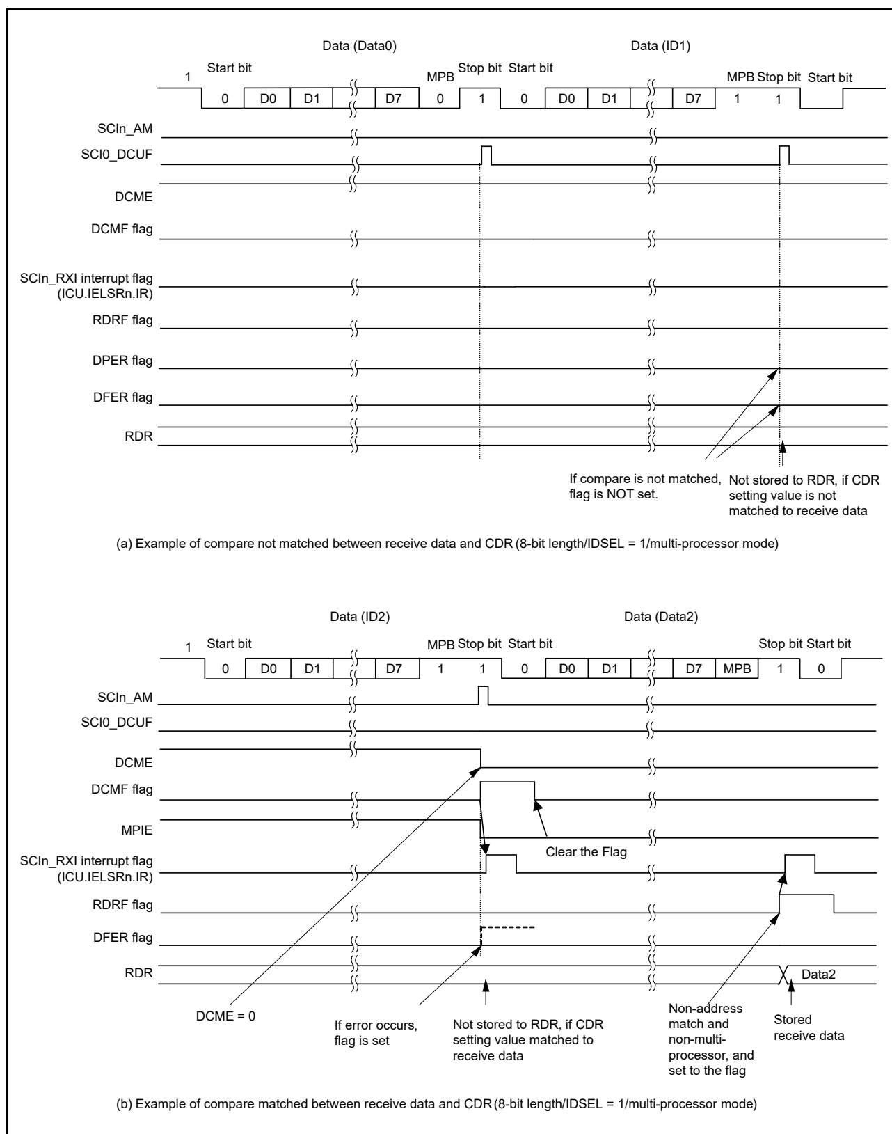
Figure 29.6 Example of address match (2) multi-processor mode
