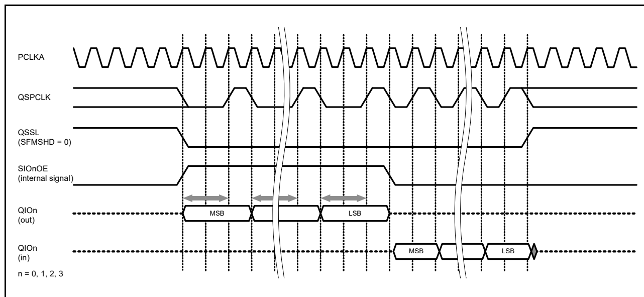
Figure 34.13 Setup time adjustment of serial data output with SFMOSW bit
