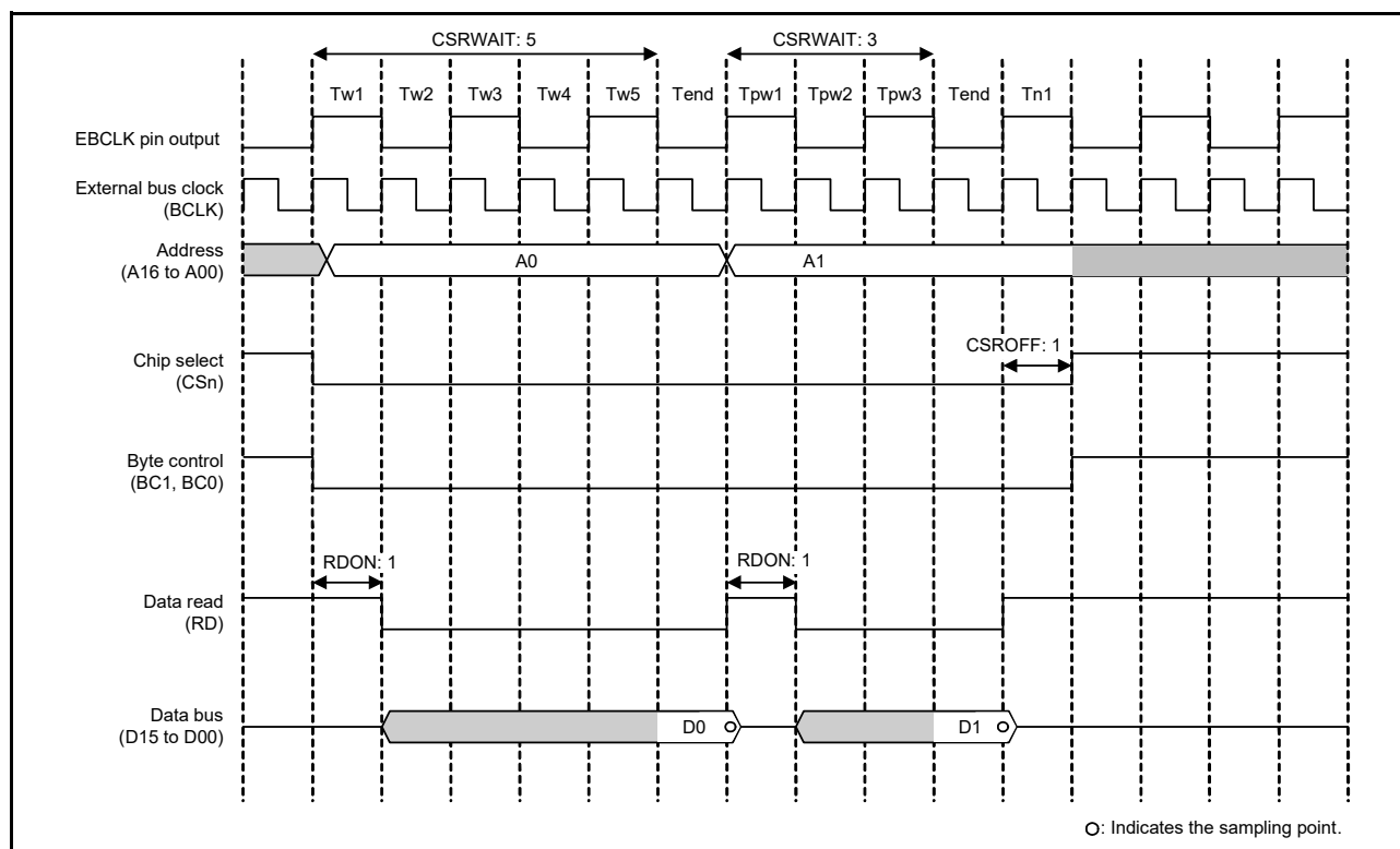
Figure 15.21 Example of page read access operation when BCLK/2 is selected in the EBCLK Pin Output Select bit and two rounds of bus access are generated in response to a single transfer request ( n = 0 to 3)
