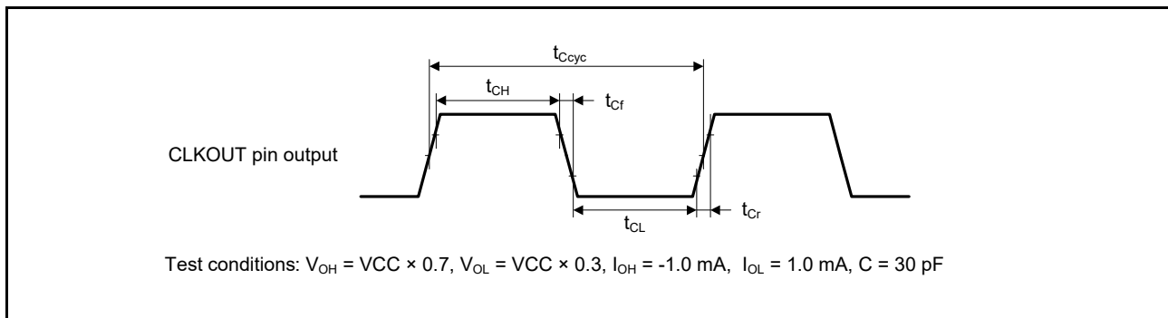
Figure 52.73 CLKOUT output timing
