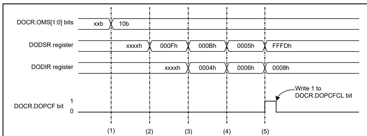
Figure 46.4 Example operation in data subtraction mode
