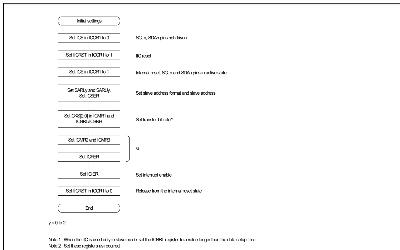
Figure 31.5 Example of IIC initialization flow
