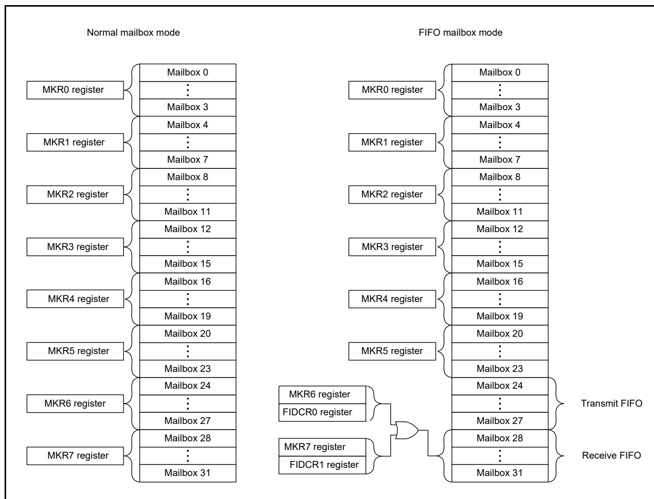
Figure 32.16 Associations between mask registers and mailboxes
