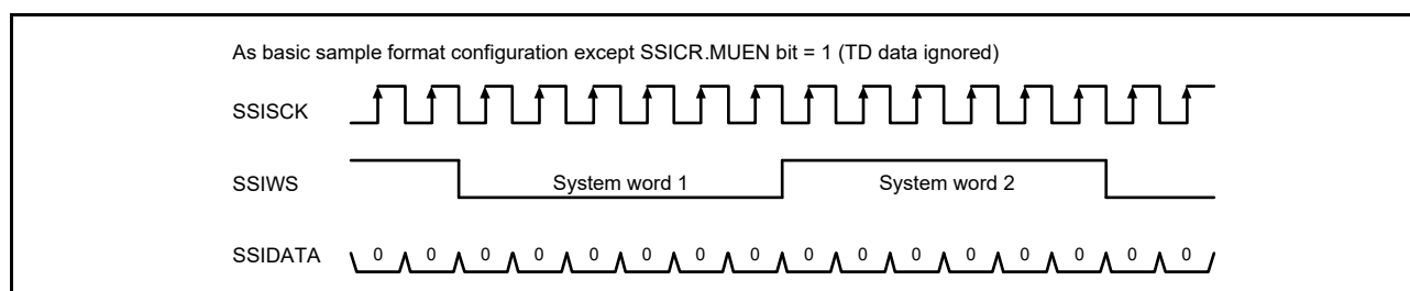
Figure 36.15 Basic format example with mute enabled
