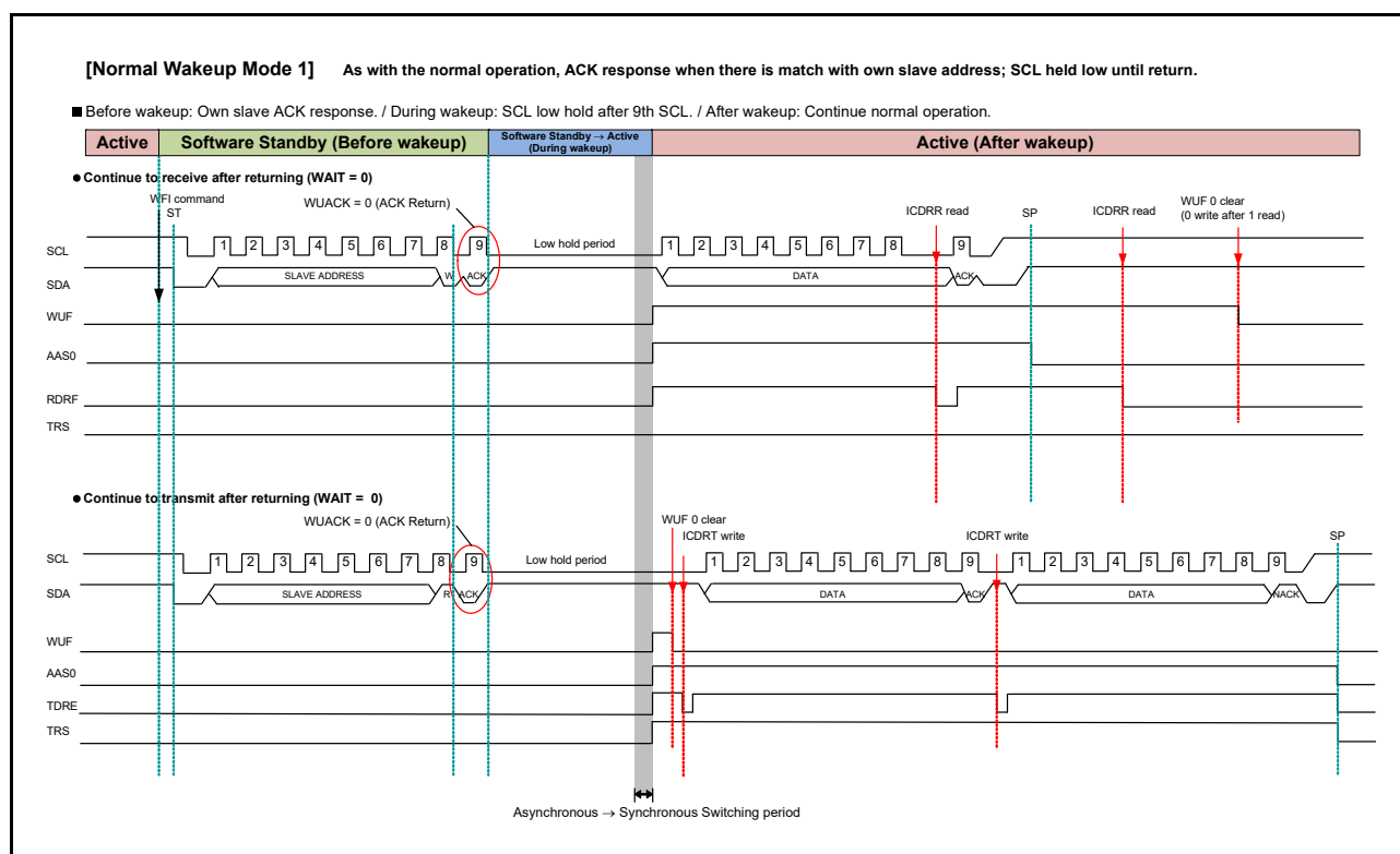
Figure 31.32 Timing of normal wakeup mode 1
