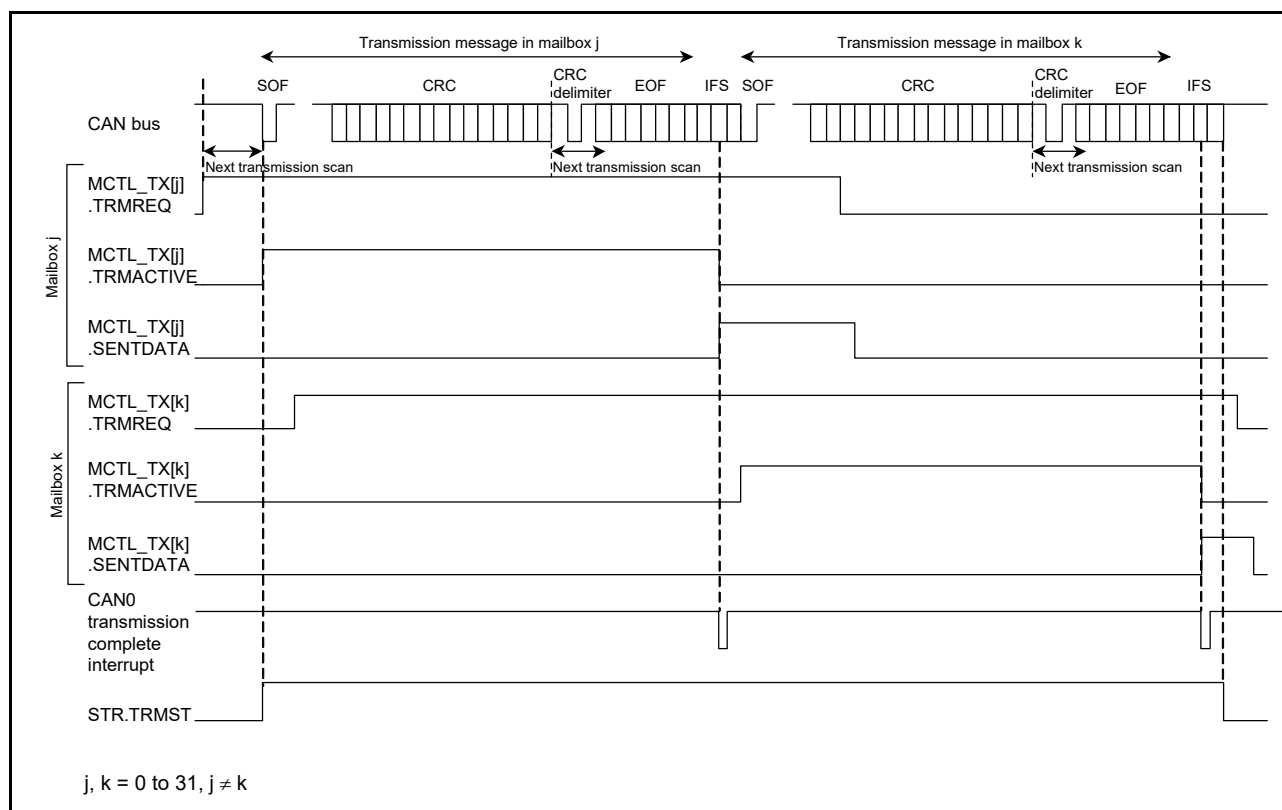
Figure 32.20 Operation example of data frame transmission
