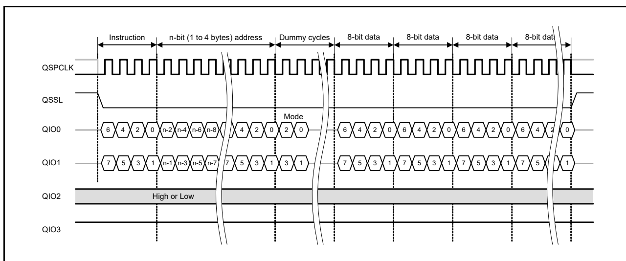
Figure 34.6 Dual SPI protocol example for Fast Read
