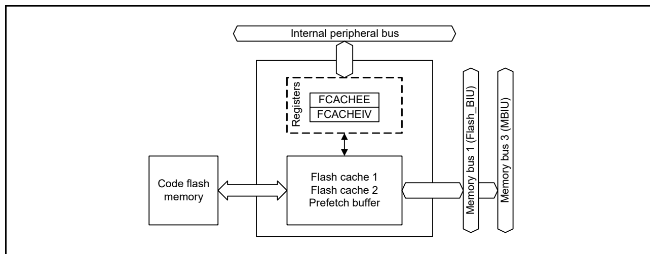
Figure 48.4 FCACHE block diagram
