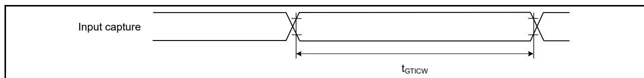
Figure 52.46 GPT input capture timing
