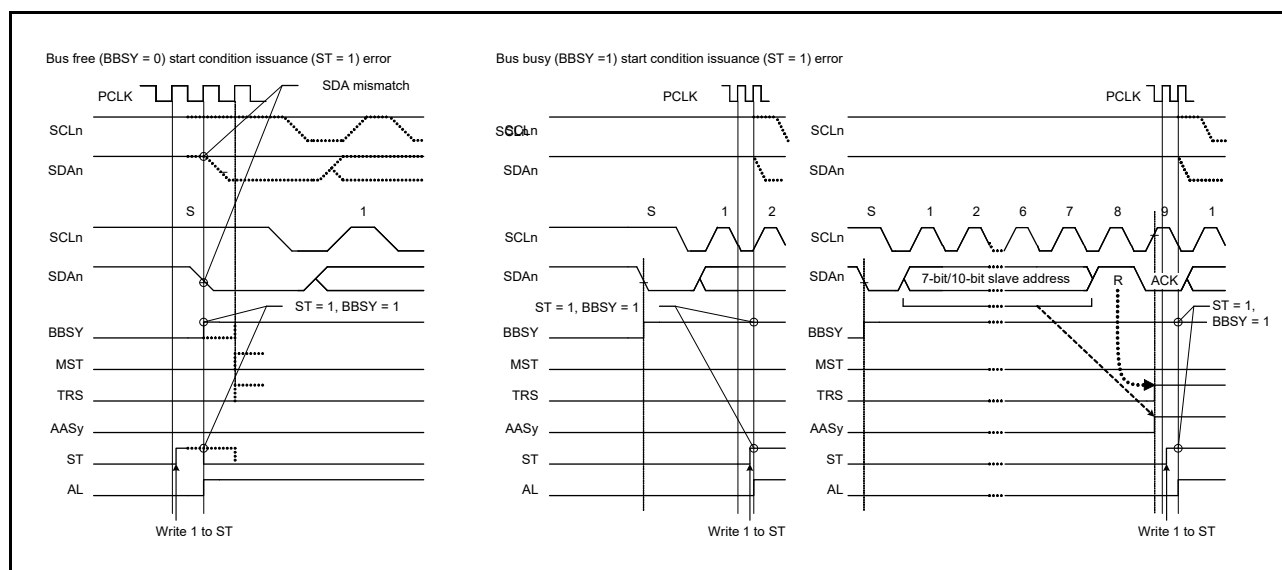
Figure 31.42 Arbitration-lost when start condition is issued (MALE = 1)
