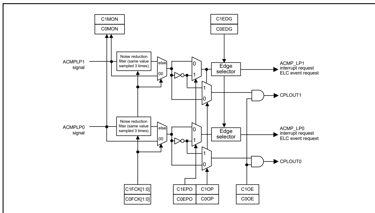
Figure 44.5 Noise filter and edge detection configuration
