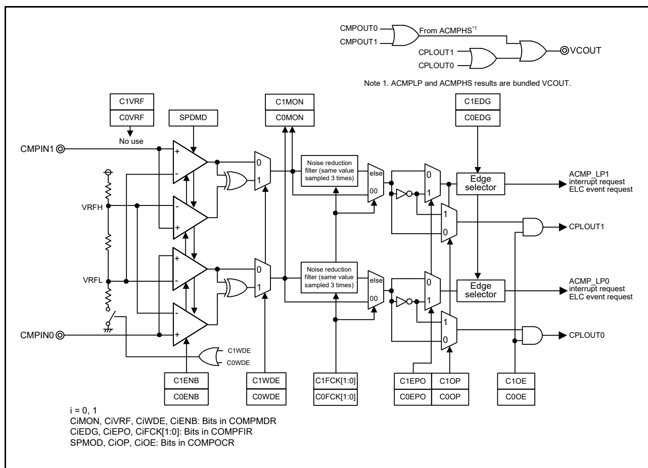
Figure 44.2 ACMPLP block diagram when window function is enabled
