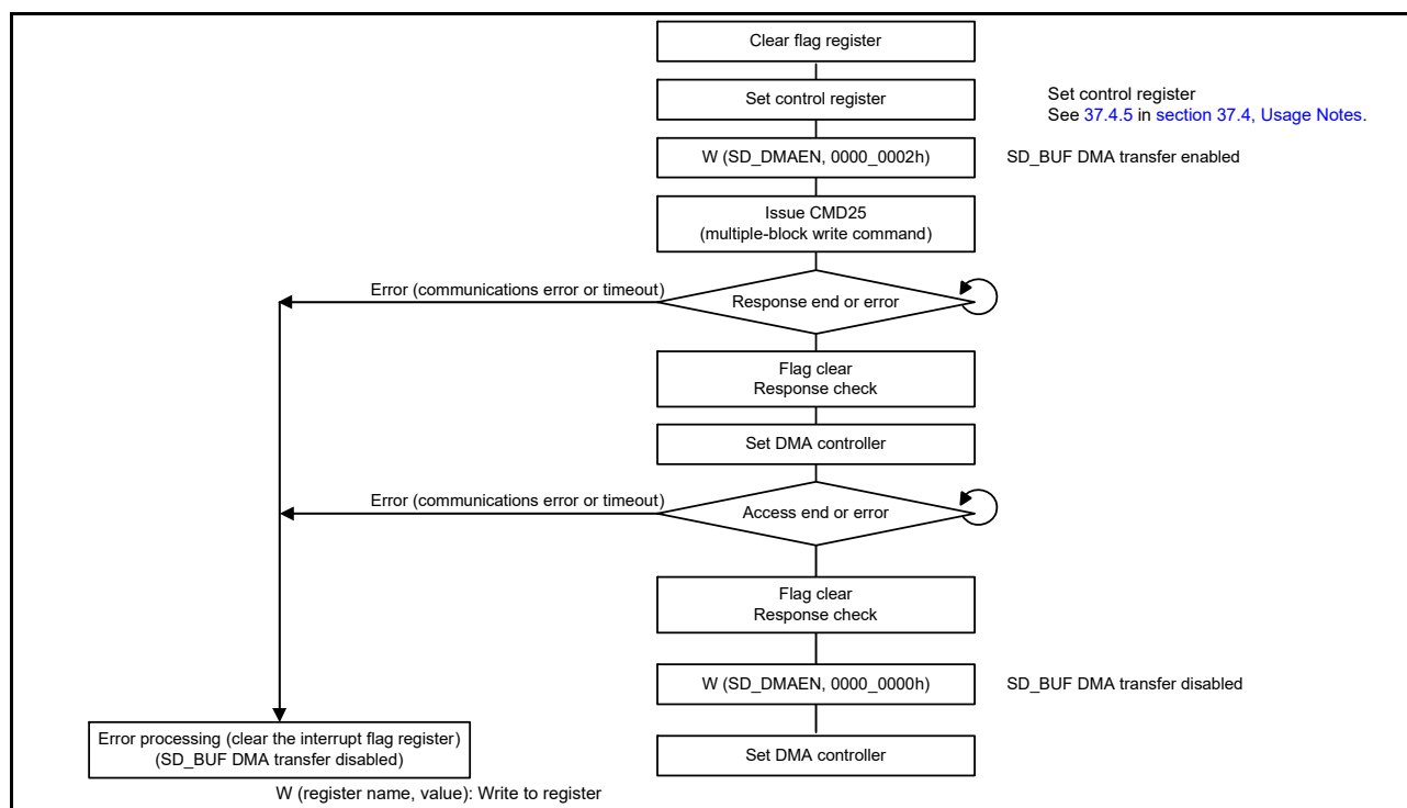
Figure 37.23 Example of SD_BUF_DMA write operation
