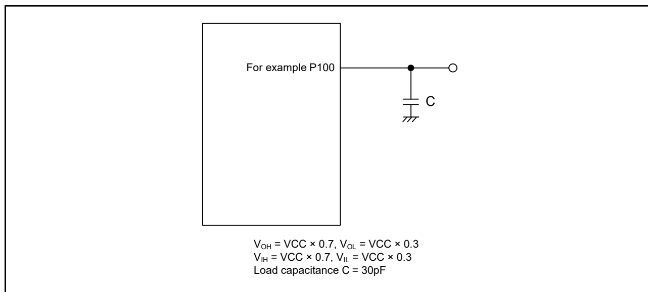
Figure 52.1 Input or output timing measurement conditions
