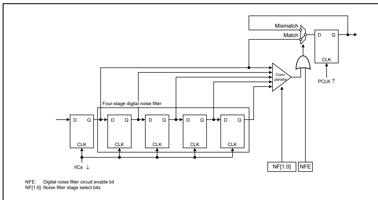
Figure 31.23 Digital noise filter circuit block diagram
