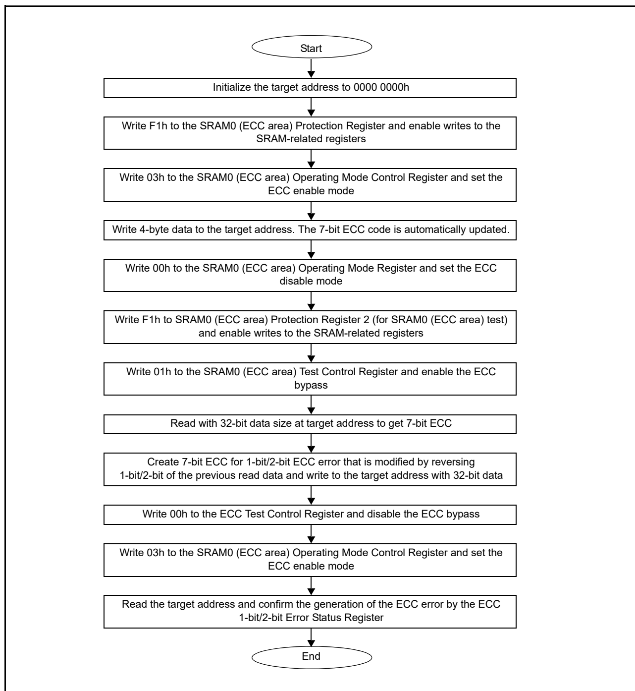
Figure 47.1 ECC decoder testing
