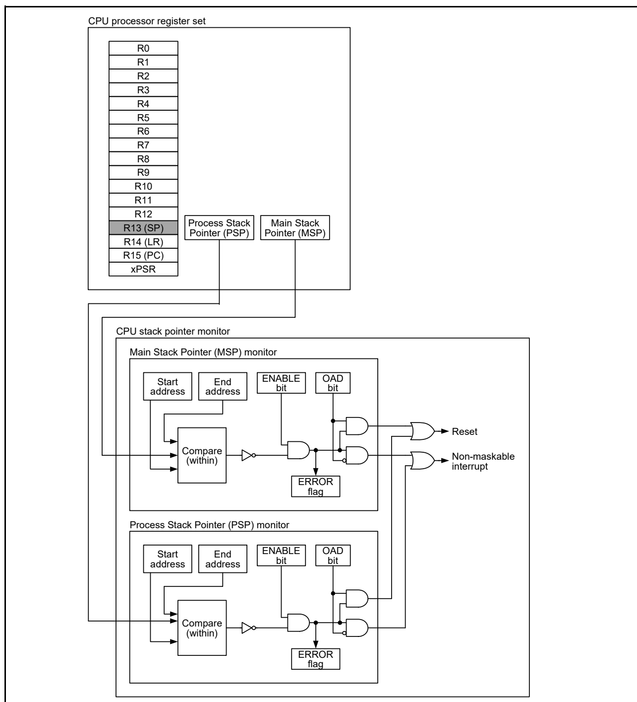
Figure 16.1 CPU stack pointer monitor block diagram
