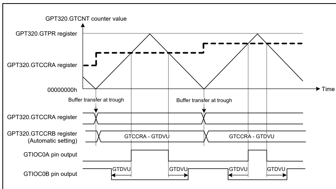
Figure 23.41 Example of automatic compare-match value setting function with dead time (triangle-wave PWM mode 1, active-high)
