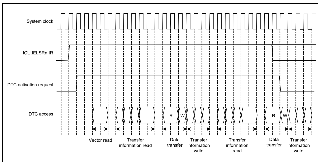
Figure 18.11 Example (3) of DTC operation timing (chain transfer)
