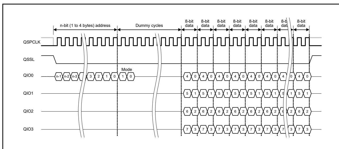
Figure 34.24 Fast read quad output bus cycle in XIP mode
