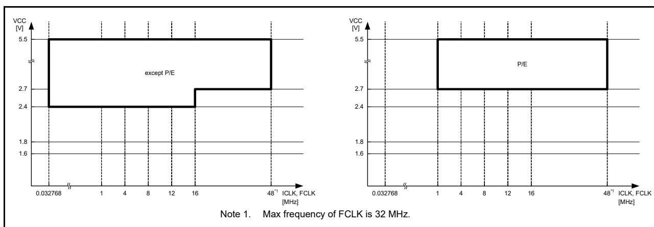
Figure 11.2 Operating voltages and frequencies in High-speed mode
