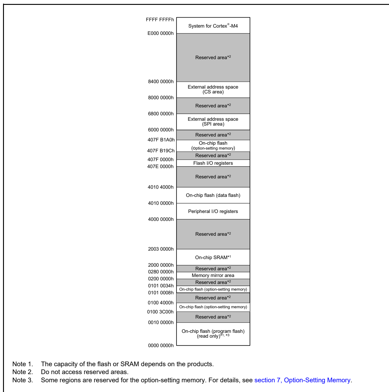
Figure 4.1 Memory map
