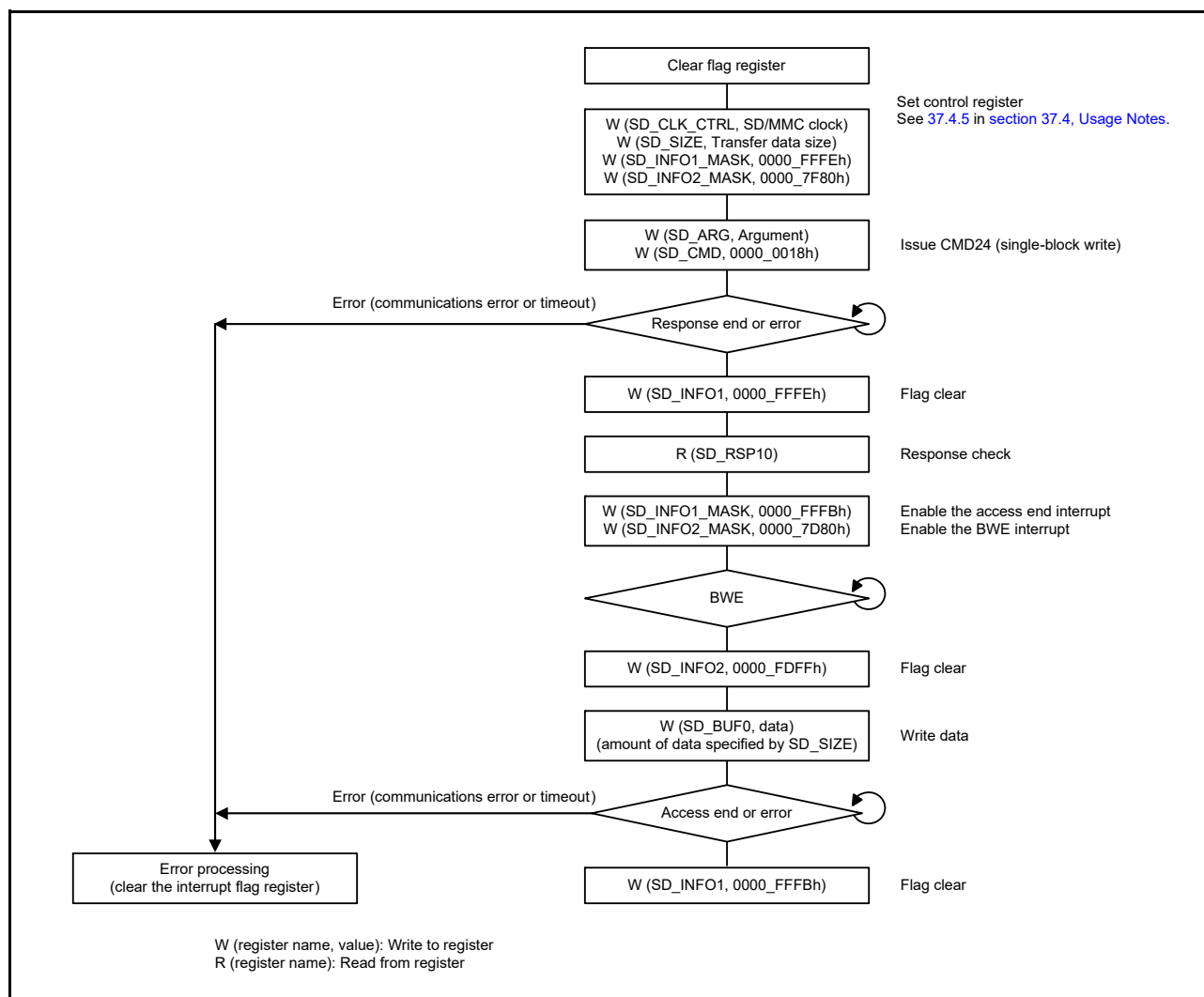
Figure 37.11 Example flow of single block write operation
