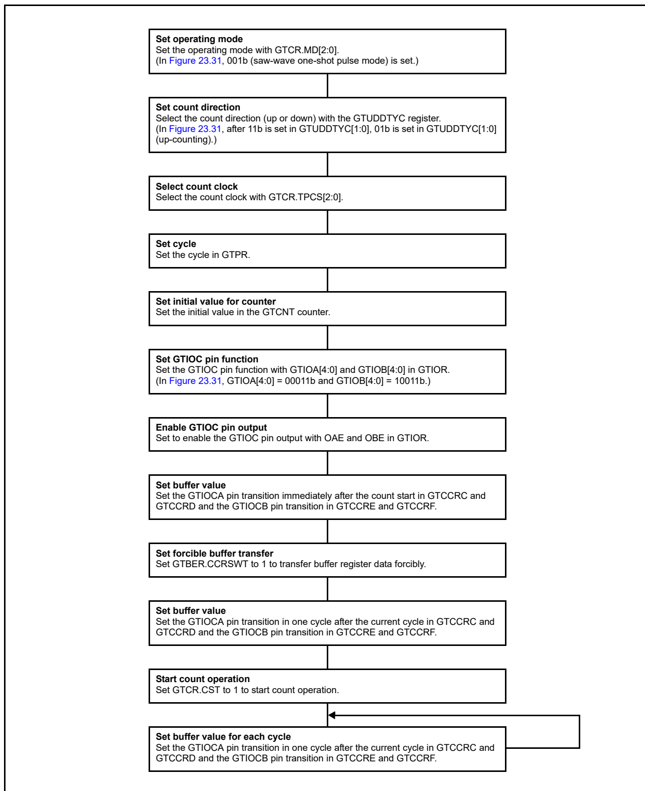
Figure 23.32 Example for setting saw-wave one-shot pulse mode
