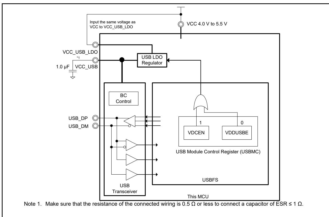
Figure 28.4 Example of power supply connection when the USB LDO regulator is used (BC not used)
