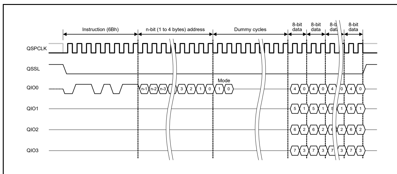
Figure 34.23 Fast read quad output bus cycle
