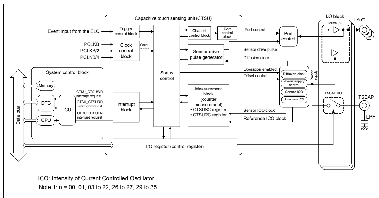
Figure 45.3 CTSU block diagram
