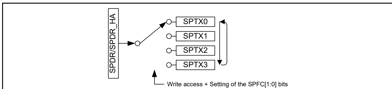
Figure 33.3 Configuration of SPDR/SPDR_HA for write access
