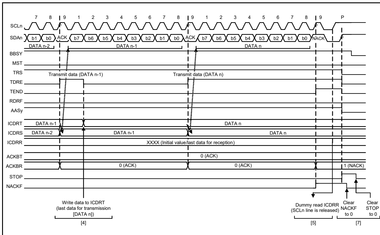
Figure 31.17 Slave transmit operation timing (2)
