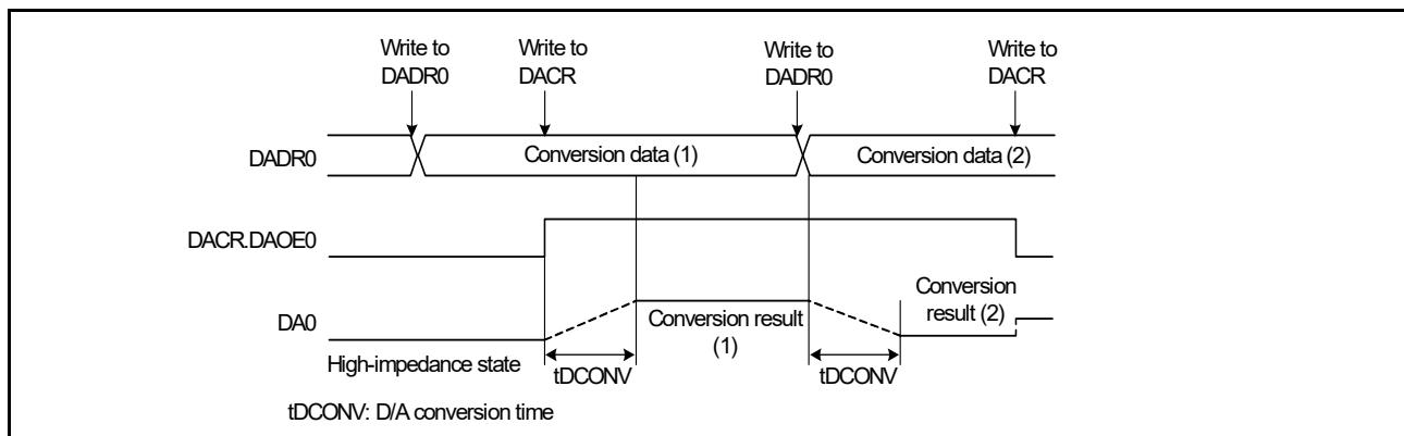
Figure 40.2 Example DAC12 operation
