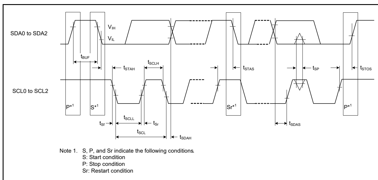
Figure 52.67 I 2 C bus interface input/output timing
