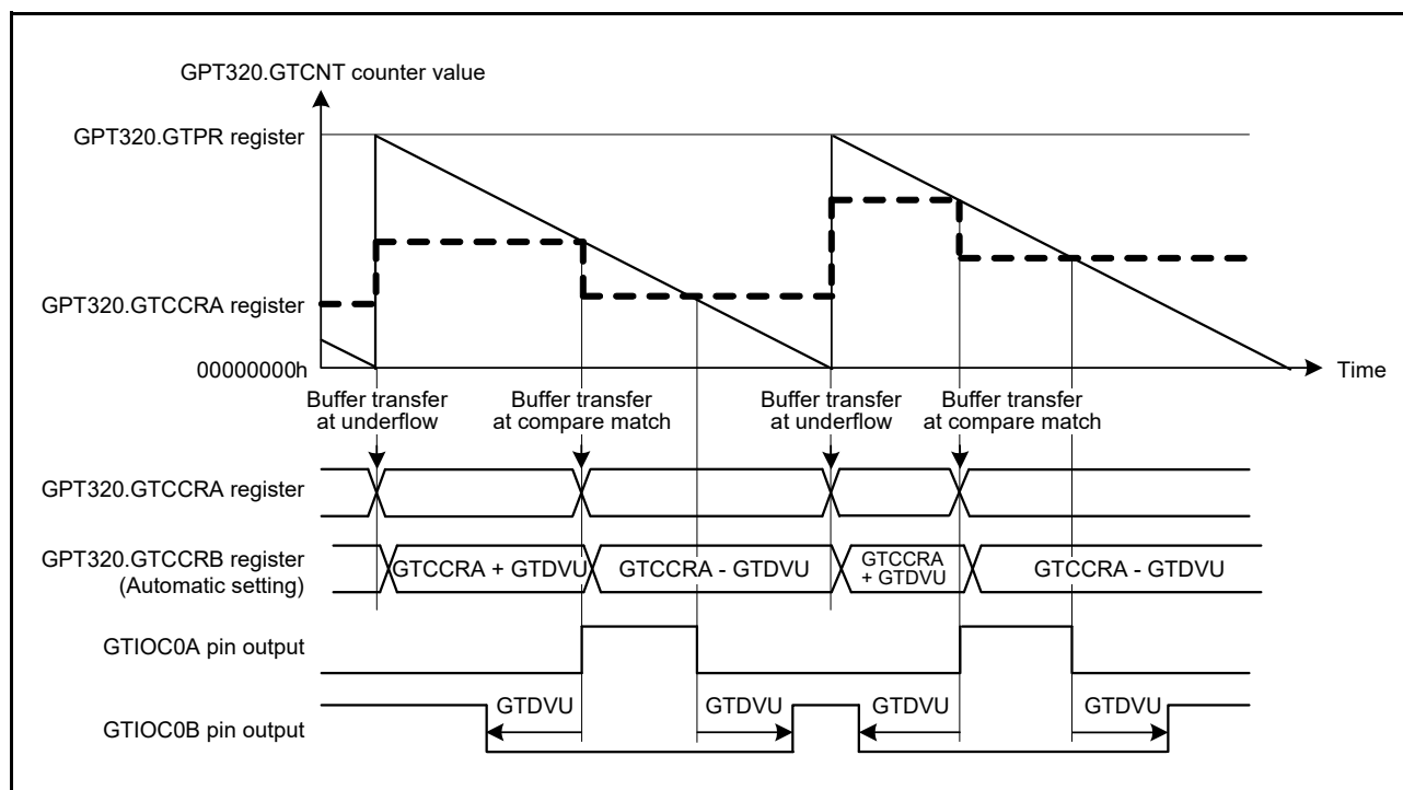
Figure 23.40 Example of automatic dead time setting function operation (saw-wave one-shot pulse mode, down-counting, active-high)
