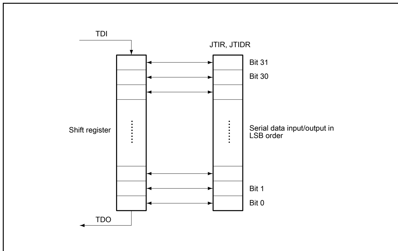
Figure 38.3 Serial data input/output
