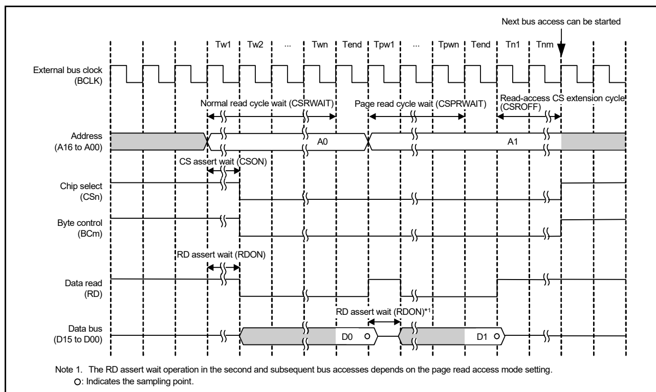
Figure 15.17 Page read access timing ( n = 0 to 3, m = 0, 1 )
