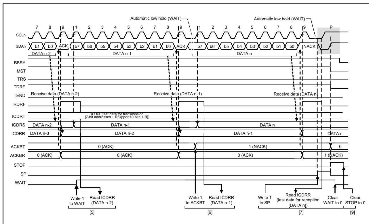
Figure 31.14 Master receive operation timing (3) when RDRFS = 0
