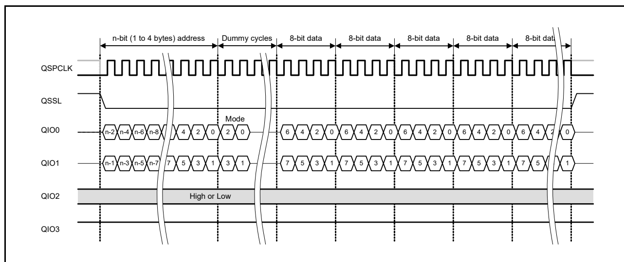
Figure 34.22 Fast read dual I/O bus cycle in XIP mode
