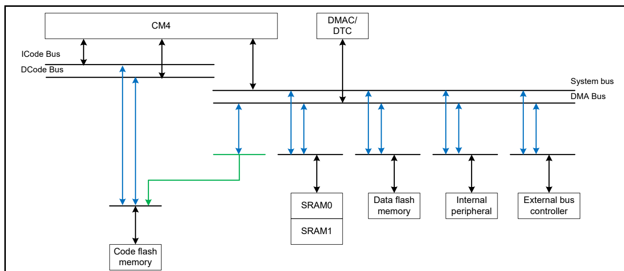
Figure 15.1 Bus configuration
