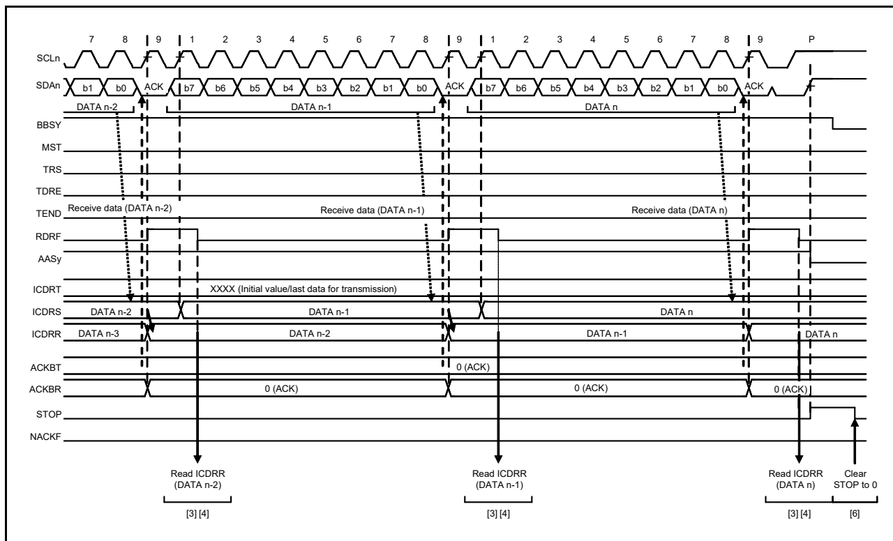
Figure 31.20 Slave receive operation timing (2) when RDRFS = 0
