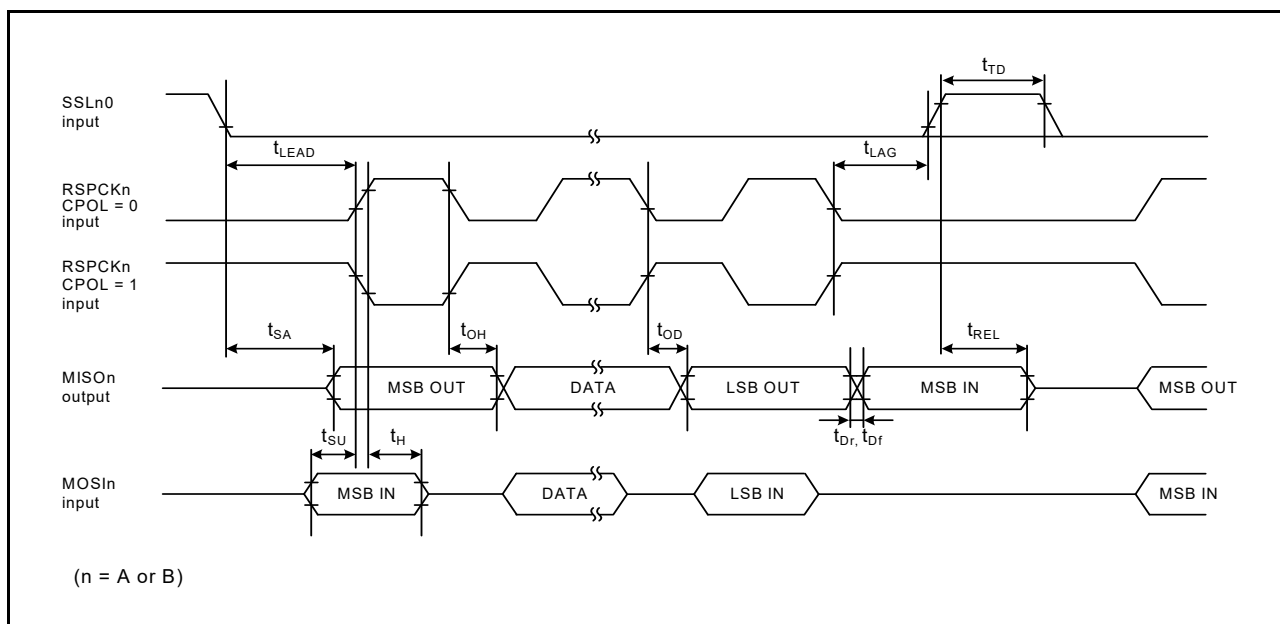
Figure 52.63 SPI timing (slave, CPHA = 0)
