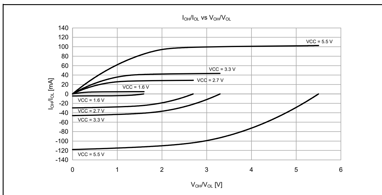
Figure 52.7 V_{OH}/V_{OL} and I_{OH}/I_{OL} voltage characteristics at T_a = 25^\circ\text{C} when middle drive output is selected (reference data)
