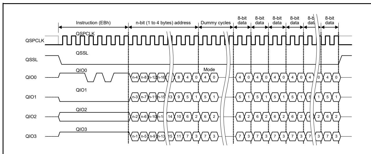
Figure 34.25 Fast read quad I/O bus cycle
