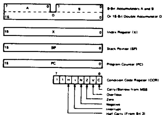
Figure 30 CPU Programming Model
