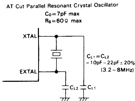
Figure 15 Connection Circuit
