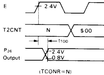
Figure 8 Timer 2 Output Timing
