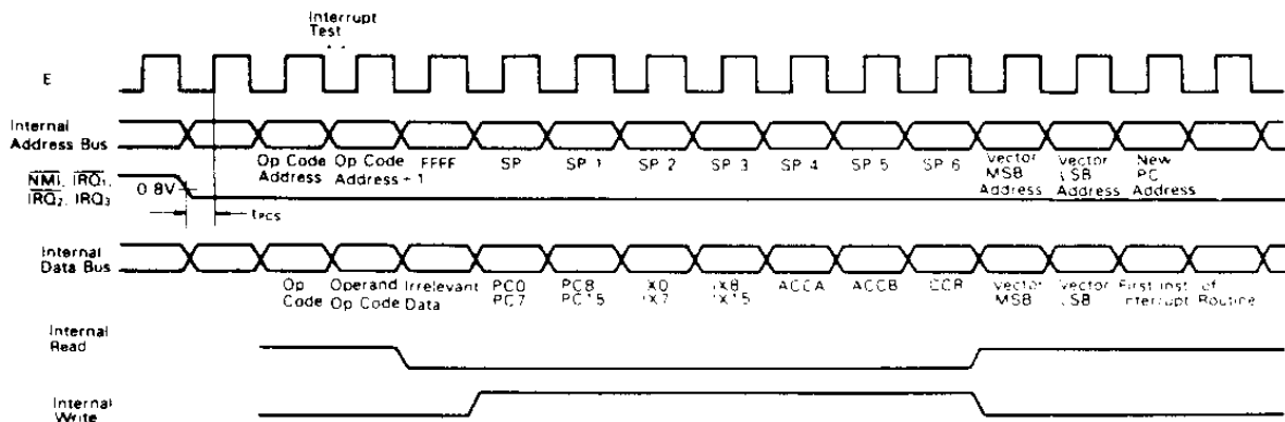
Figure 13 Interrupt Sequence
