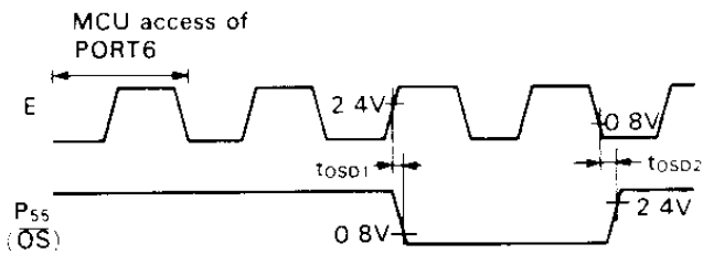
Figure 11 Output Strobe Timing
