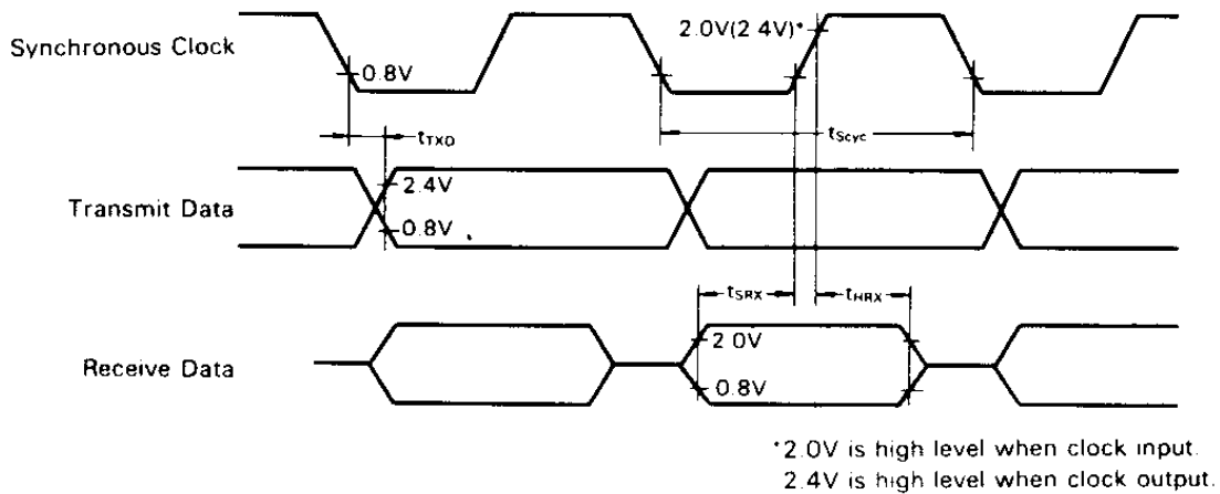
Figure 4 SCI Clocked Synchronous Timing
