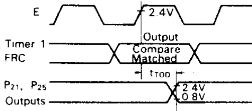
Figure 7 Timer 1 Output Timing
