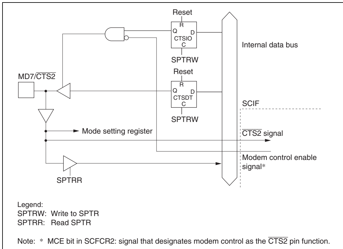
Figure 18.9 MD7/CTS2 Pin
