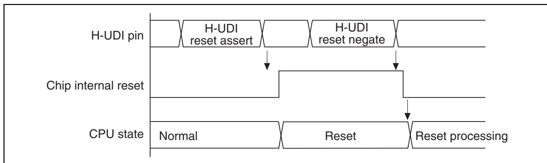
Figure 21.3 H-UDI Reset
