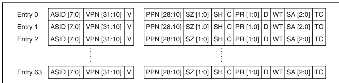
Figure 3.7 UTLB Configuration
