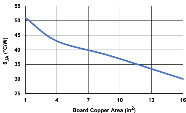
Figure 89. \theta_{JA} vs Copper Area Sizes (SOIC)
