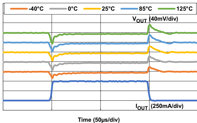
Figure 3. Load Transient Response for Various Junction Temperatures ( V_{IN} = 2.5V , V_{OUT} = V_{ADJ} , C_{OUT} = 4.7\mu F , C_{FF} = \text{None} , \Delta I_{OUT} = 1mA to 500mA at 100mA/\mu s )
