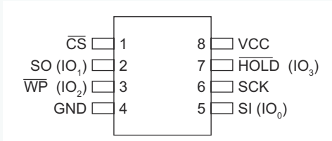
Figure 2-1. 8-SOIC (0.208”) — Top View
