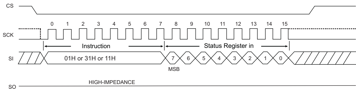
Figure 11-3. Write Status Register
