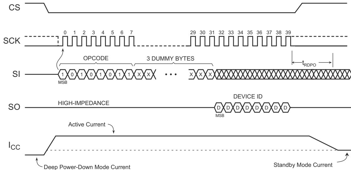
Figure 12-7. Resume from Deep Power-Down and Read Device ID
