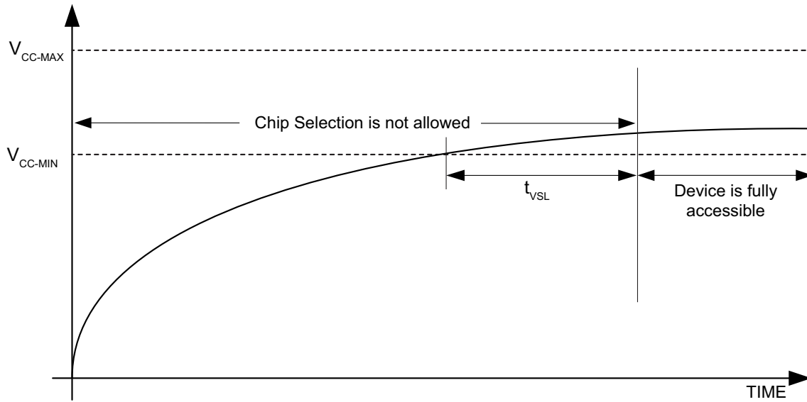
Figure 13-1. Power-up Timing and Voltage Levels
