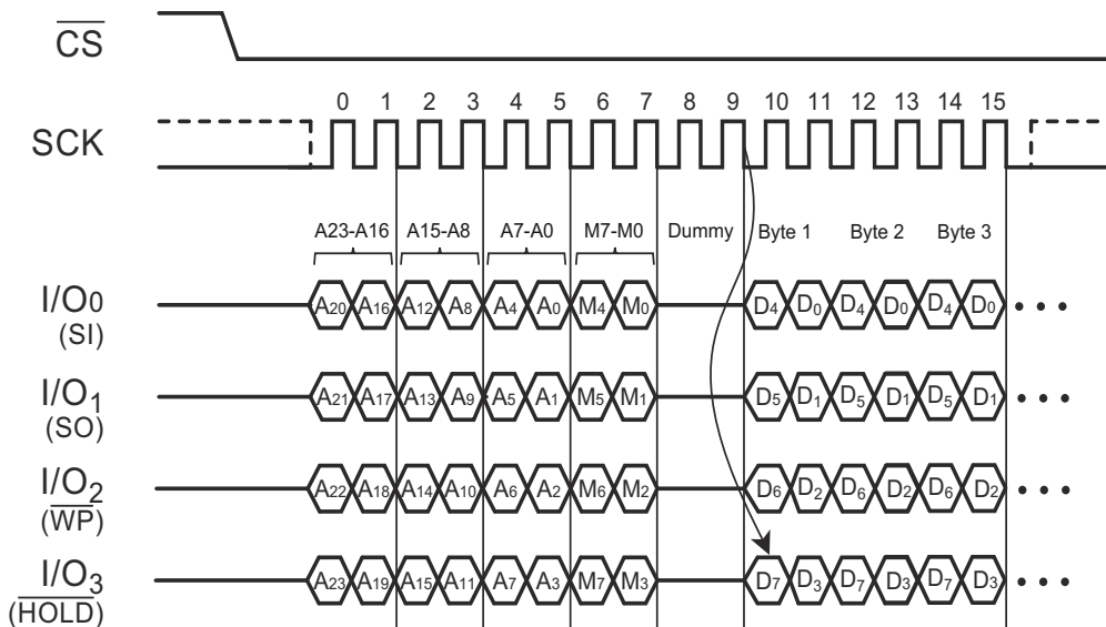
Figure 7-11. Quad-I/O Word Fast Read Timing (Previous Command Set M5, M4 = 1,0) SPI Mode
