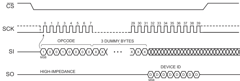
Figure 12-2. Read Manufacture ID and Device (Legacy Command)
