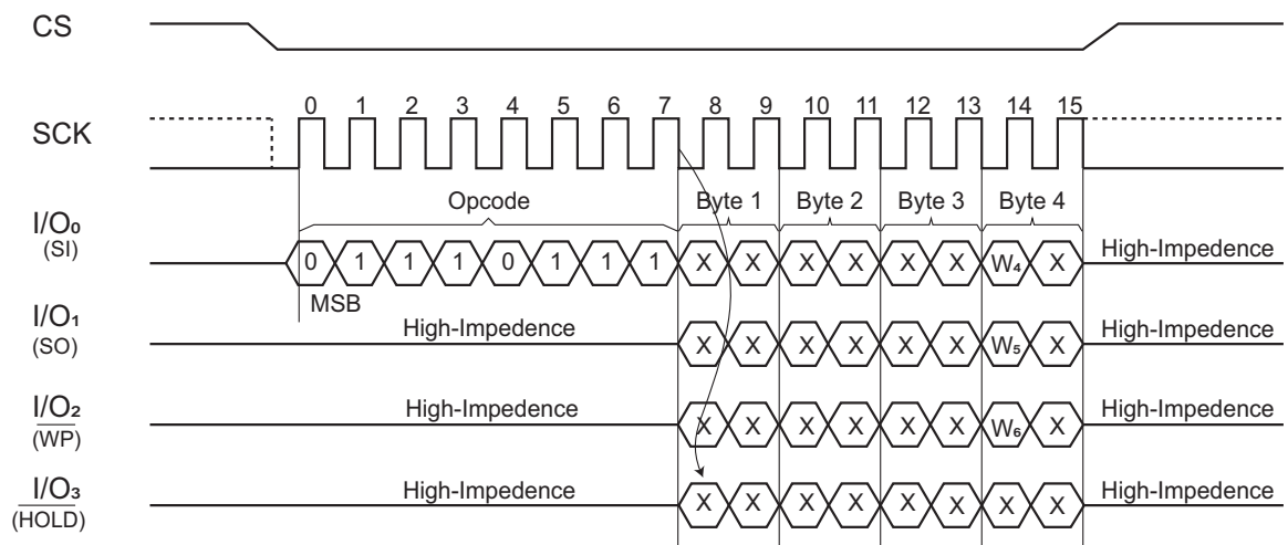
Figure 7-9. Set Burst with Wrap Timing (SPI Mode)
