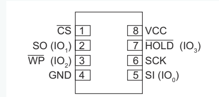
Figure 2-2. 8-UDFN — Top View
