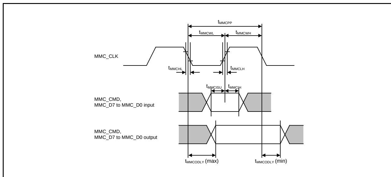
Figure 2.70 MMC Interface
