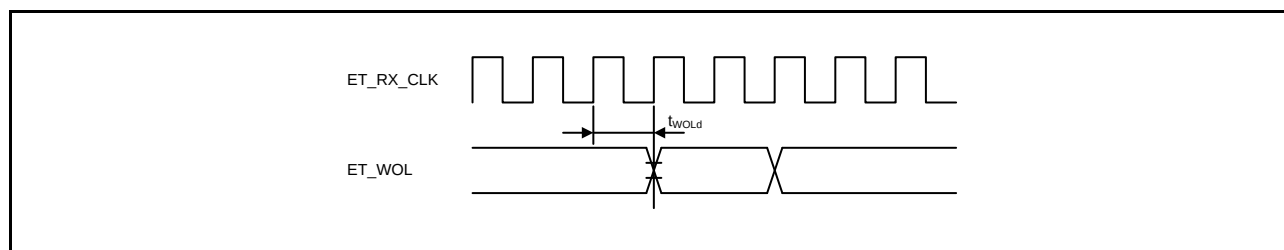
Figure 2.81 WOL Output Timing (MII)
