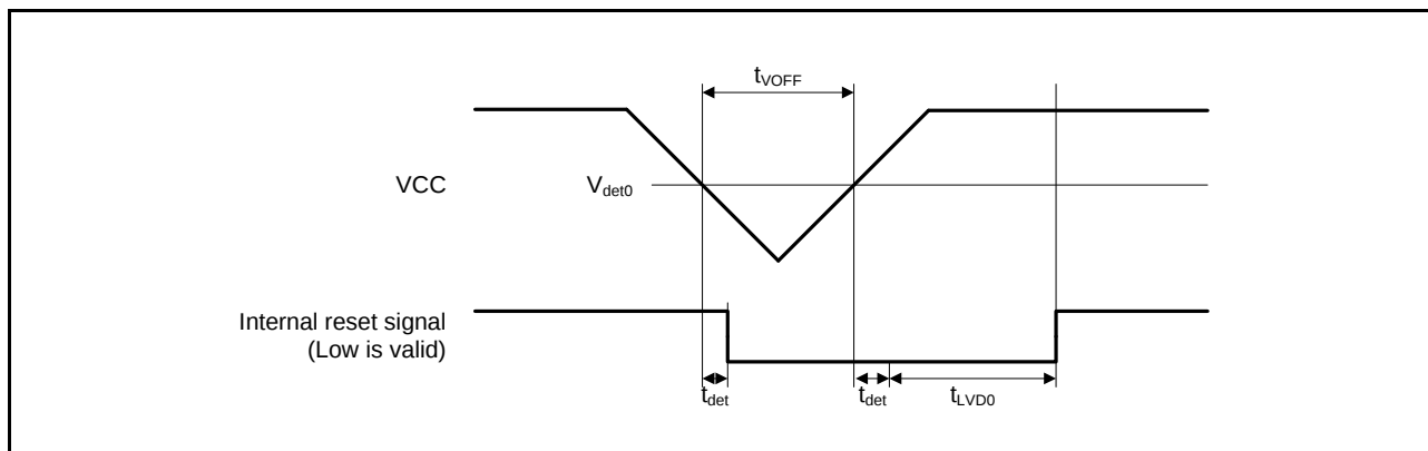
Figure 2.95 Voltage Detection Circuit Timing ( V_{det0} )
