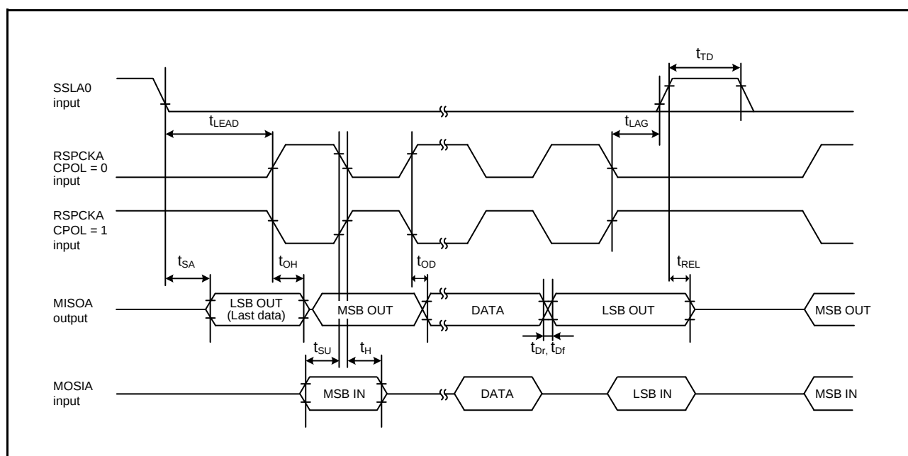
Figure 2.62 RSPI Timing (Slave, CPHA = 1)
