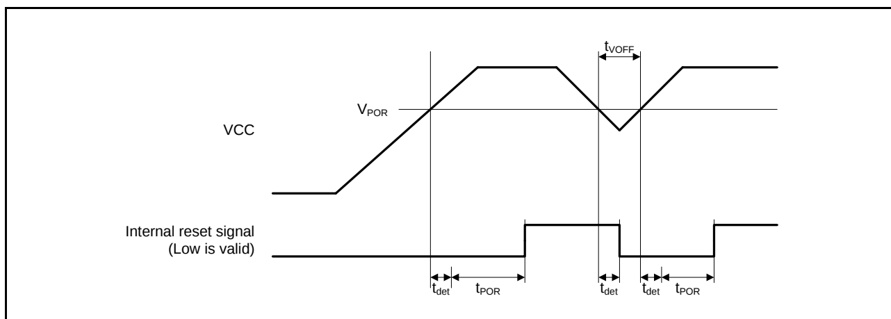
Figure 2.94 Power-on Reset Timing
