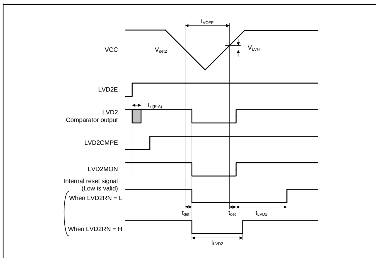
Figure 2.97 Voltage Detection Circuit Timing (V det2 )
