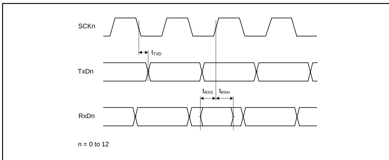
Figure 2.48 SCI Input/Output Timing: Clock Synchronous Mode
