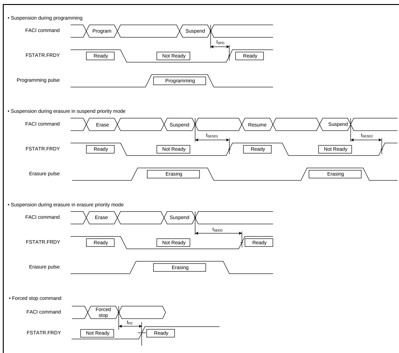
Figure 2.100 Flash Memory Programming/Erasure Suspension Timing
