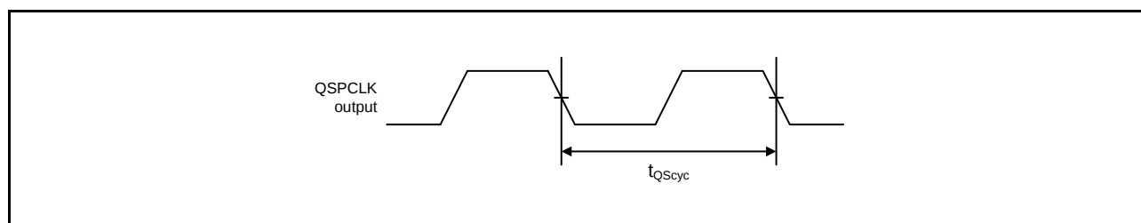
Figure 2.63 QSPI Clock Timing
