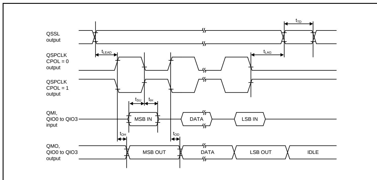
Figure 2.65 Transmit/Receive Timing (CPHA = 1)
