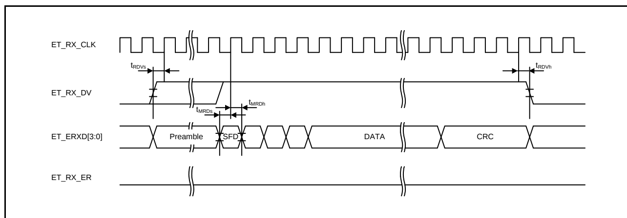
Figure 2.79 MII Reception Timing (Normal Operation)
