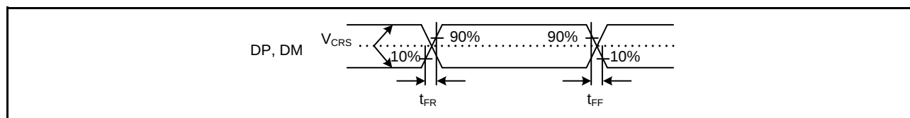
Figure 2.88 DP and DM Output Timing (Full-Speed)
