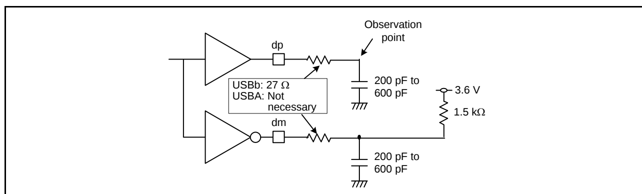
Figure 2.87 Test Circuit (Low Speed)
