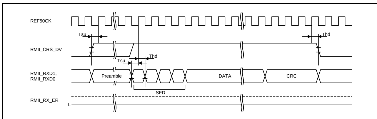
Figure 2.74 RMII Reception Timing (Normal Operation)
