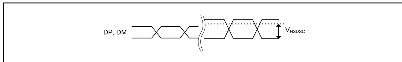
Figure 2.91 DP and DM Disconnect detect sensitivity (High-Speed)
