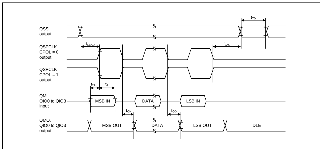
Figure 2.64 Transmit/Receive Timing (CPHA = 0)
