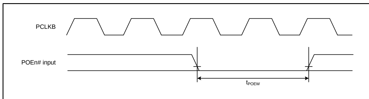
Figure 2.40 POE# Input Timing
