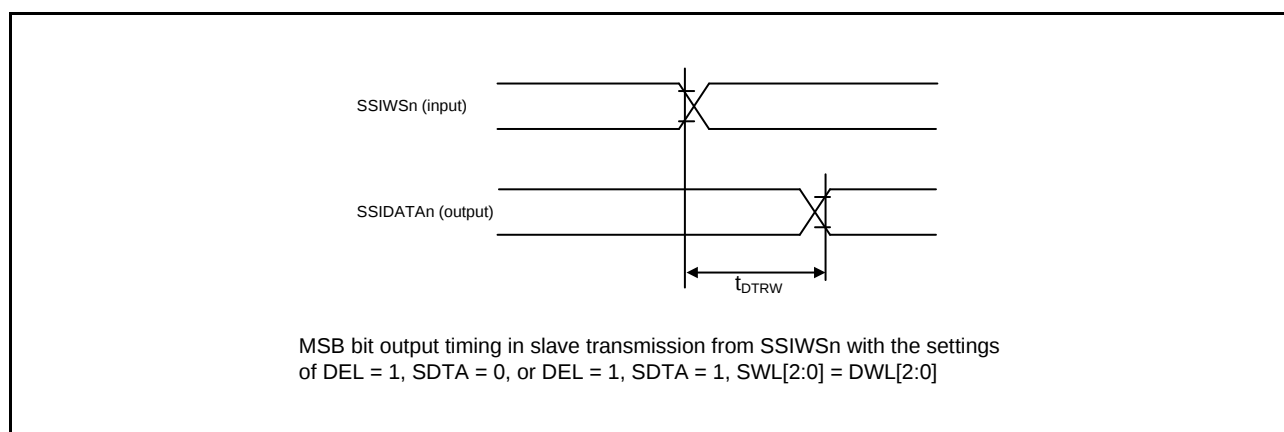
Figure 2.69 SSIDATA Output Delay from SSIWSn Change Edge
