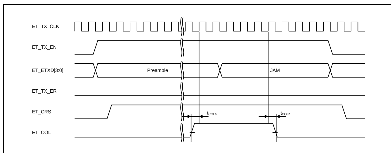
Figure 2.78 MII Transmission Timing (Conflict Occurrence)
