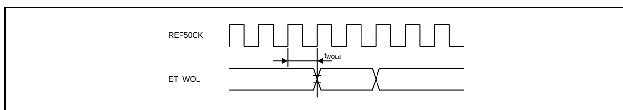
Figure 2.76 WOL Output Timing (RMII)
