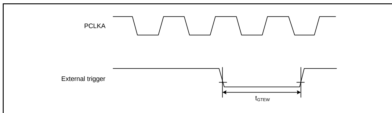
Figure 2.46 GPT External Trigger Input Timing
