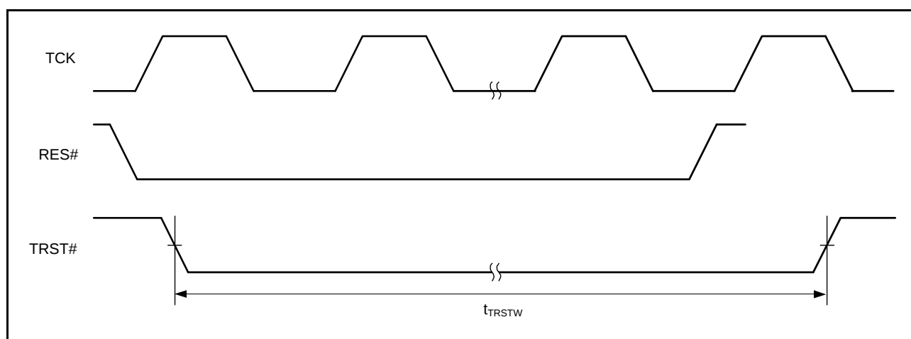
Figure 2.102 Boundary Scan TRST# Timing
