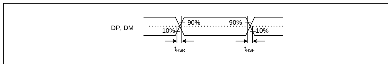
Figure 2.92 DP and DM Output Timing (High-Speed)
