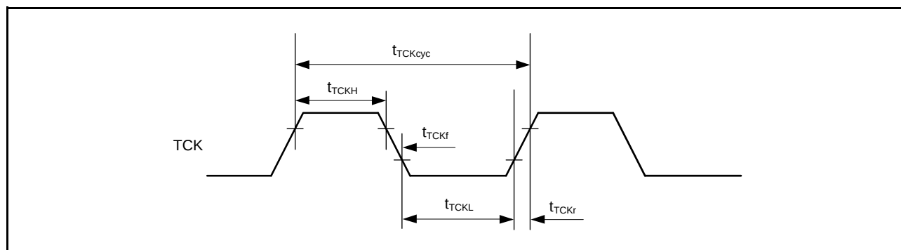
Figure 2.101 Boundary Scan TCK Timing
