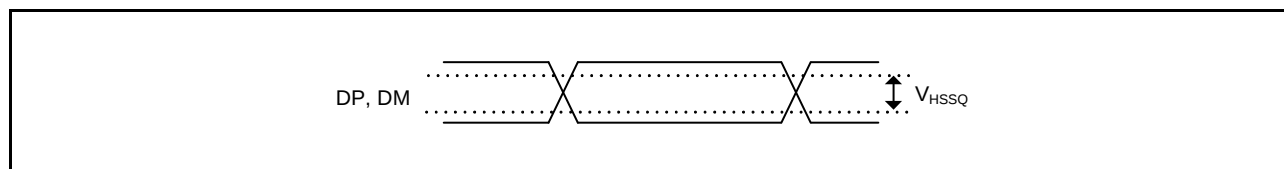
Figure 2.90 DP and DM Squelch detect sensitivity (High-Speed)
