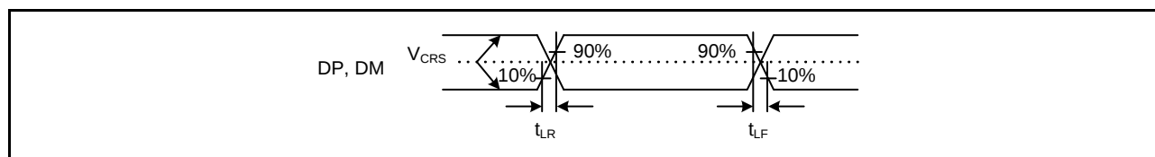
Figure 2.86 DP and DM Output Timing (Low Speed)
