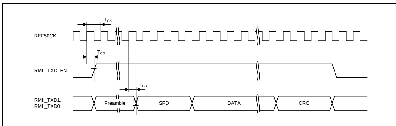
Figure 2.73 RMII Transmission Timing
