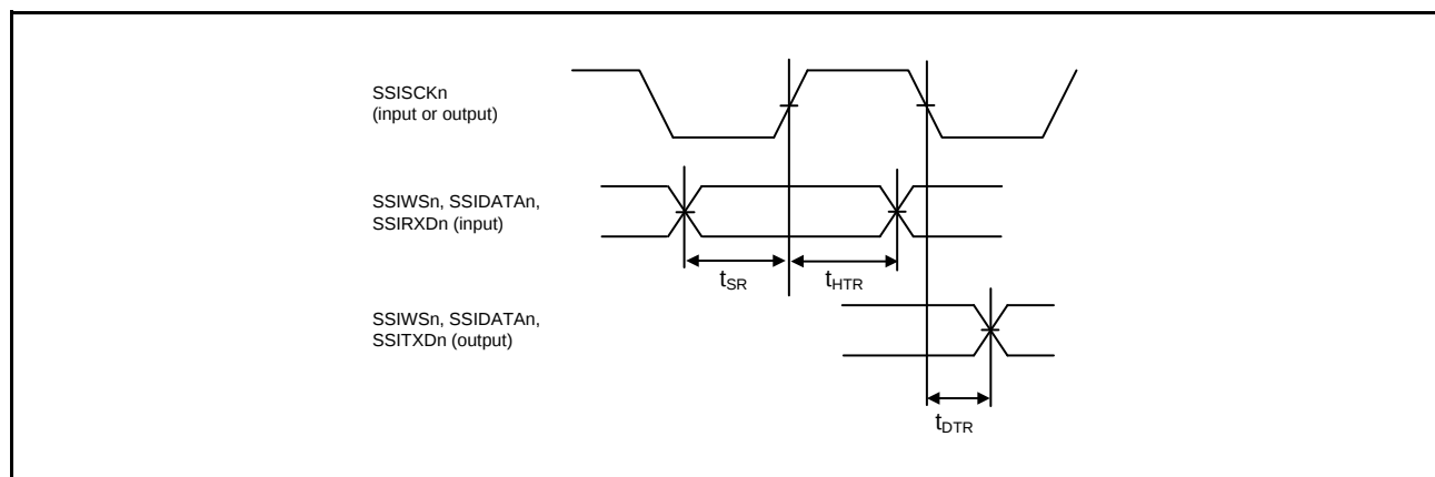
Figure 2.67 Transmit/Receive Timing (SSISCKn Rising Synchronous)
