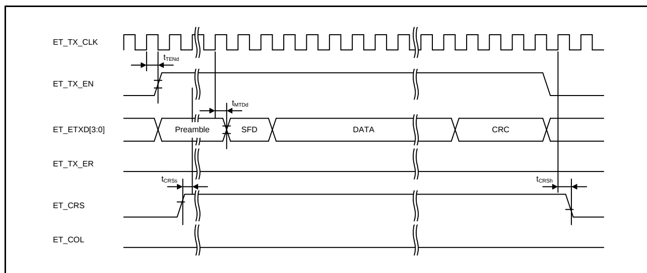
Figure 2.77 MII Transmission Timing (Normal Operation)
