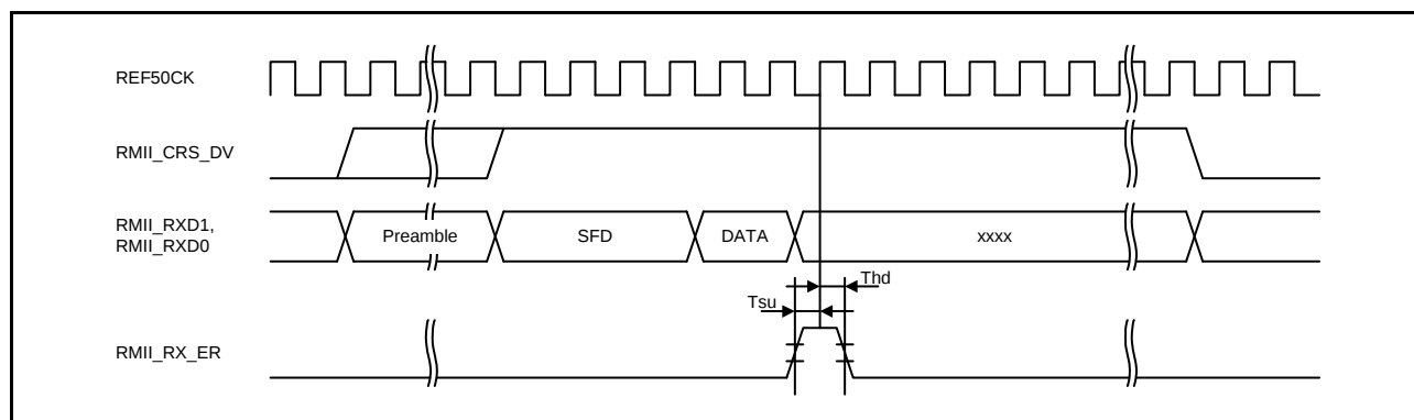
Figure 2.75 RMII Reception Timing (Error Occurrence)
