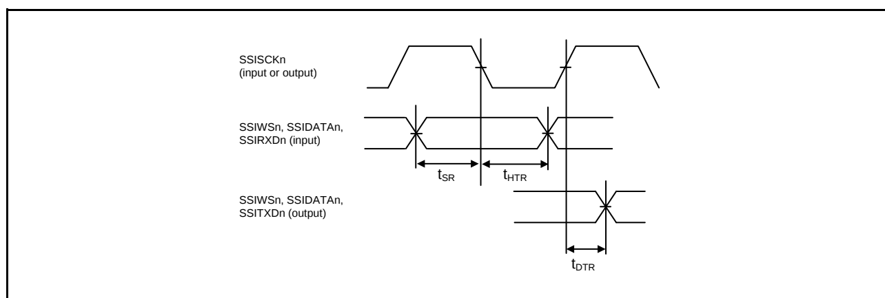
Figure 2.68 Transmit/Receive Timing (SSISCKn Falling Synchronous)
