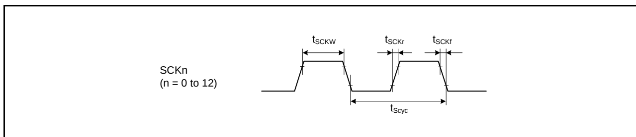
Figure 2.47 SCK Clock Input Timing
