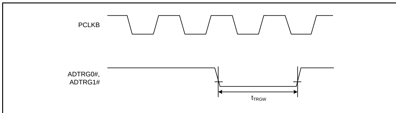
Figure 2.85 A/D Converter Trigger Input Timing
