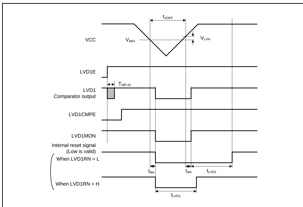
Figure 2.96 Voltage Detection Circuit Timing (V det1 )
