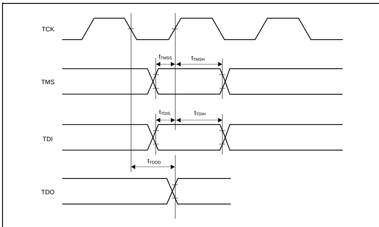
Figure 2.103 Boundary Scan Input/Output Timing
