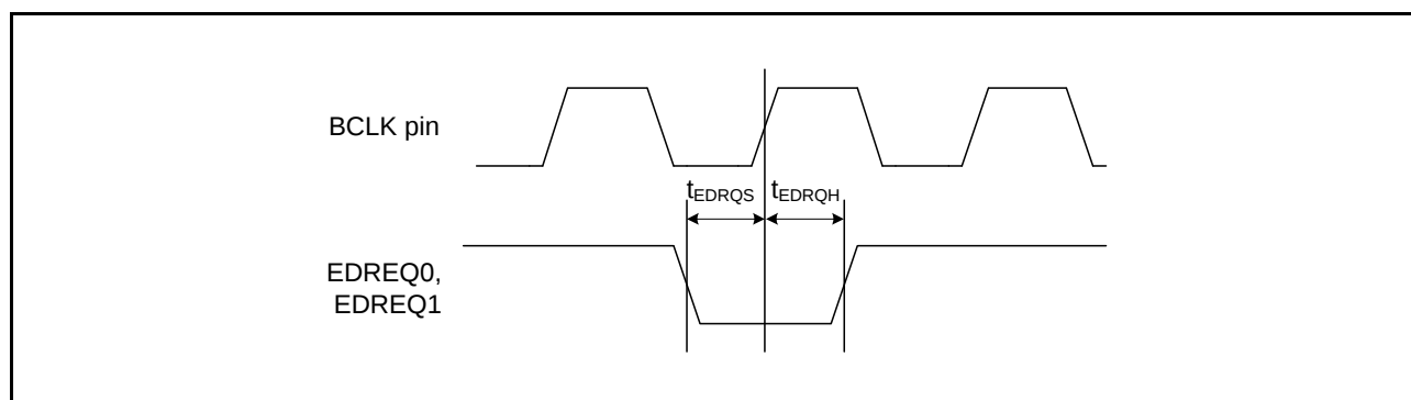
Figure 2.30 EDREQ0 and EDREQ1 Input Timing
