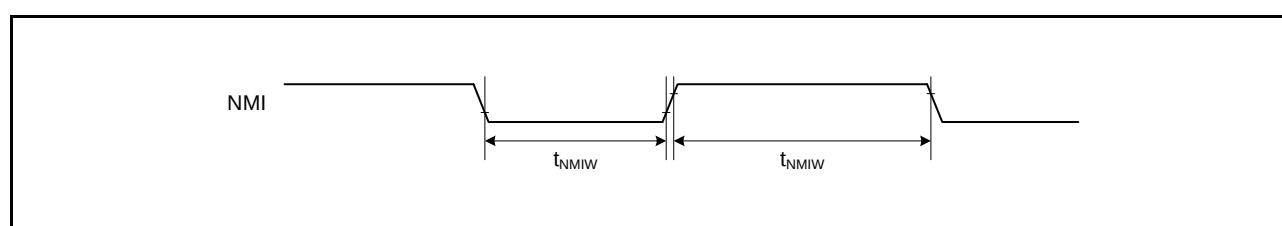
Figure 2.14 NMI Interrupt Input Timing
