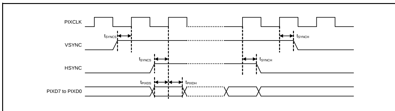
Figure 2.84 PDC AC Timing
