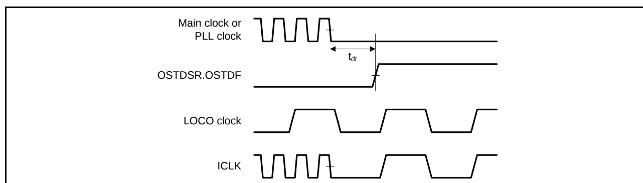
Figure 2.98 Oscillation Stop Detection Timing
