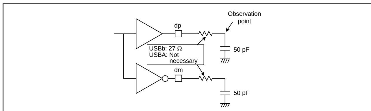
Figure 2.89 Test Circuit (Full-Speed)
