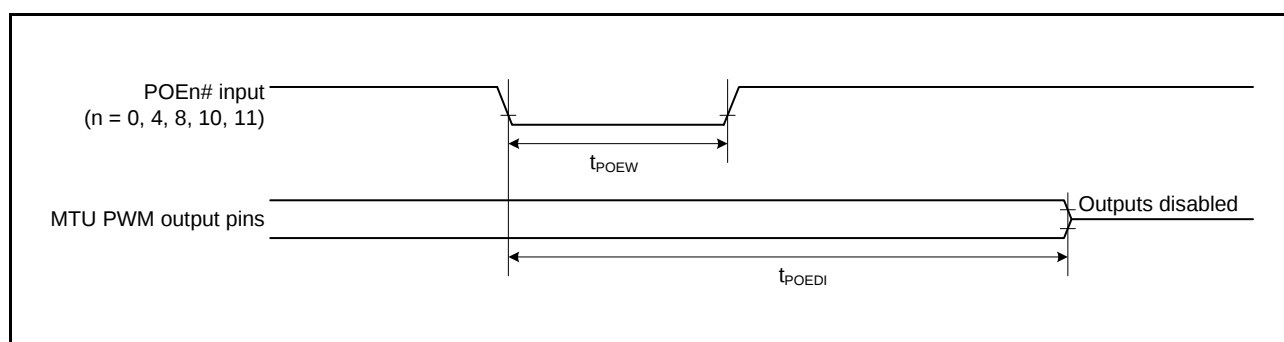
Figure 2.41 Output Disable Time for POE in Response to Transition of the POEn# Signal Level
