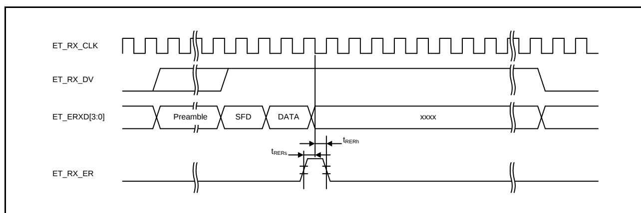
Figure 2.80 MII Reception Timing (Error Occurrence)
