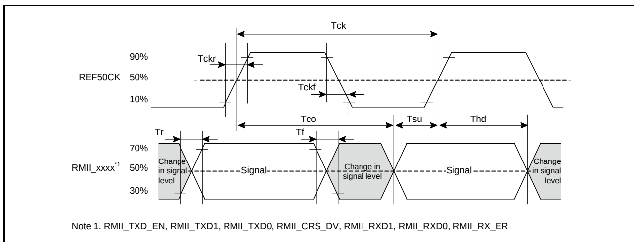
Figure 2.72 Timing with the REF50CK and RMII Signals
