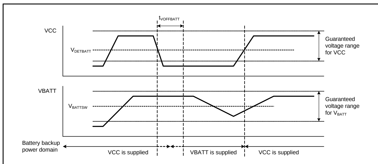
Figure 2.99 Battery Backup Function Characteristics
