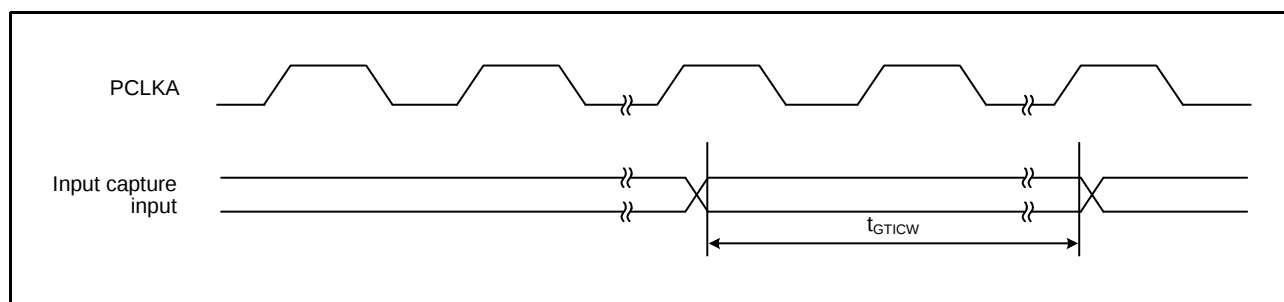
Figure 2.45 GPT Input Capture Input Timing
