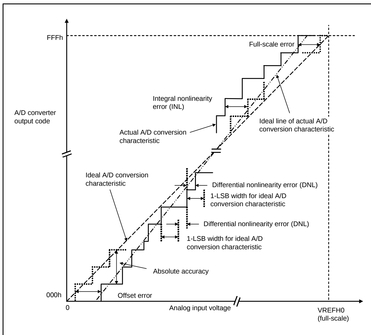
Figure 5.37 Illustration of A/D Converter Characteristic Terms
