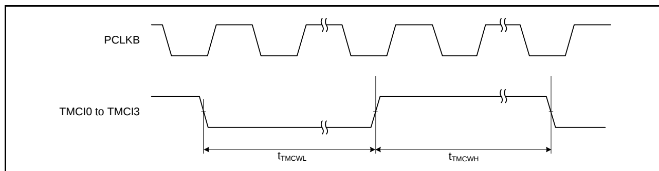
Figure 5.24 8-Bit Timer Clock Input Timing
