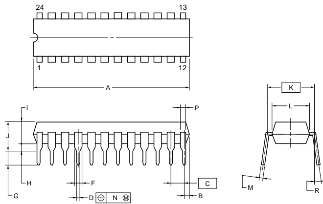
24PIN PLASTIC DIP (300 mil)
