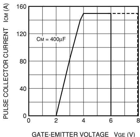
Figure1. MAXIMUM PULSE COLLECTOR CURRENT
