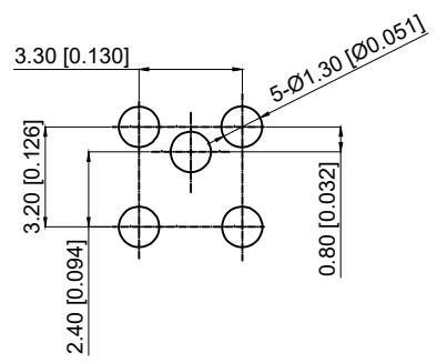
PCB board installation size PCB板安装尺寸
