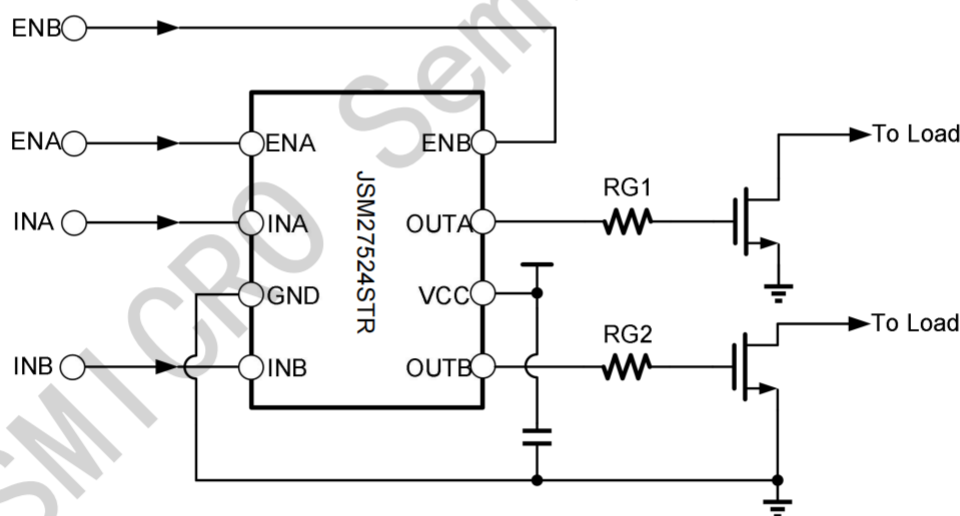
Figure 20 Inverting Typical Application Diagram of JSM27524
