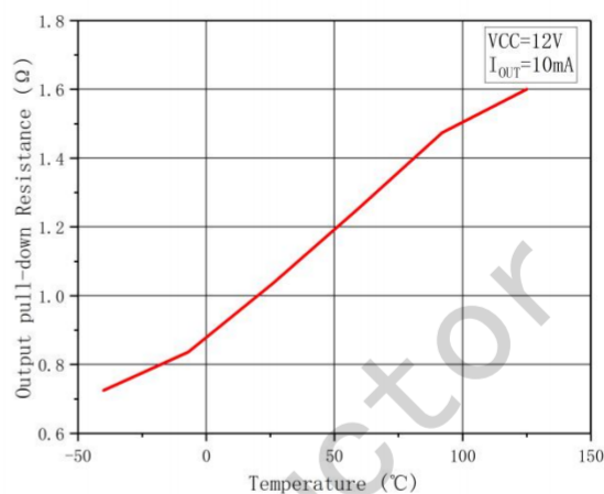
Figure 10. Output Pull-down Resistance vs Temperature
