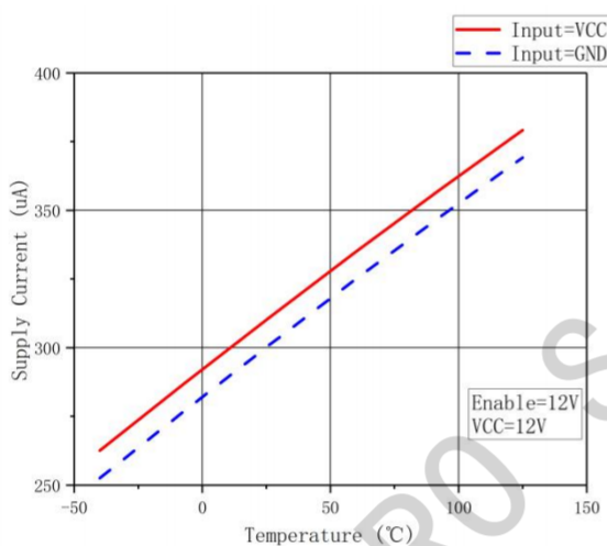
Figure 5. Supply Current vs Temperature (Outputs In DC On/Off Condition)
