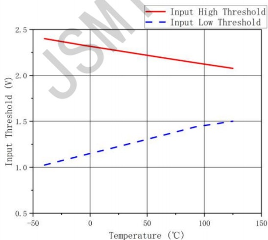
Figure 7. Input Threshold vs Temperature
