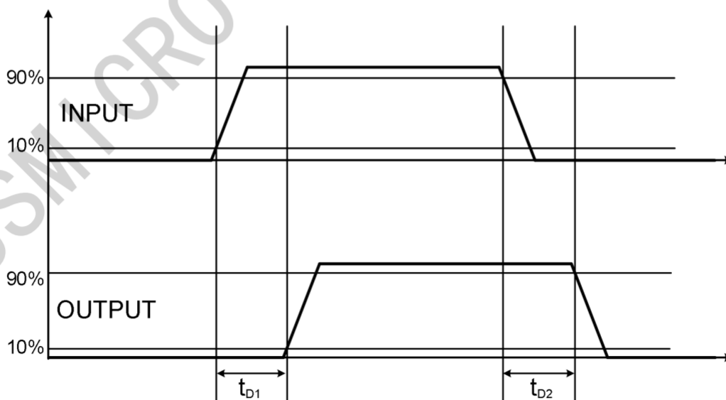
Figure 1 Input-Output waveform(non-inverting)
