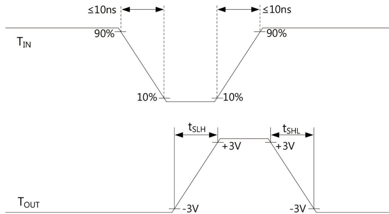
Figure 3. t_{\text{SLH}} and t_{\text{SHL}} waveforms of Transmitter
