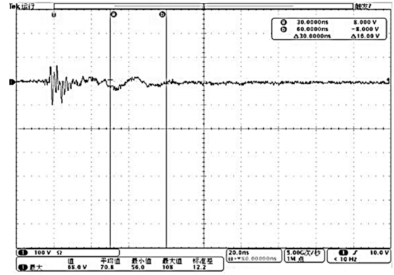
Fig 8. Clamping Voltage at IEC61000-4-2 -8kV Pulse Waveform
