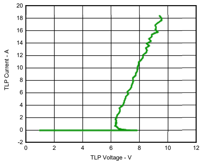
Fig 6. TLP Measurement
