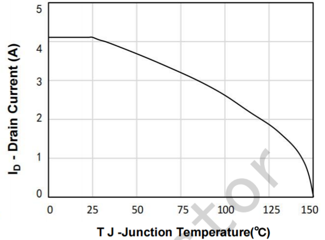
Figure 8. Maximum Continuous Drain Current vs Temperature
