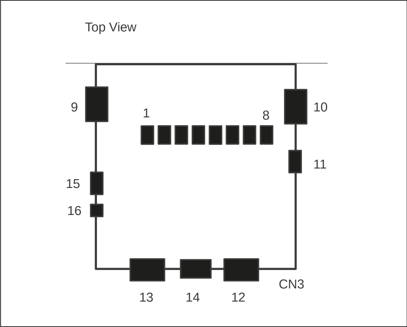
Figure 3.3 microSD Card Slot (CN3) Pin Layout Diagram
