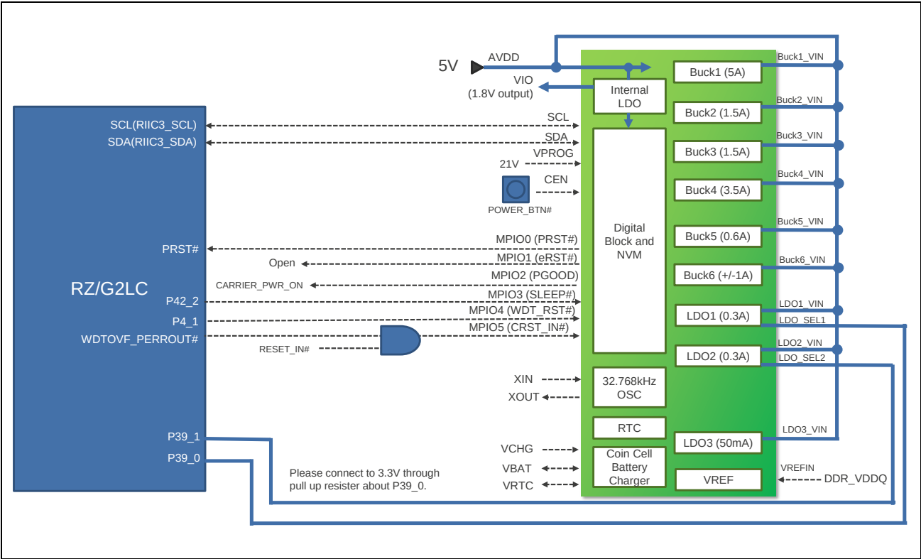
Figure 2.8 Block Diagram around PMIC
