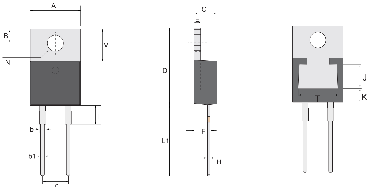
TO-220AC mechanical data
