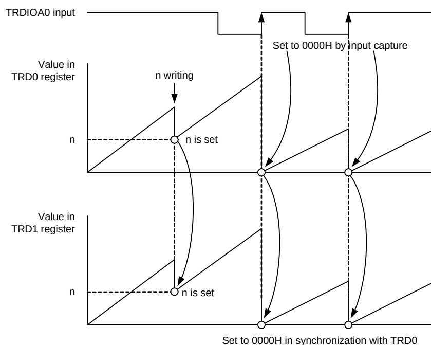
Figure 8-43. Synchronous Operation
