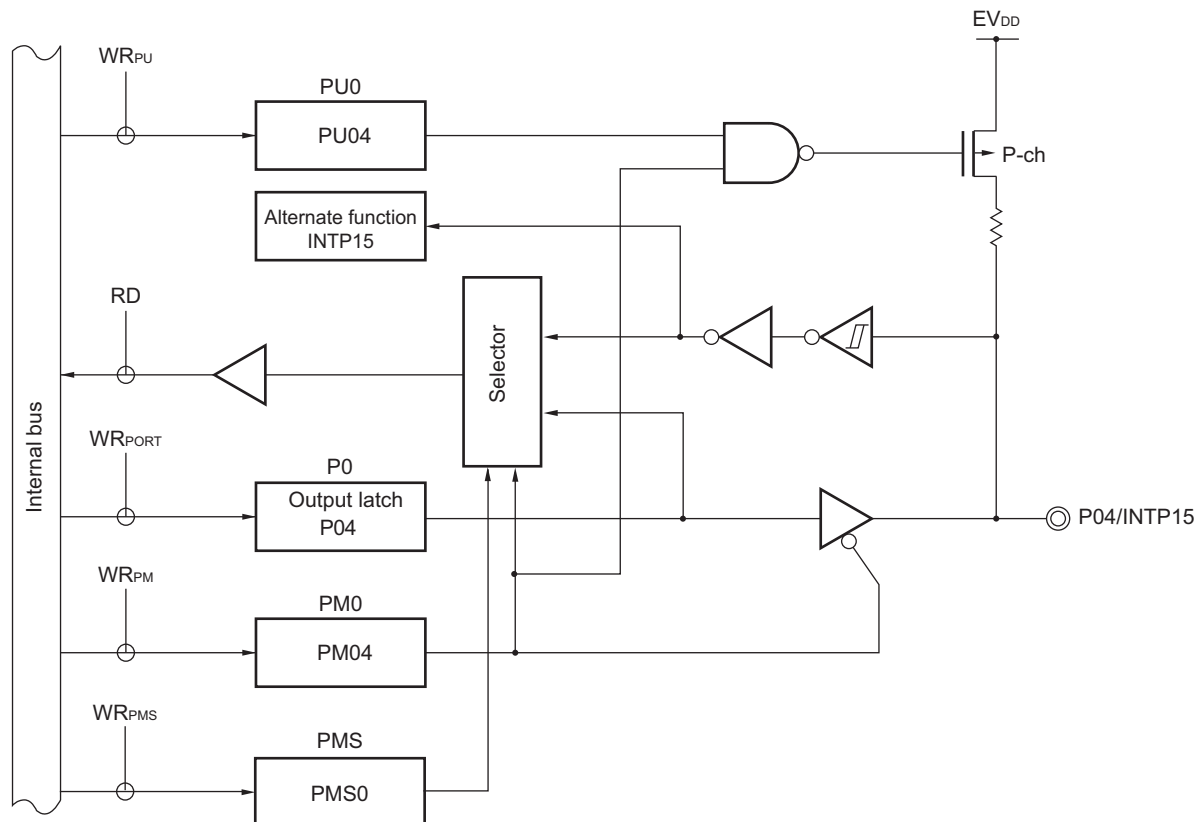
Figure 4-5. Block Diagram of P04
