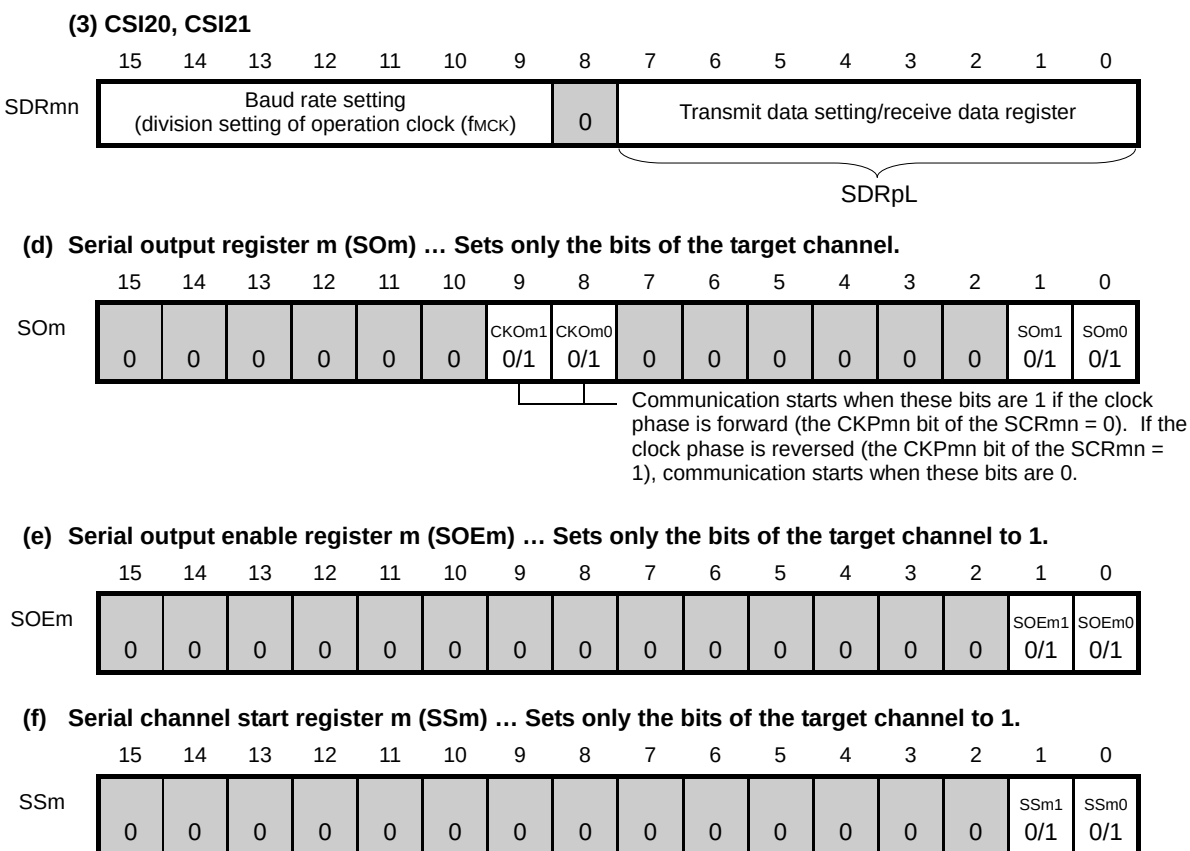
Figure 15-54. Example of Contents of Registers for Master Transmission/Reception of 3-Wire Serial I/O (CSI00, CSI01, CSI10, CSI11, CSI20, CSI21) (2/2)
