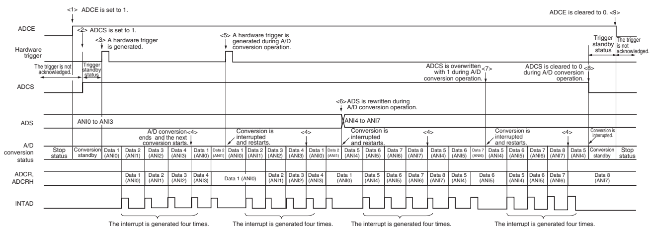
Figure 12-26. Example of Hardware Trigger No-Wait Mode (Scan Mode, Sequential Conversion Mode) Operation
