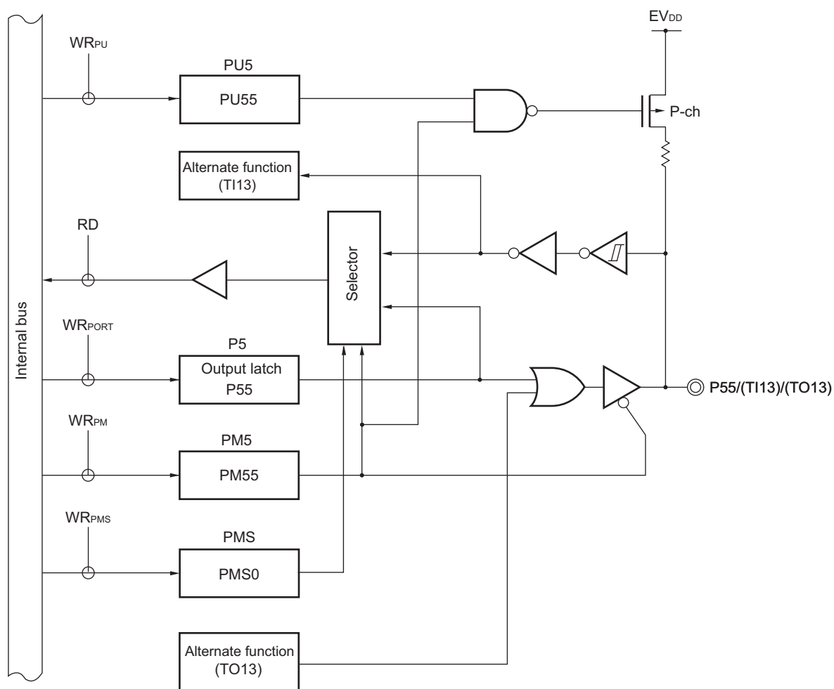
Figure 4-42. Block Diagram of P55
