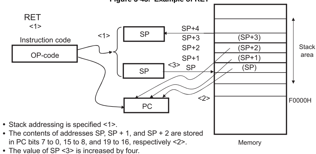
Figure 3-43. Example of RET
