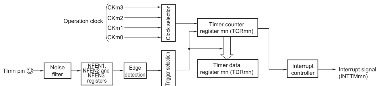
Figure 6-61 Block Diagram of Operation as Input Signal High-/Low-Level Width Measurement
