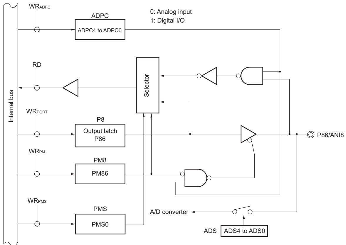
Figure 4-67. Block Diagram of P86
