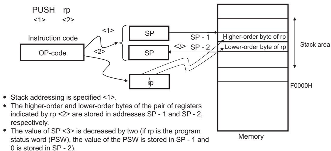
Figure 3-40. Example of PUSH rp
