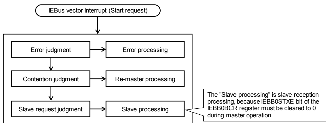
Figure 19-37. IEBus vector interrupt (Start request) processing flow example (Master reception)
