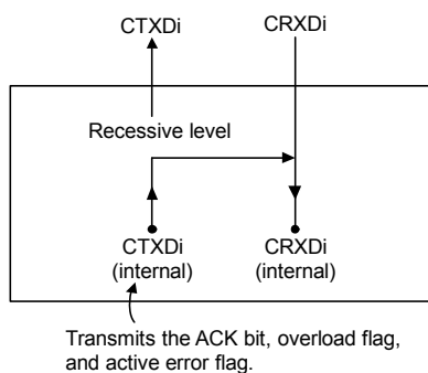
Figure 18-10. Connection when Listen-Only Mode is Selected
