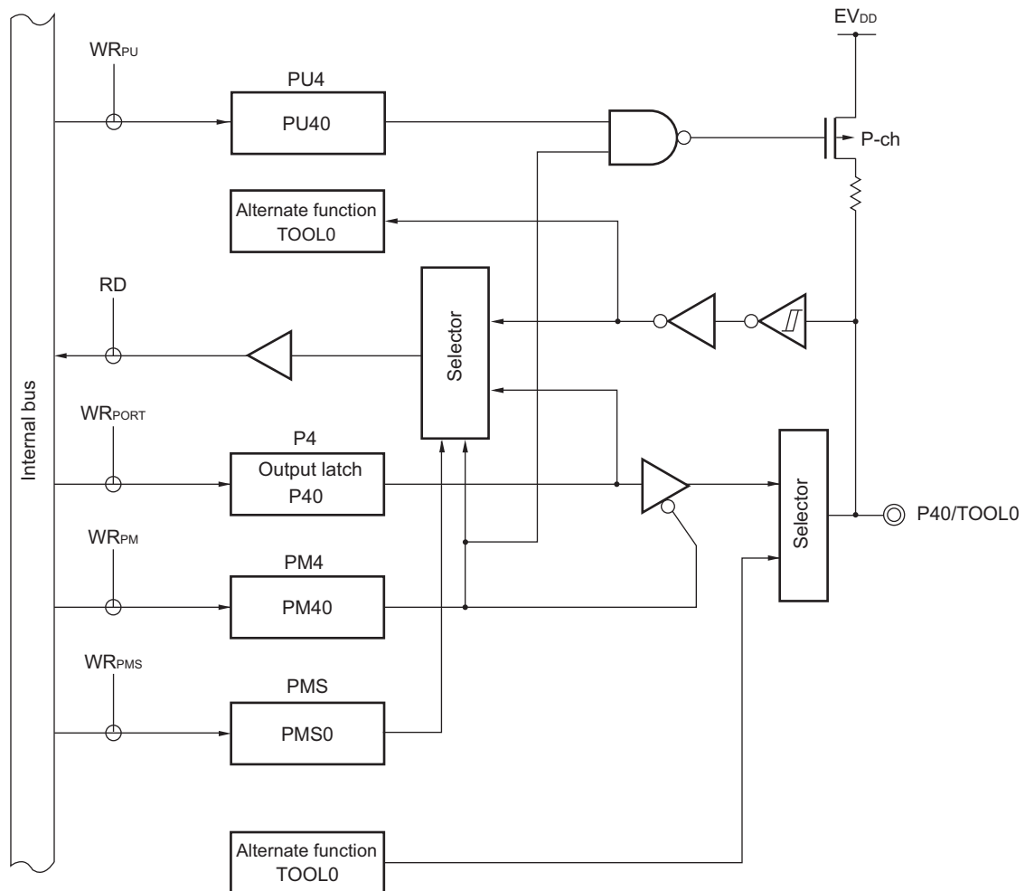
Figure 4-29. Block Diagram of P40
