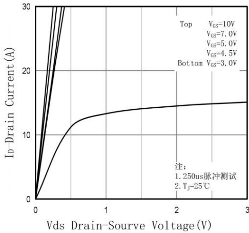
Fig.1 Output Characteristic
