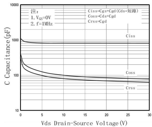
Fig.6 Capacitance Characteristic
