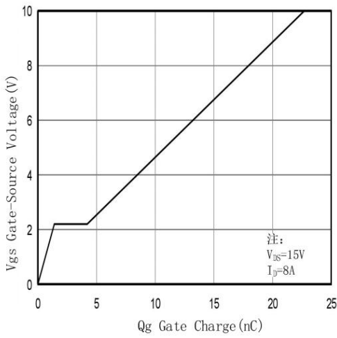
Fig.7 Gate-Charge Characteristic
