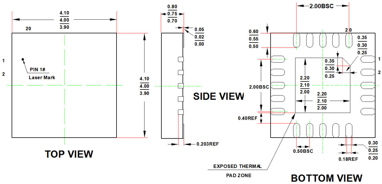
Figure 48. 20-Lead QFN Package Dimensions Shown in Millimeter
