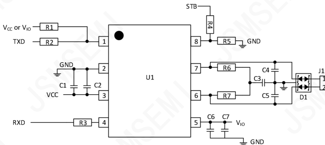
Figure 10-1. Layout Example
