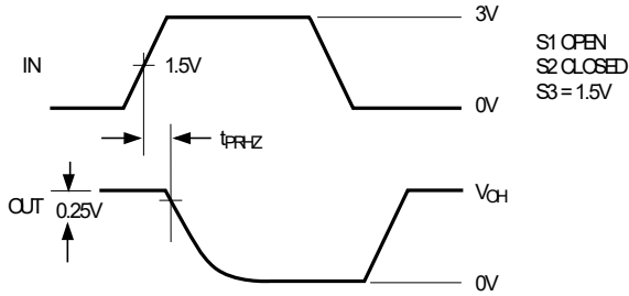
Figure 8. Receiver Enable and Disable Times
