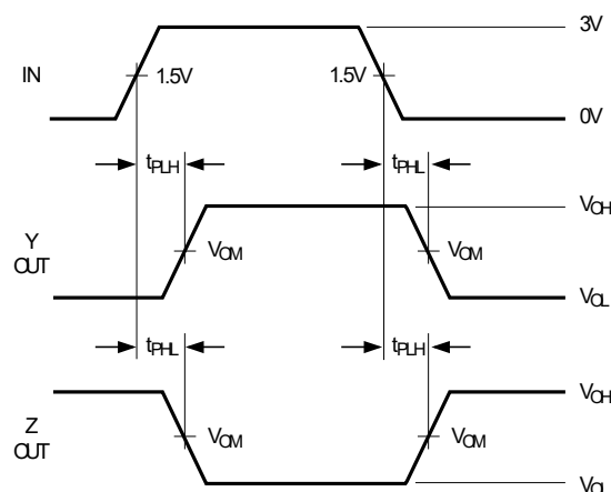
Figure 4. Driver Propagation Times
