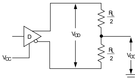
Figure 2. Driver DC test load
