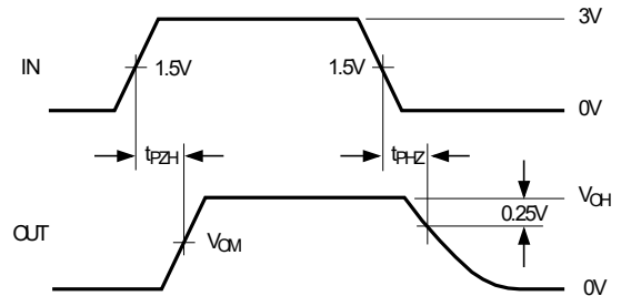
Figure 5. Driver enable and disable times
