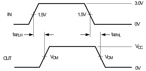
Figure 7. Receiver Propagation Delay
