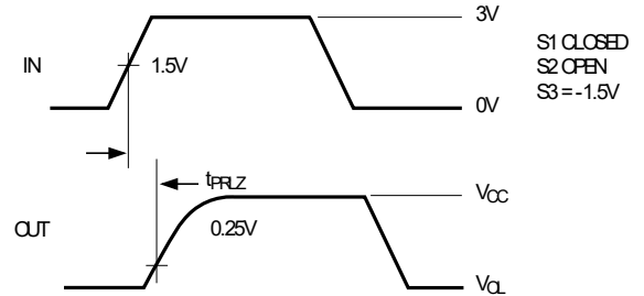
Figure 8. Receiver Enable and Disable Times
