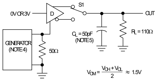
Figure 5. Driver enable and disable times
