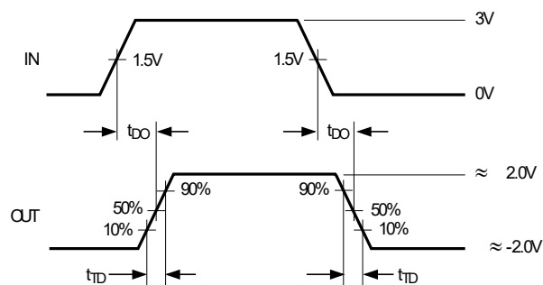
Figure 3. Driver Differential Output Delay and Transition Times
