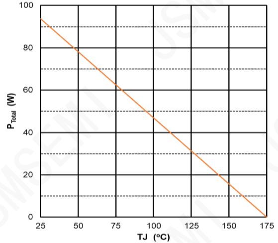
Figure 4. Power Derating
