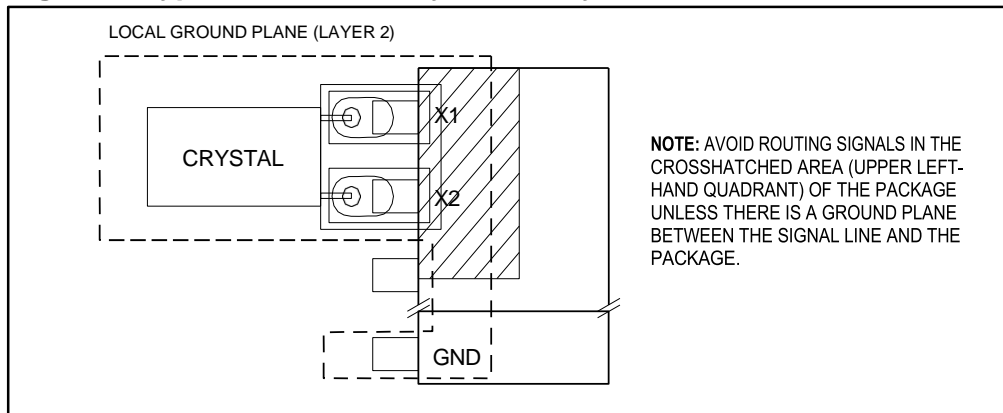
Figure 2. Typical PC Board Layout for Crystal
