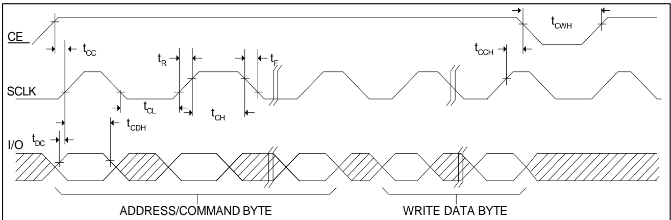
Figure 7. Timing Diagram: Write Data Transfer
