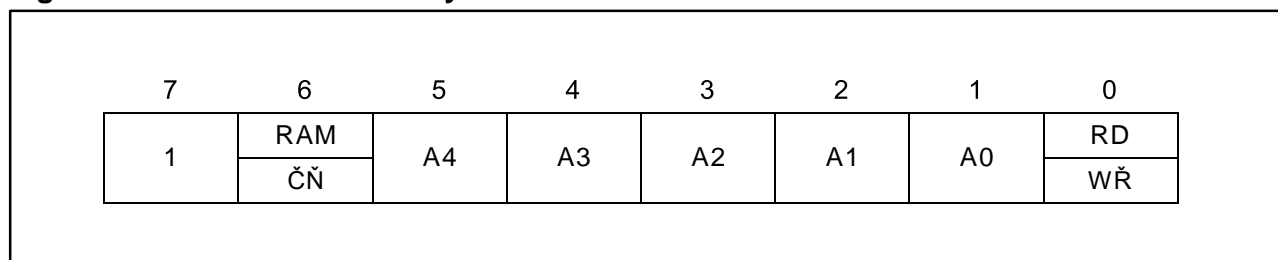
Figure 3. Address/Command Byte
