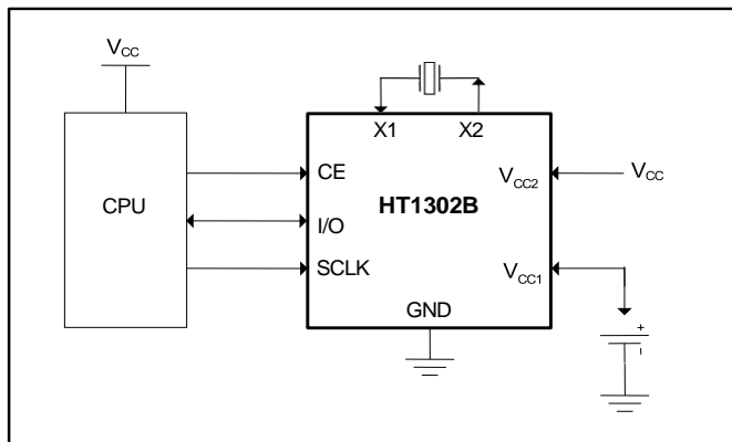
Figure 1 shows the main elements of the serial timekeeper: shift register, control logic, oscillator, real-time clock, and RAM.
