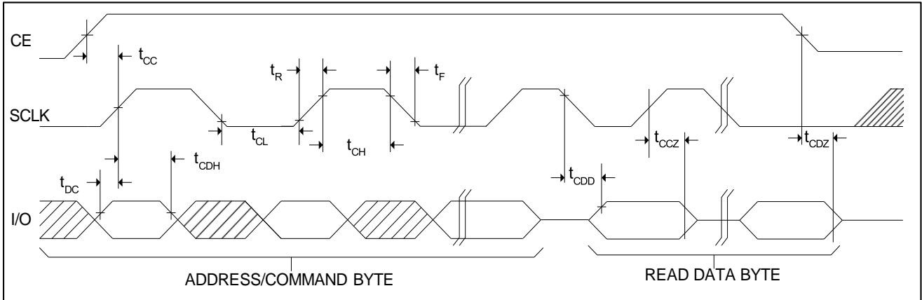
Figure 6. Timing Diagram: Read Data Transfer
