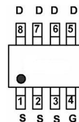
pin assignment
