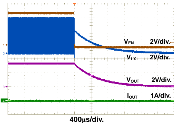
Figure 14. Power Off through EN Waveform
