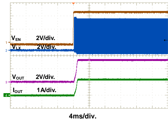
Figure 13. Power On through EN Waveform
