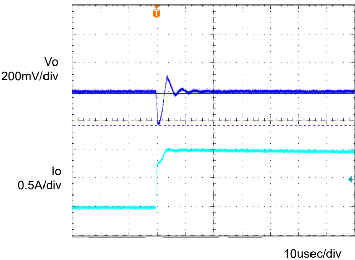
Fig.3 Transient Response (0 \rightarrow 1.0A) Co=1 \mu F, Ta=-40°C
