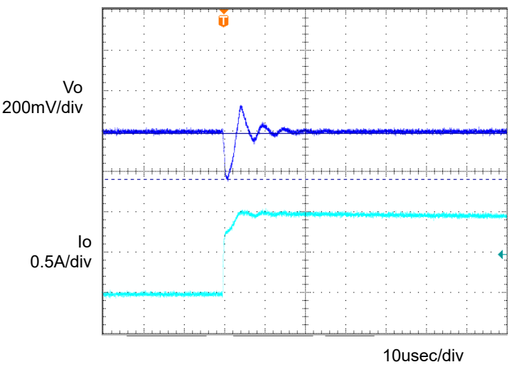
Fig.4 Transient Response (1.0 \rightarrow 0A) Co=1 \mu F, Ta=25°C
