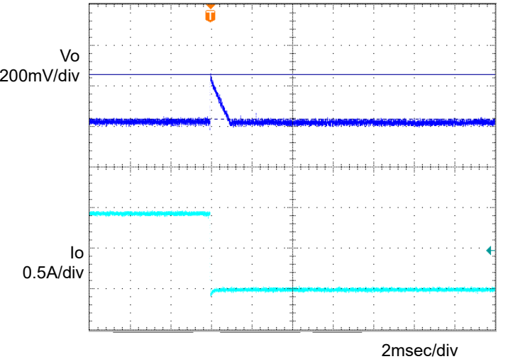
Fig.6 Transient Response (1.0 \rightarrow 0A) Co=1 \mu F, Ta=-40°C
