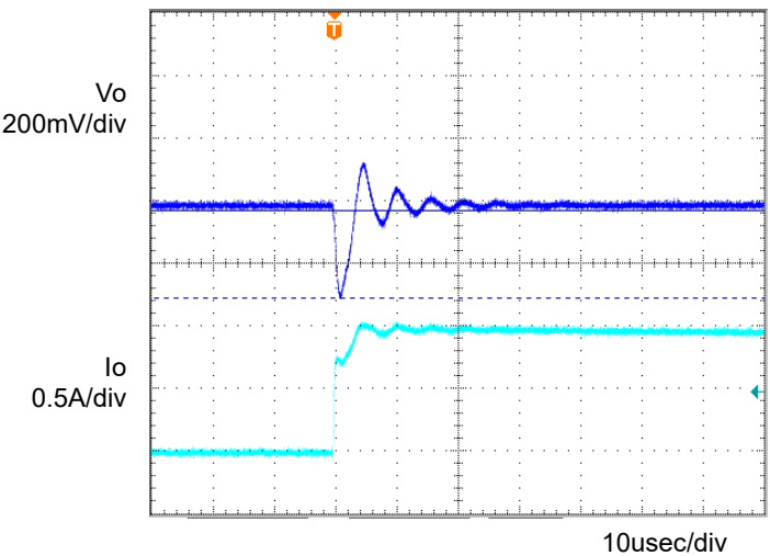
Fig.5 Transient Response (0 \rightarrow 1.0A) Co=1 \mu F, Ta=105°C
