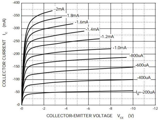
Static Characteristic
