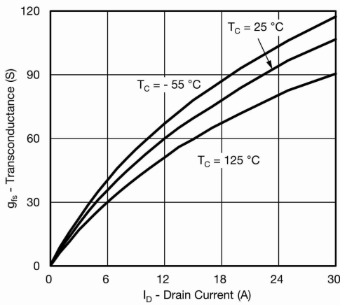
Transconductance
