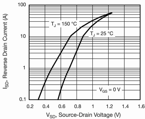
Fig. 8 - Typical Source-Drain Diode Forward Voltage
