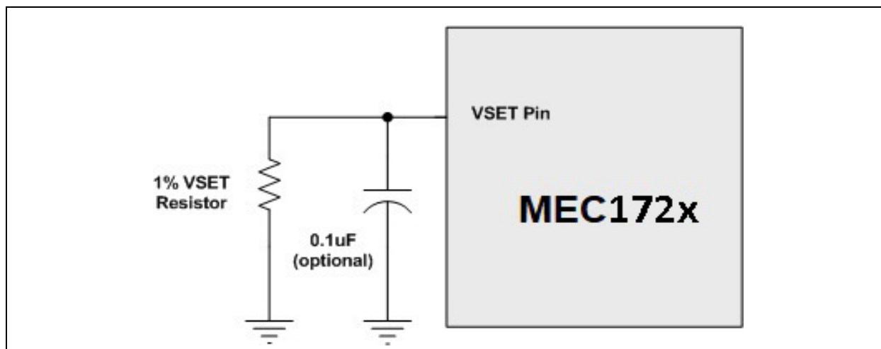
FIGURE 2-9: VSET CIRCUIT
