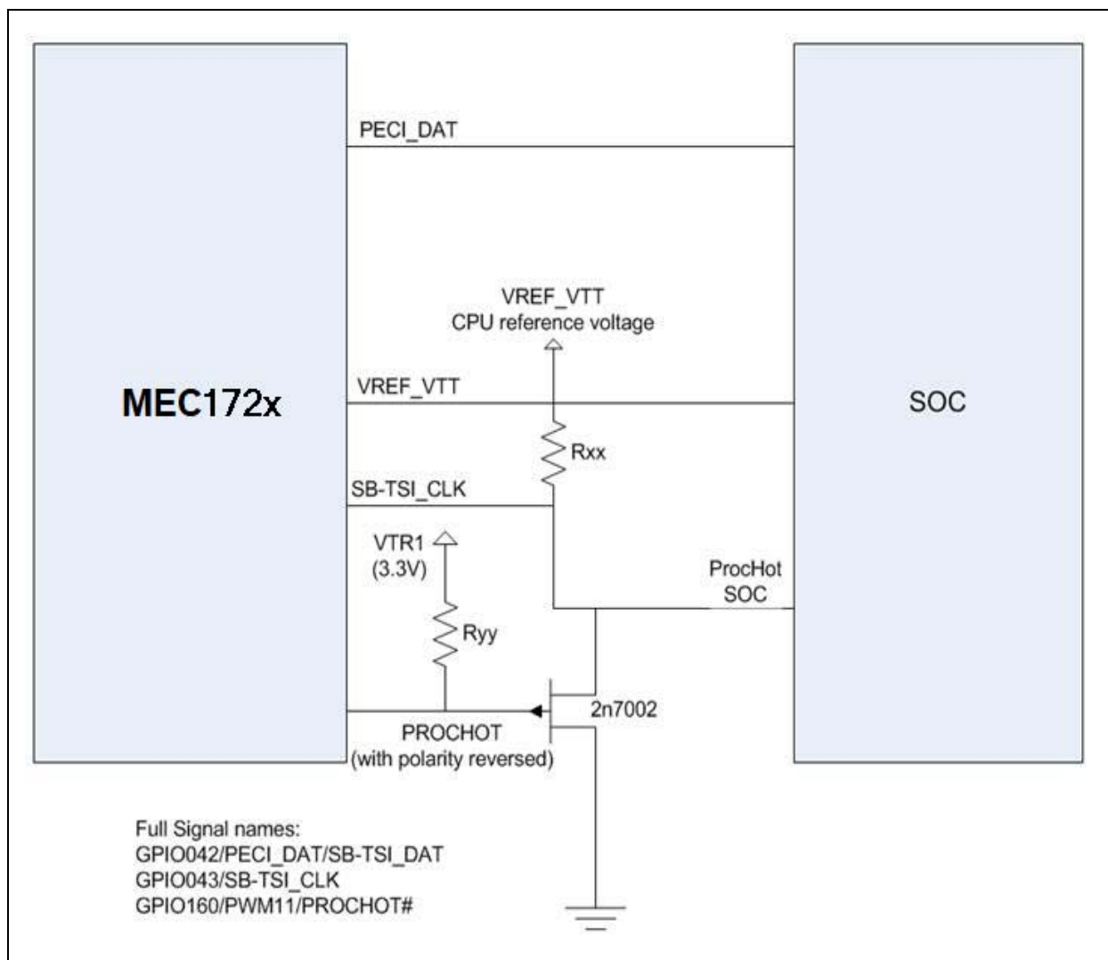
FIGURE 2-11: PROCHOT IMPLEMENTATION
