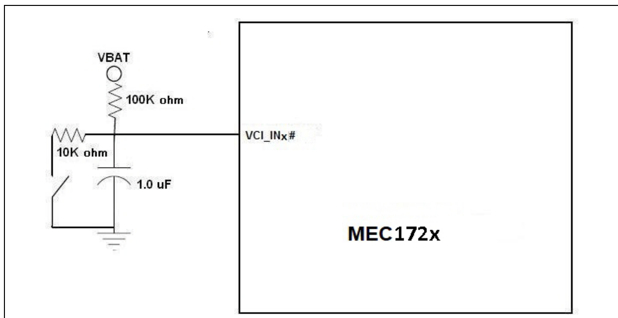
FIGURE 2-8: VBAT-POWERED CONTROL INPUT CIRCUIT
