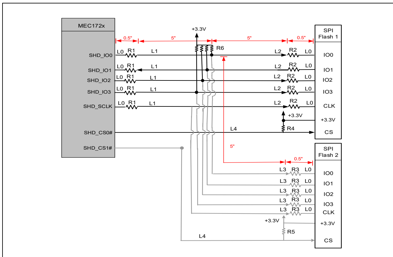
FIGURE 2-7: MEC1721/MEC1723 TOPOLOGY FOR NON-SHARED DUAL SPI FLASH DEVICE
