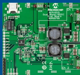
MCP19215 Dual Boost/SEPIC Evaluation Board
