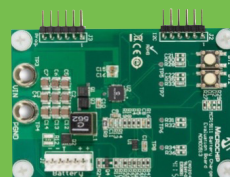
MCP19111 Battery Charger Evaluation Board
