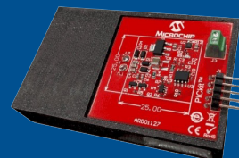
Qi Wireless Power Micro-Receiver Reference Design
