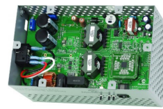
Digital Power Interleaved PFC Reference Design
