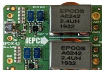
EPC9143 300W 1/16 Brick Power Module Reference Design
