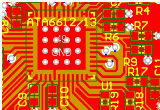
Figure 3. PCB Layout Example for Atmel® ATA6612/ATA6613 Central Pad
