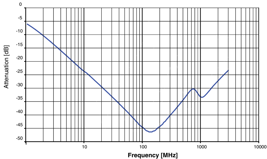
Figure 1-3. Attenuation of 2 Ceramic Capacitors of 10nF and 100pF in Parallel in a 50Ω System
