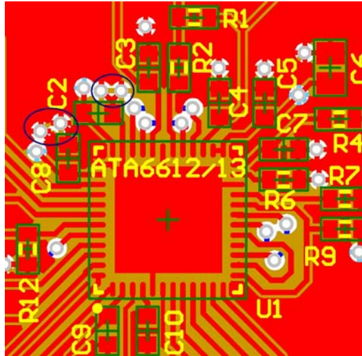
Figure 1. PCB Layout Example for VCC Decoupling
