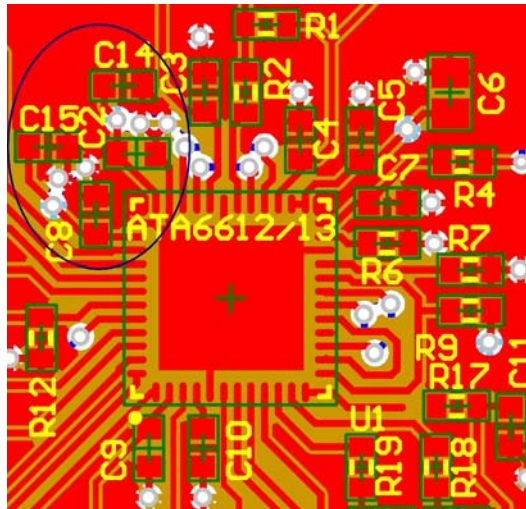
Figure 2. PCB Layout Example for Improved VCC Decoupling
