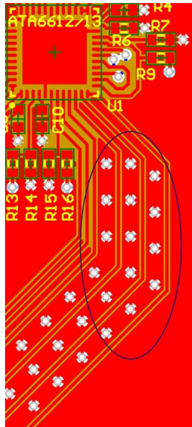
Figure 6. PCB Layout Example for Improved Signal Track Decoupling
