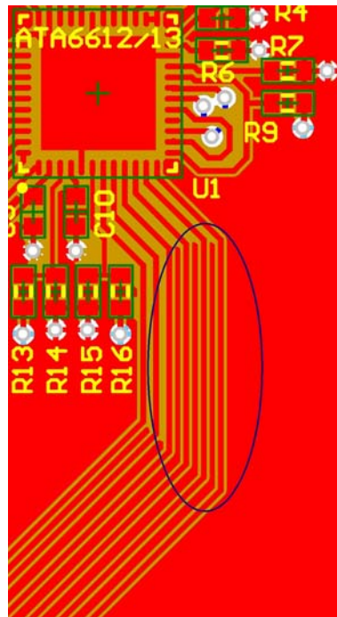
Figure 5. PCB Layout Example for Signal Track Decoupling
