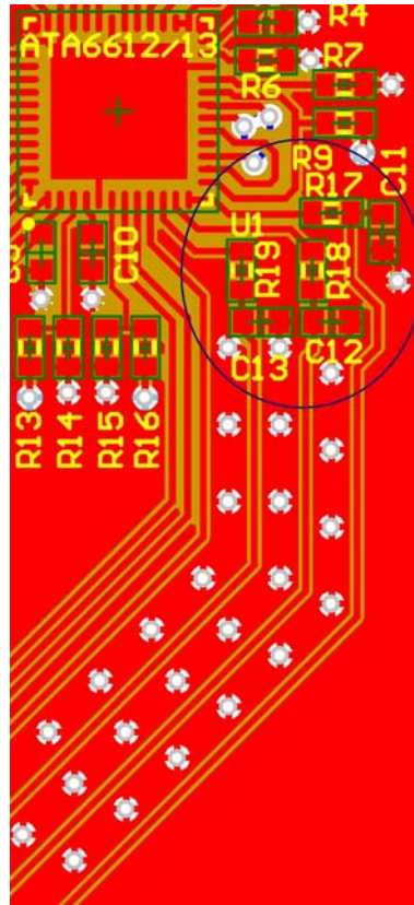
Figure 4. PCB Layout Example for RC Filters in Switched Signal Lines
