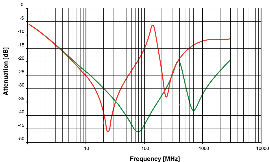
Figure 1-4. Attenuation of 2 Ceramic Capacitors of 10nF and 100pF in Parallel in a 50Ω System with Realistic Parasitic Components in Connecting Tracks
