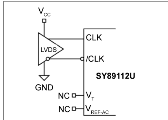
FIGURE 5-5: LVDS Interface.
