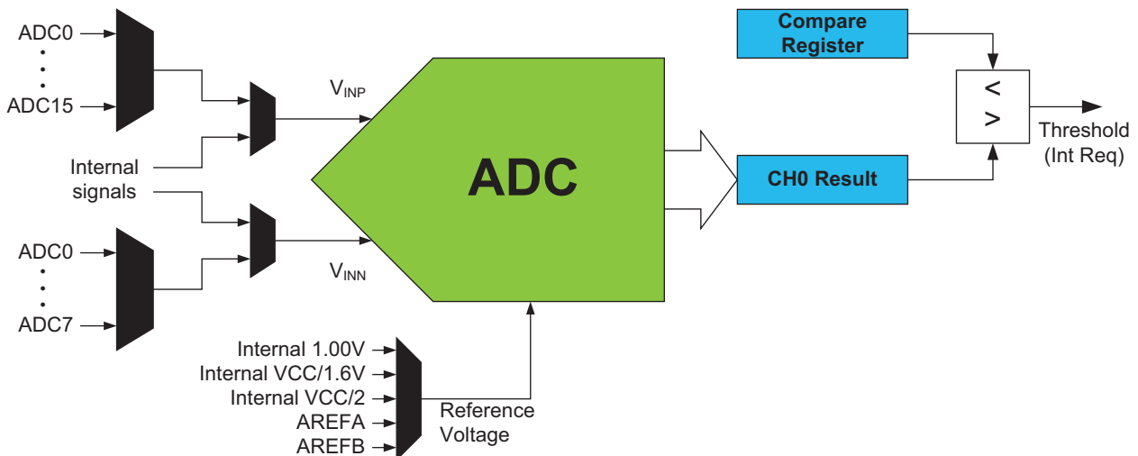
Figure 3-1. ADC Overview
