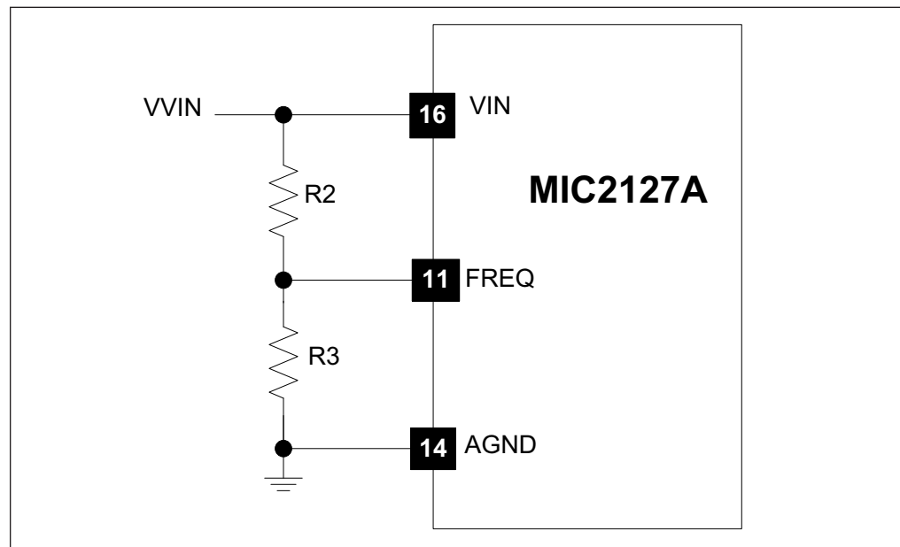
FIGURE 2-2: Switching Frequency Adjustment.
