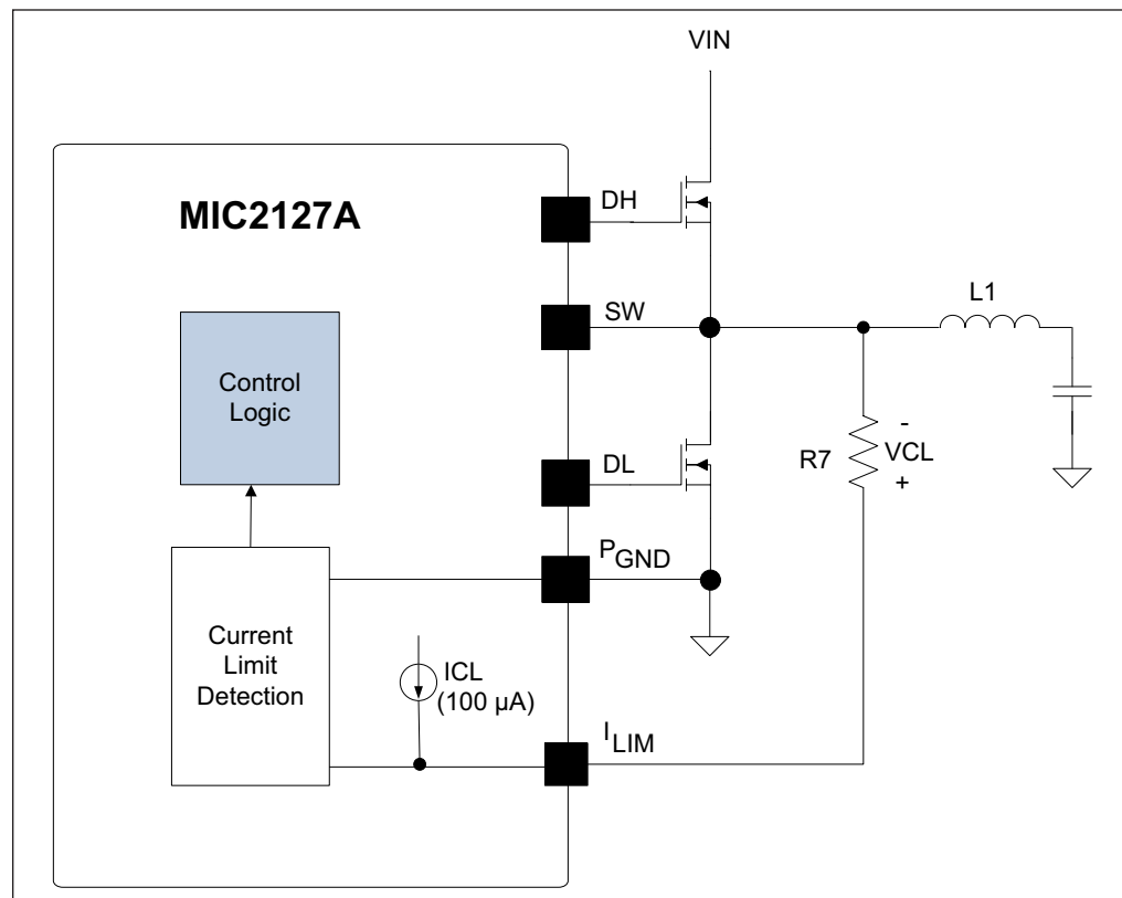
FIGURE 2-1: Switching Frequency Adjustment.
