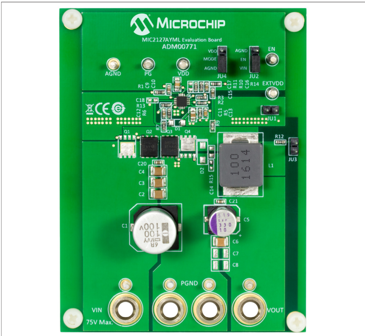
FIGURE 1-1: MIC2127A Evaluation Board Overview.
