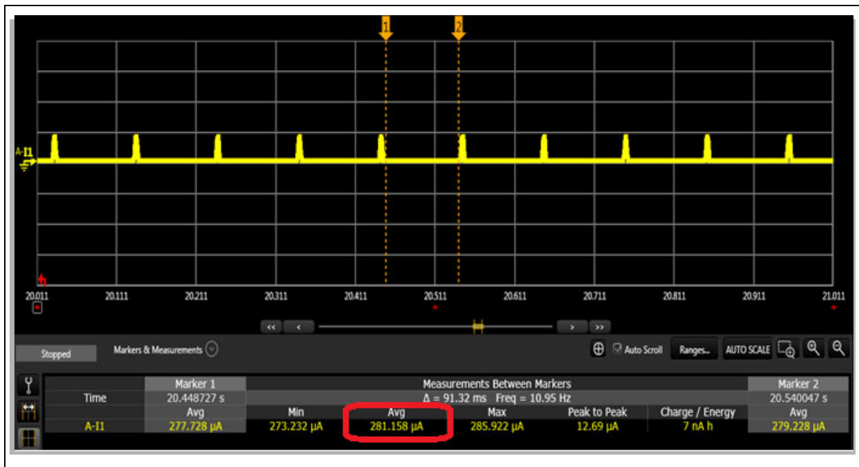
FIGURE 4: WINC1500 AUTO DEEP SLEEP CURRENT
