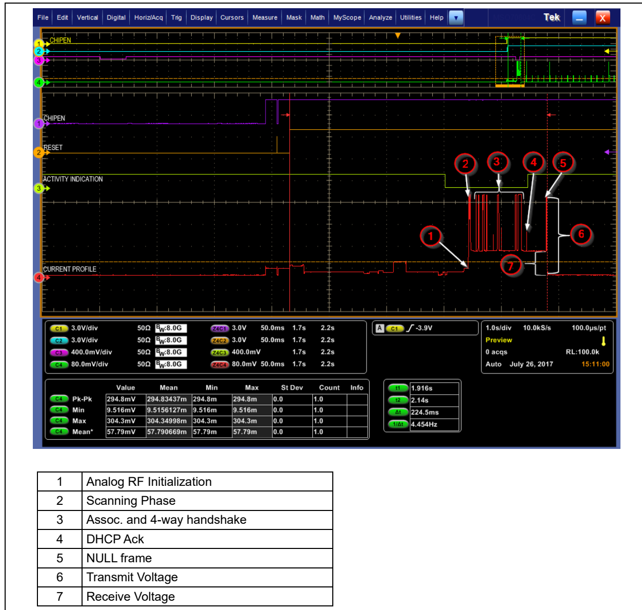
FIGURE 13: ZOOMED IN CAPTURE OF WINC1500 CONNECTION TO AP
