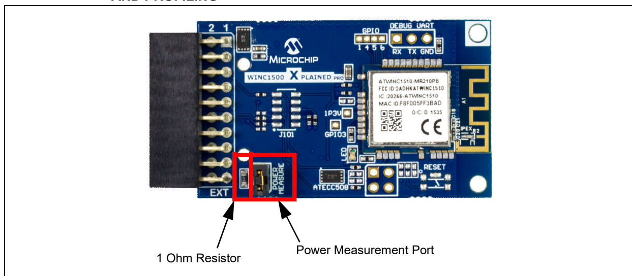
FIGURE 2: WINC1500 POWER MEASUREMENT PORT USED FOR CURRENT MEASUREMENT AND PROFILING
