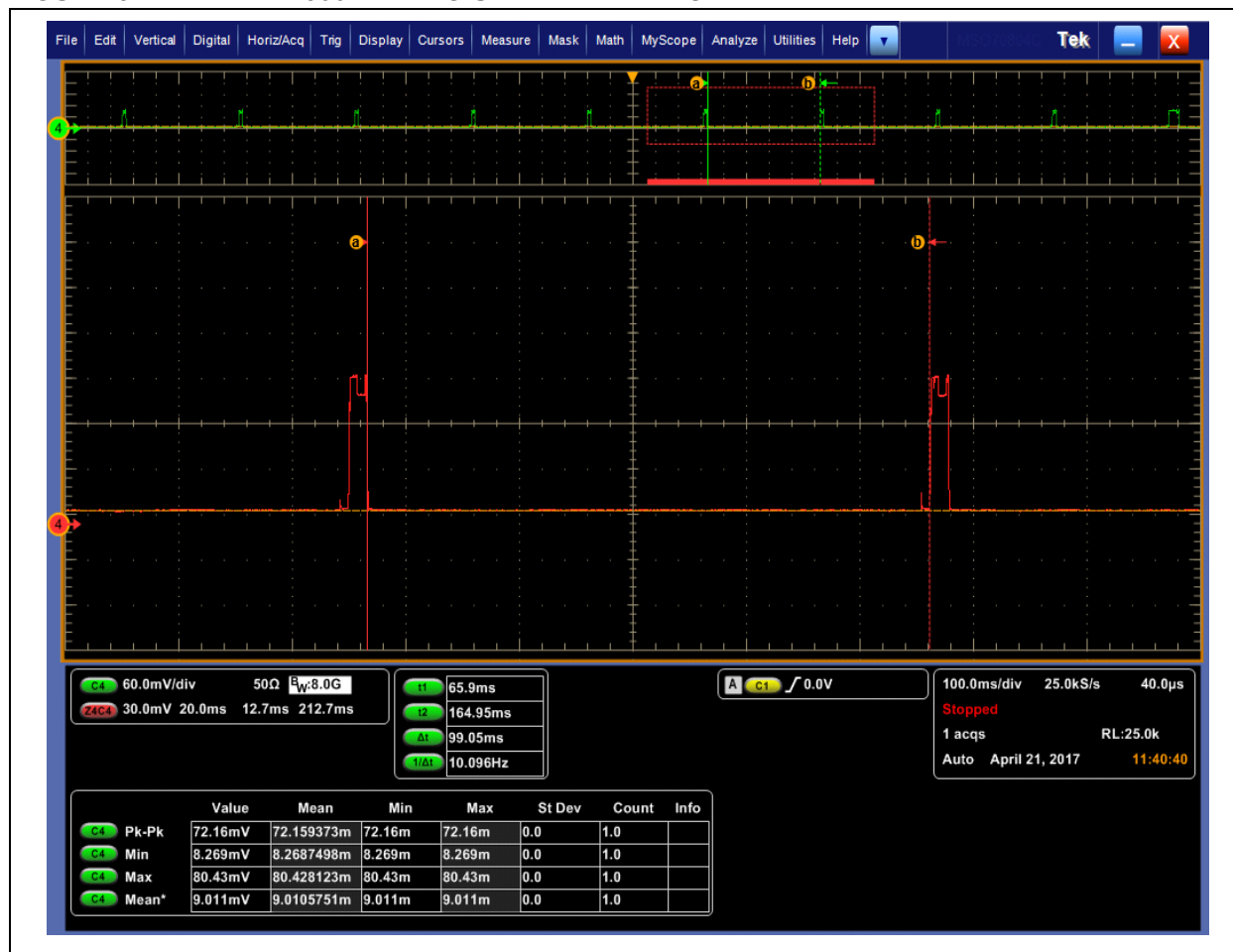
FIGURE 5: WINC1500 WAKING UP EVERY BEACON INTERVAL
