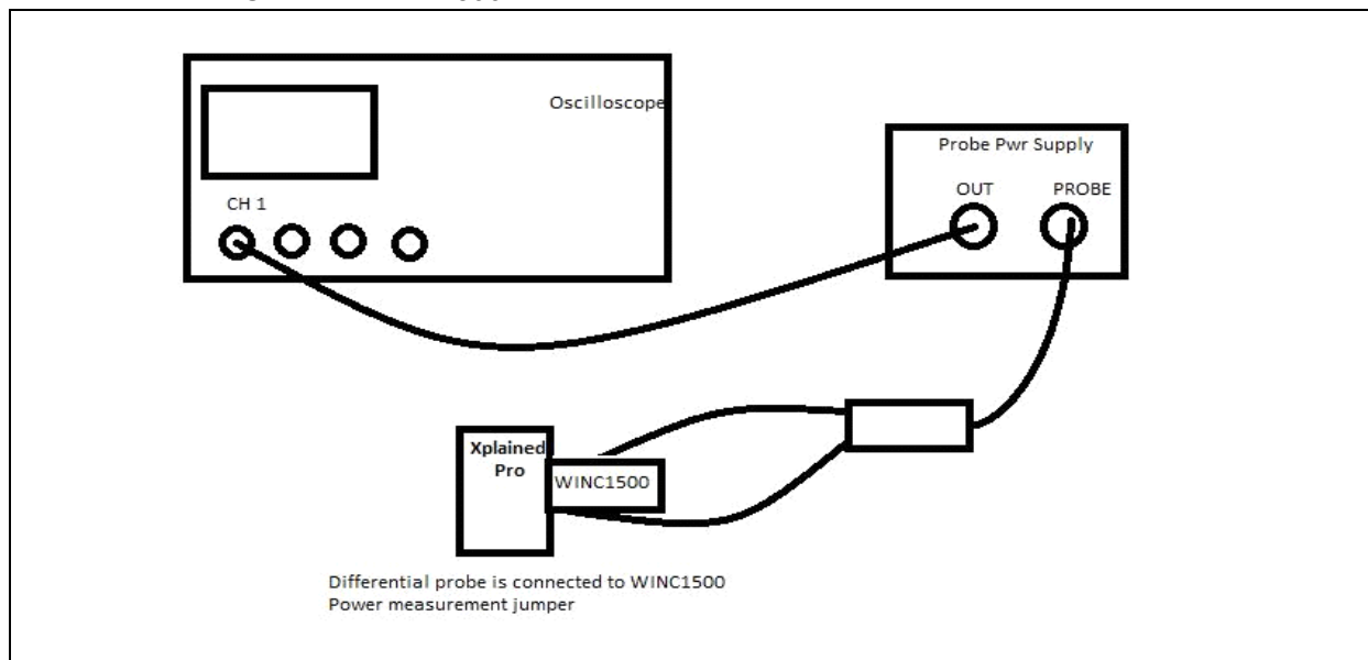
FIGURE 1: EXAMPLE DIFFERENTIAL PROBE SETUP TO MEASURE VARIOUS PARAMETERS ON THE WINC1500
