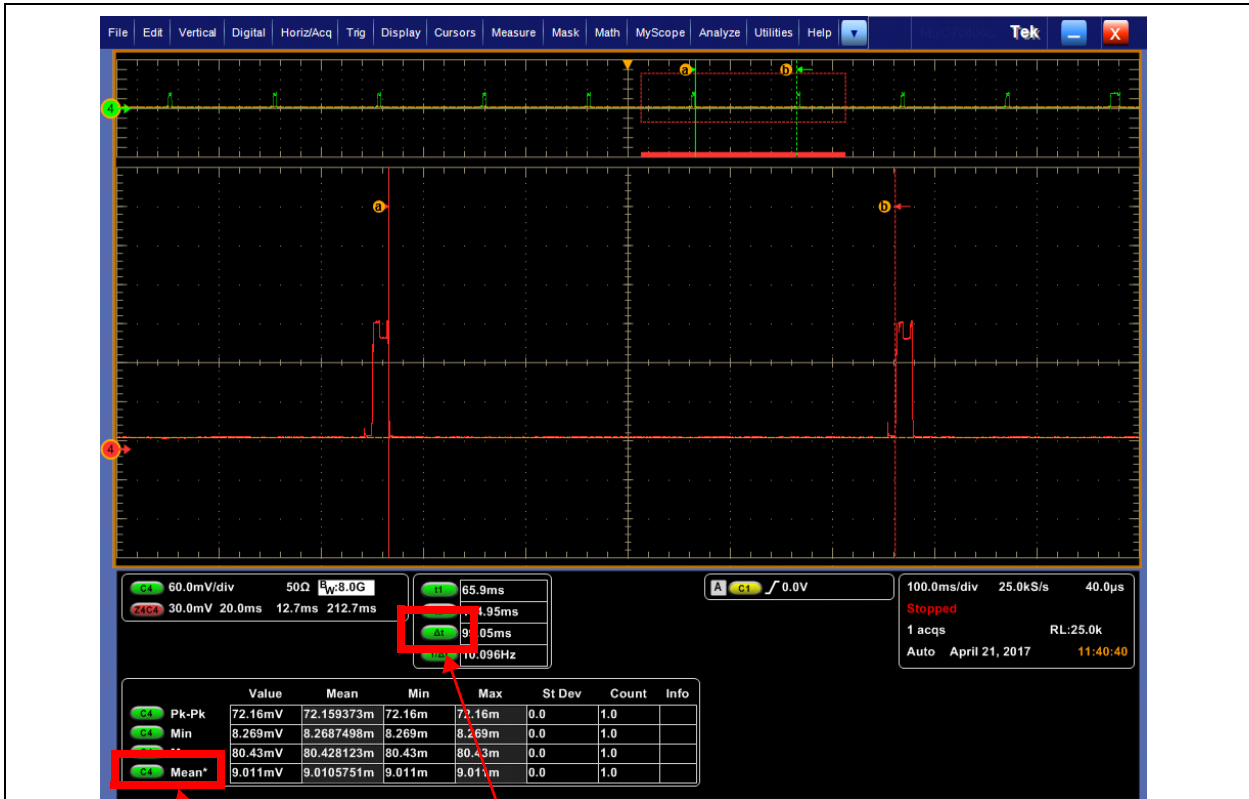
FIGURE 3: HOW TO INTERPRET THE MEASUREMENTS
