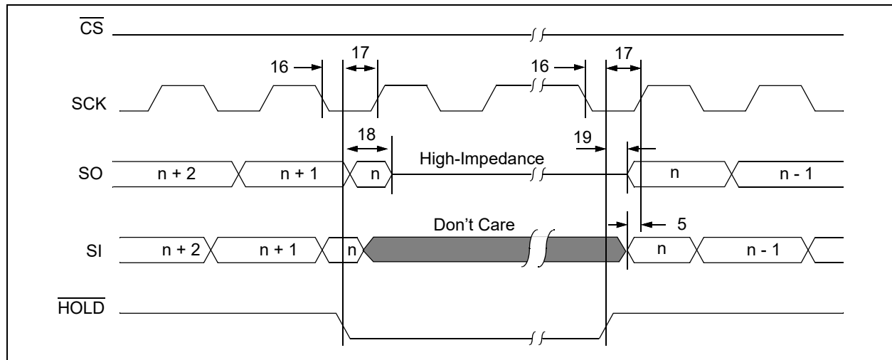
FIGURE 1-1: HOLD TIMING
