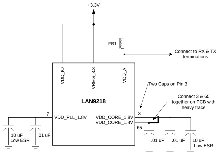
Figure 3 - LAN9218 Power Connections
