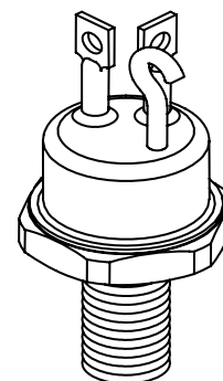
TO-59
