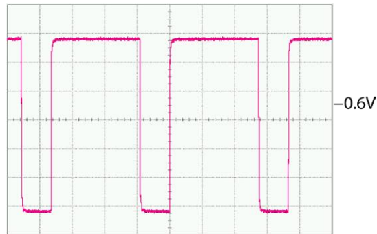
10 ns/DIV, 200mV/DIV
