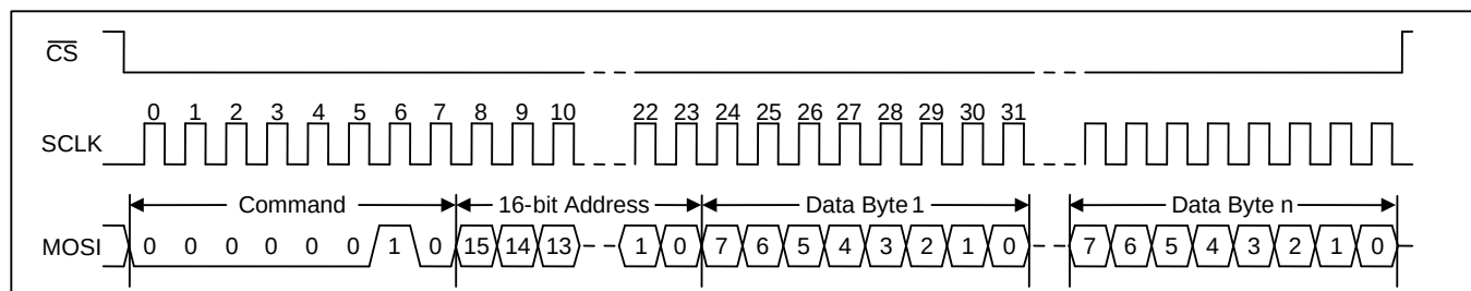
Figure 7 - SPI Write Transaction Functional Timing
