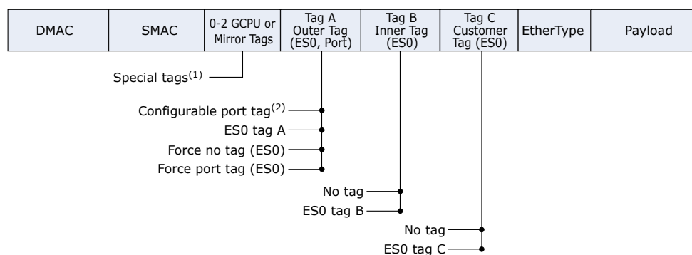
Figure 4-92. VLAN Pushing
