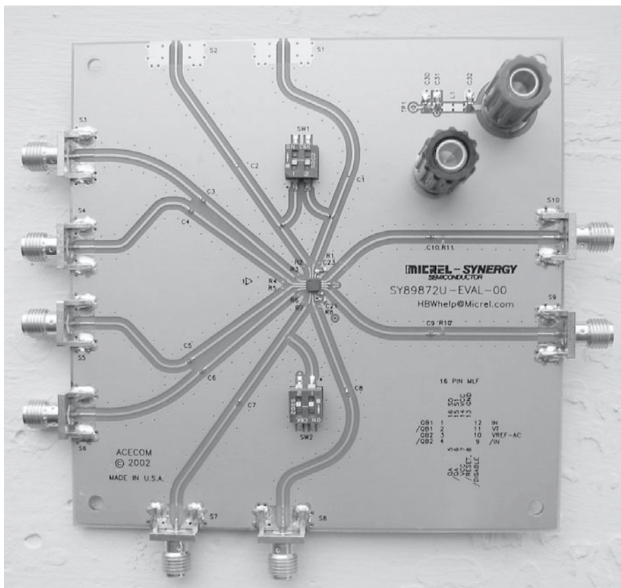
Figure 1. SY89872U Evaluation Board
