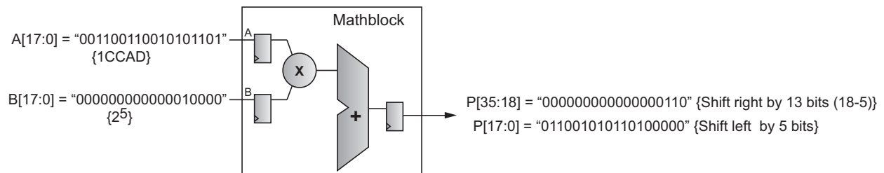
Figure 16 • Logical Shift Left/Right using Mathblock
