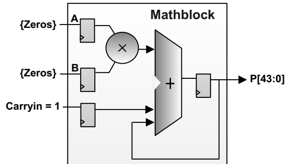
Figure 27 • Binary Counter using Mathblock
