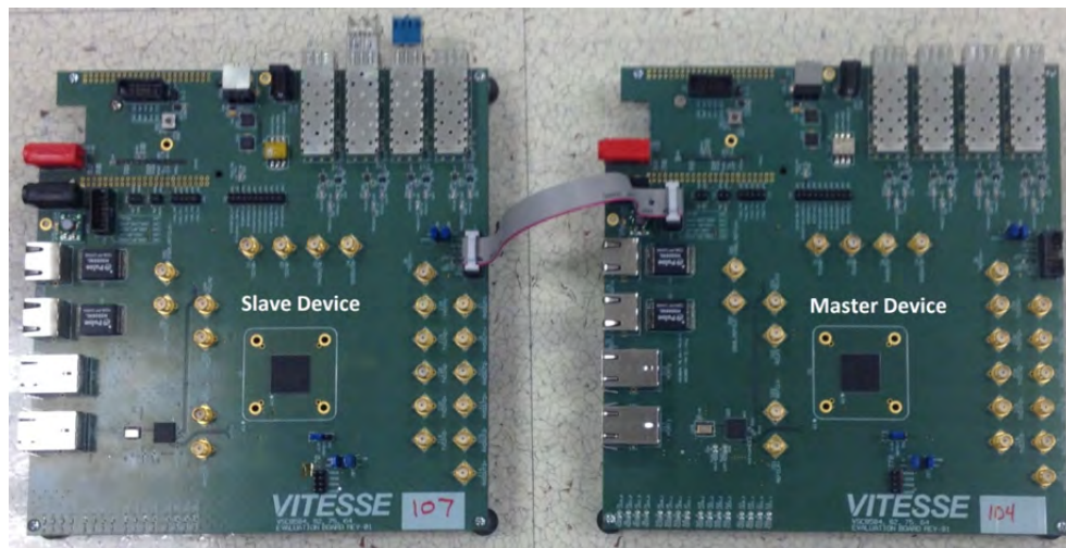
Figure 3 • 1588 Daisy-Chain SPI Interconnect
